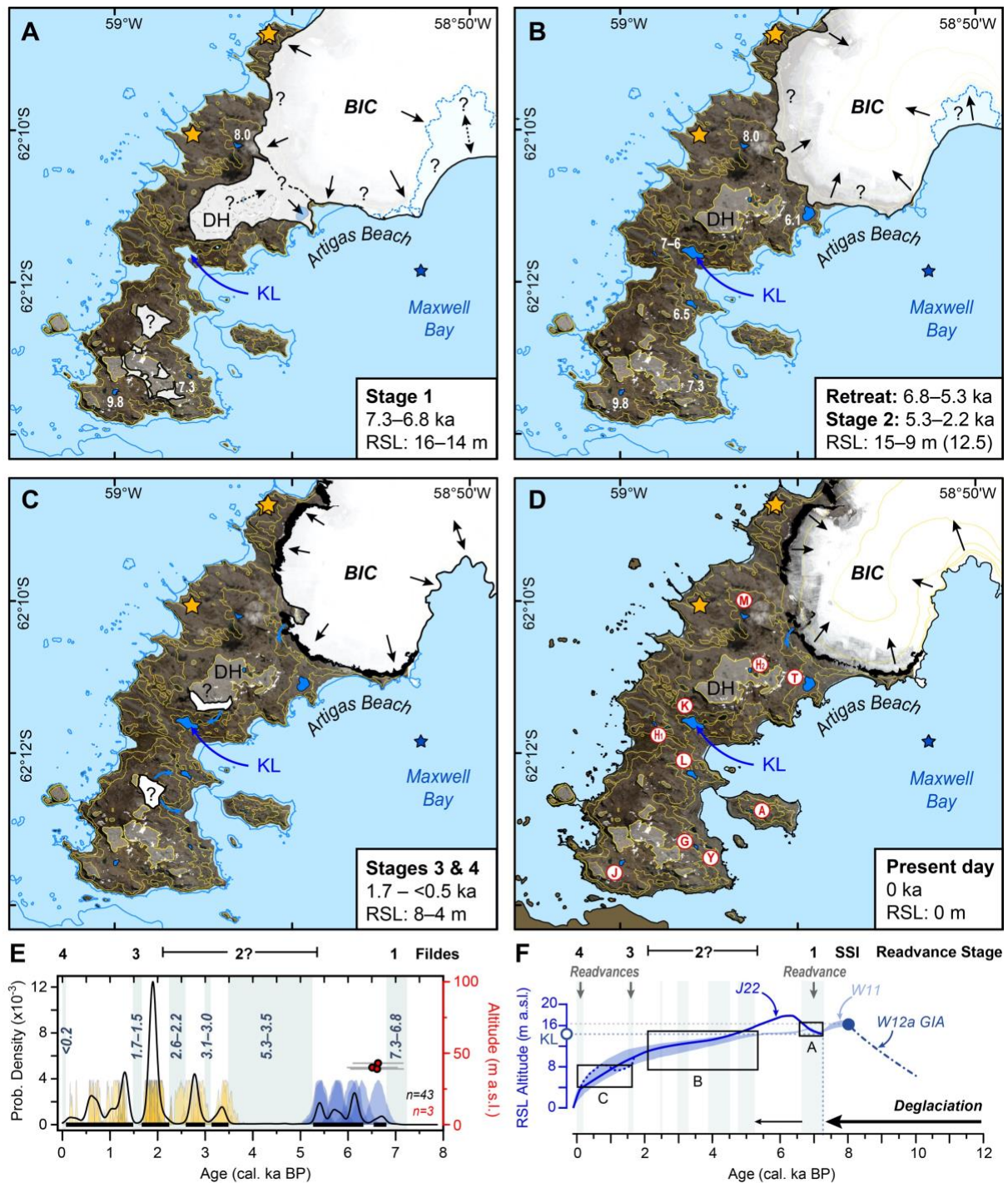
Figure 6. A–D) Schematic reconstruction of Mid- to Late Holocene glacier readvance extents during Stages 1–4 on the Fildes Peninsula. Glacier extents shown in A–C are based on a compilation of new and published chronological data (panel E) for the Shetland I moraine (dark shading in C and D). E) Radiocarbon ages and probability density phase model for age constraints on glacier readvance on the Fildes Peninsula (n=43; Figure 3C for details; yellow distributions are radiocarbon ages of terrestrial material embedded in moraines; blue distributions are radiocarbon ages of marine material embedded in moraines; red circles with
