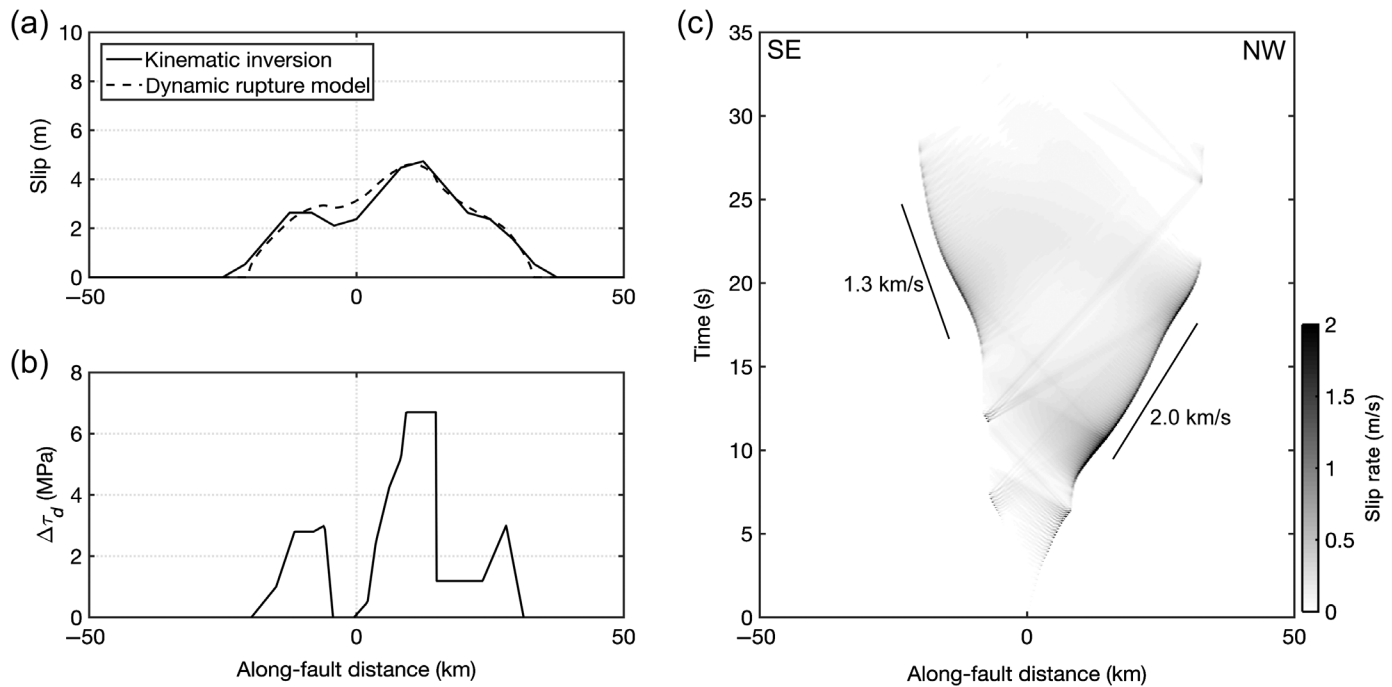
Figure 5. (a) Along-fault slip distribution resolved by the kinematic slip inversion (solid line) and that calculated from the dynamic rupture model (dashed line). The x-axis measures distance from where the earthquake is nucleated in our model. (b) Dynamic stress drop along the fault. Location shown in Figure 4. (c) Spatiotemporal and bilateral rupture history predicted by the dynamic rupture model. Solid lines signify average rupture-front speed. Both rupture fronts propagate at sub-Rayleigh wavespeed.
