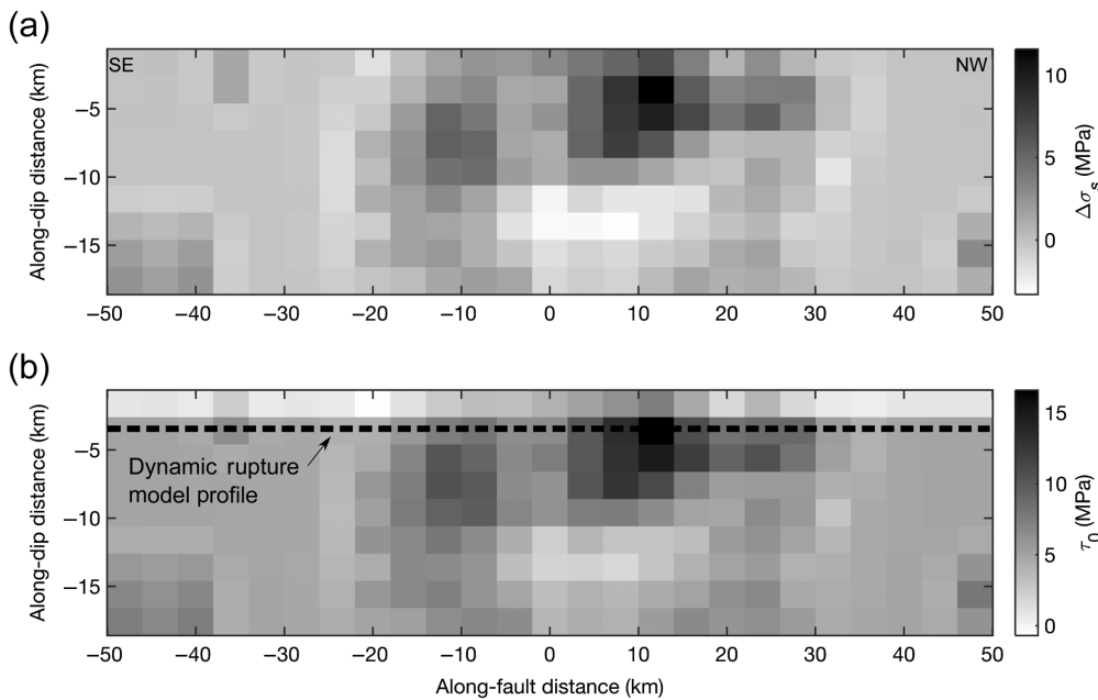
Figure 4. (a) Static stress drop and (b) initial shear stress along the mainshock fault plane. Static stress drop is calculated assuming a homogeneous Poisson medium and initial shear stress is computed using the complete stress-drop assumption. We select an initial shear stress profile through the main asperity at 3 km depth (dashed line) for our 2D dynamic rupture models.
