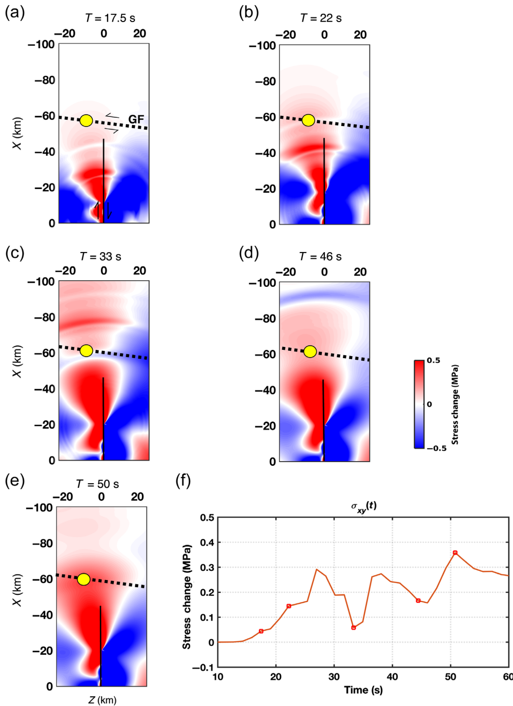
Figure 8. Similar to Figure 9, but shear stress changes ( \sigma_{xy} ) during coseismic rupture. (a–e) \sigma_{xy} from 17.5 to 50 s during rupture propagation. (f) The time history of \sigma_{xy} showing three distinct peaks in stress change on the Garlock fault at \sim 28 , 38, and 50 s. The color version of this figure is available only in the electronic edition.
