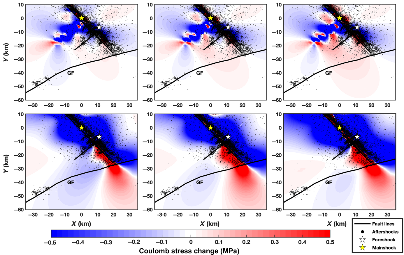
Figure 3. \Delta CFS of the mainshock on a receiver fault of 70° strike and 90° dip, approximating the leftmost part of the Garlock fault in this figure. (Top) \Delta CFS results for a 5 km depth source at friction coefficients of (left to right) 0.2, 0.4, and 0.6. (Bottom) \Delta CFS results for a 10 km depth source with the same friction coefficients. The color version of this figure is available only in the electronic edition.
