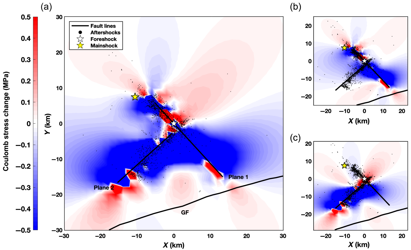
Figure 2. Coulomb stress change ( \Delta CFS ) due to foreshock planes 1 and 2 on the mainshock fault plane calculated at a depth of 5 km and with a friction coefficient of 0.6. (a) The combined effect of both aftershock fault plane slip on the mainshock. (b) The \Delta CFS from plane 1, which is parallel to the main fault plane. (c) \Delta CFS from plane 2, which is the northeast–southwest-striking cross fault. The aftershocks depicted are the earthquakes that occurred after the foreshock and do not include those induced from mainshock stress changes. GF, Garlock fault. The color version of this figure is available only in the electronic edition.
