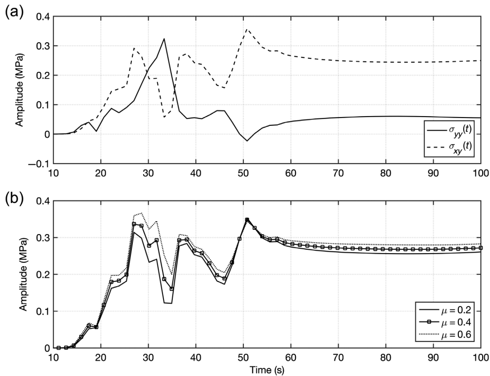
Figure 9. Stress-change evolution on a section of the Garlock fault during the entire Ridgecrest earthquake simulation. (a) Normal ( \sigma_{yy} ) and shear ( \sigma_{xy} ) stress change. (b) Temporal \Delta CFS for friction coefficient levels assessed in the static stress-change analysis. Note that we plot the temporal stress change starting at 10 s because this is when the nucleation procedure ceases.
