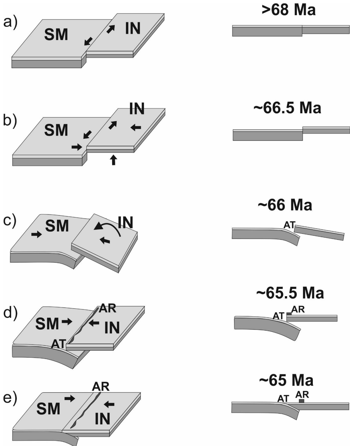
Figure. 15 Model showing the evolution of India-Somalia (Arabia) boundary at the Deccan event, along the western margin of India below the Baluchistan subduction zone. a) The boundary between Indian and Arabian plates is essentially a sinistral transform fault, with the Somali (Arabia) block moving downwards and the Indian plate moving
