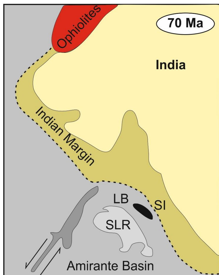
Figure. 3 The proposed point of Subduction initiation in the Laxmi Basin along the continental margin of India. The region highlighted by the black enclosure marks the point where Pandey et al (2019) reported signatures of Boninite like and Fore Arc Basalt
