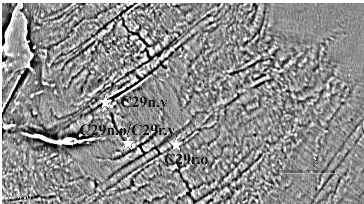
Figure. 5 Gravity map of the Central Indian Ridge after Vertical Gravity Gradient model of Sandwell et al (2014). The three white stars indicate changing positions of India at the onset and
