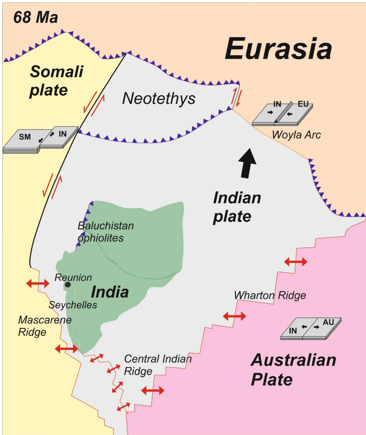
Figure. 10 The alignment of plate boundaries surrounding the Indian plate. At 68 Ma, the India -Somalia boundary is a left lateral strike slip fault in the north and a spreading centre in the south. The northern margin of the transform fault meets first the intraoceanic subduction between India and Eurasia, and further north ending in the subduction zone at the southern margin of Eurasia. The southern region ends in a triple
