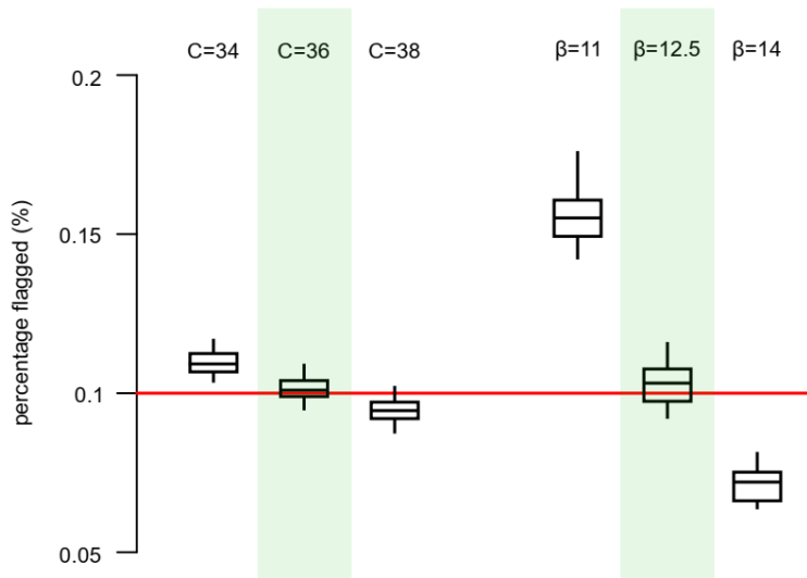
Fig. S1. Impact of the C values and \beta values on the percentage of outliers flagged in small samples ( n = 9 ) by respectively the Boxplot rule (using \alpha = A \log(n) + B + \frac{C}{n} with A and B known) and the MAD rule ( [l, u] = [\tilde{x} - \beta \text{MAD}, \tilde{x} + \beta \text{MAD}] with \tilde{x} the median). Each boxplot has been constructed on 100 generations of 10^5 random samples of size n = 9 from the Pearson family.
