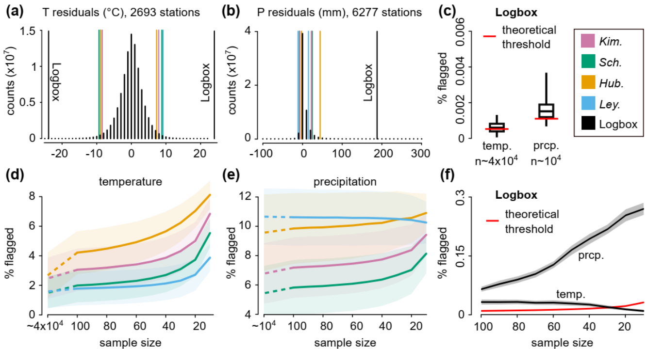
Fig. 2. Comparison between five outlier detection methods performed on two sets of residuals (temperature and precipitation) obtained from weather stations with daily measurements over at least 100 years. The two histograms (panels a and b ) represent aggregated residuals from all stations (for visualization purpose only) and show counts with at least 100 daily occurrences, with the median of the lower/upper threshold displayed for each method. For the methods Kim. (Kimber, 1990), Sch. (Schwertman et al., 2004), Hub. (Hubert & Vandervieren, 2008) and Ley. (Leys et al., 2013), the mean percentage ( \pm 1 SD) of flagged data is shown for sample sizes varying from 10 to 100, and for all available points per station ( n \sim 4 \times 10^4 for the temperature and n \sim 10^4 for the precipitation, panels d and e ). For Logbox (panels c and f ), this percentage is calculated by pooling all points, and the variability is estimated with a random resampling of stations (see method). The theoretical threshold is the expected percentage of erroneously flagged outliers ( p_{theo} = f(n) \times \frac{100}{n} = \frac{0.1}{\sqrt{n}} %).
