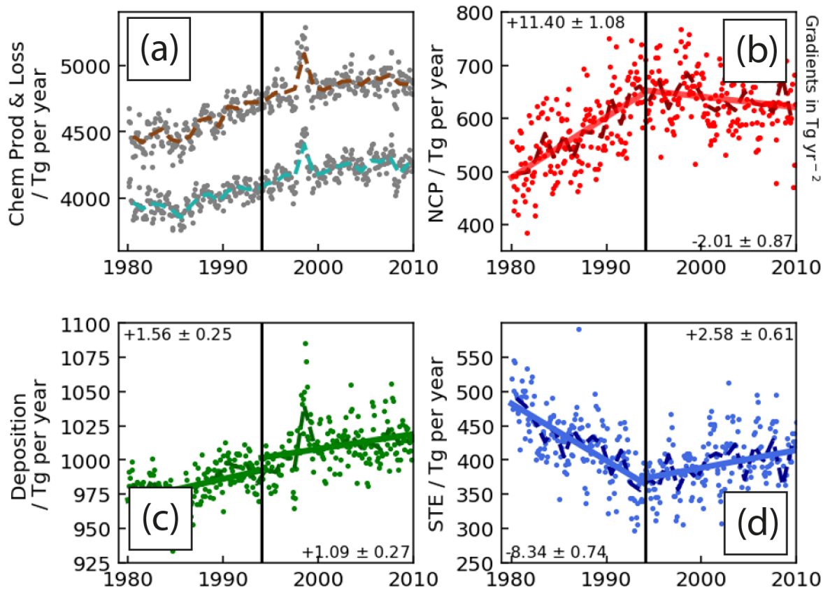
Figure 2: behaviour of the fluxes controlling the tropospheric ozone burden. a: Chemical production and loss. (b): Net ( P_{O_3}-L_{O_3} ) chemical production. (c): Deposition of Ox and NO_y . (d): Net STT of ozone. Dots represent the deseasonalized global monthly mean fluxes. Dashed lines show annual means. Solid lines show a linear fit to the data, based on a break-point of 1994. Captions show trend in Tg per year.
