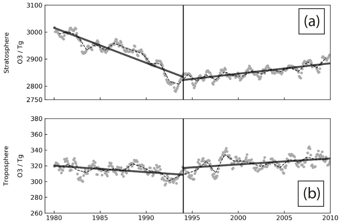
Figure 1 - Transient behaviour of stratospheric (a, upper) and tropospheric (b, lower) ozone burden. The seasonal cycle in ozone has been removed. The breakpoint at 1994 is a guide for the eye and is explained in the text
