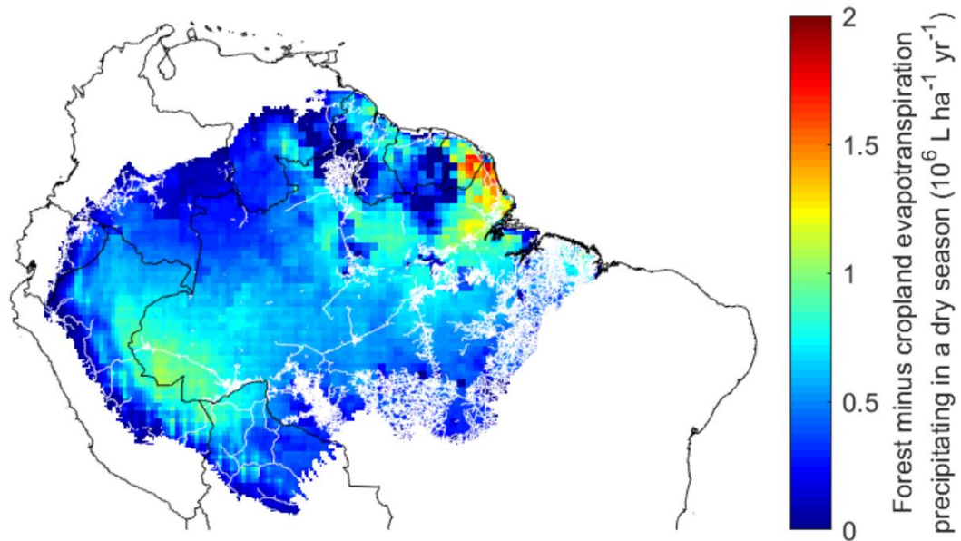
Figure 4: The effects of deforestation on rainfall recycling within dry seasons in the Amazon ( 10^6 \text{ L ha}^{-1} \text{ yr}^{-1} ) with its major roads. Because the map shows how many million liters of water each hectare of forest conversion to cropland would precipitate less elsewhere in the Amazon during the local dry season, the depicted values are smaller than total forest evapotranspiration. The results depend on both the local evapotranspiration calculations and the atmospheric moisture-tracking simulations. The roads [48] are given in white.
