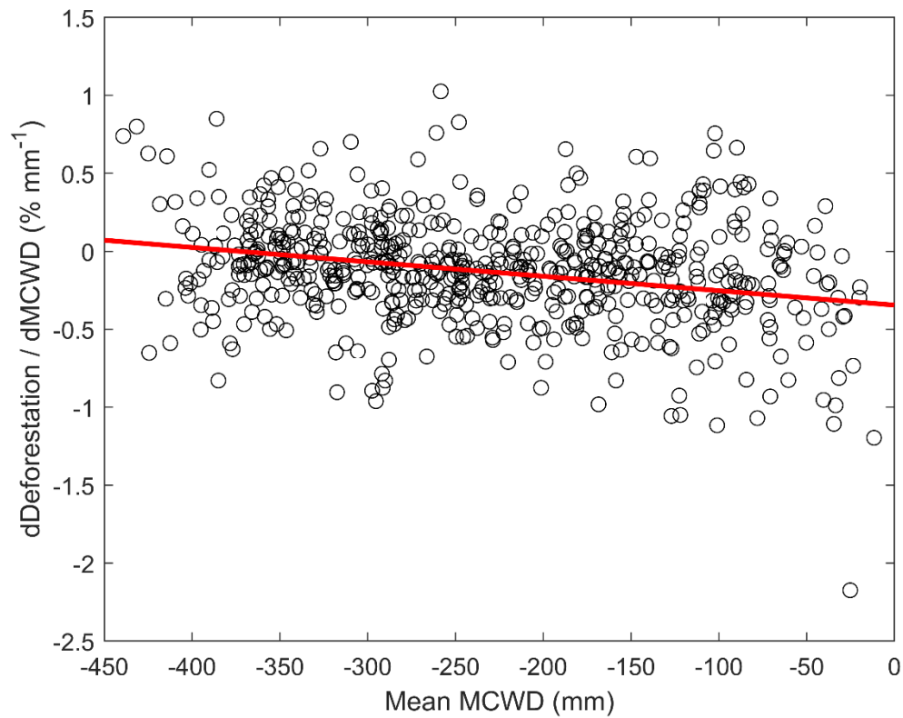
Figure S5: The effect of mean Maximum Climatological Water Deficit (MCWD in mm) over 2001–2014 on the sensitivity of deforestation to MCWD ( \Delta\text{Deforestation} / \Delta\text{MCWD} in \% \text{ mm}^{-1} ) on a 1^\circ basis. Because the explained variance by the regression is small ( R^2 = 0.076 ) we assume the mean value for \Delta\text{Deforestation} / \Delta\text{MCWD} across MCWD in our calculations: -0.13 \text{ \% mm}^{-1} (95% CI [-0.14, -0.12] ).
