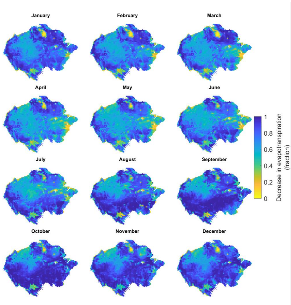
Figure S6: The decrease in evapotranspiration that would occur if all forest would be converted to cropland. The results are averaged over 2003–2014 and given as fraction of total evapotranspiration.
