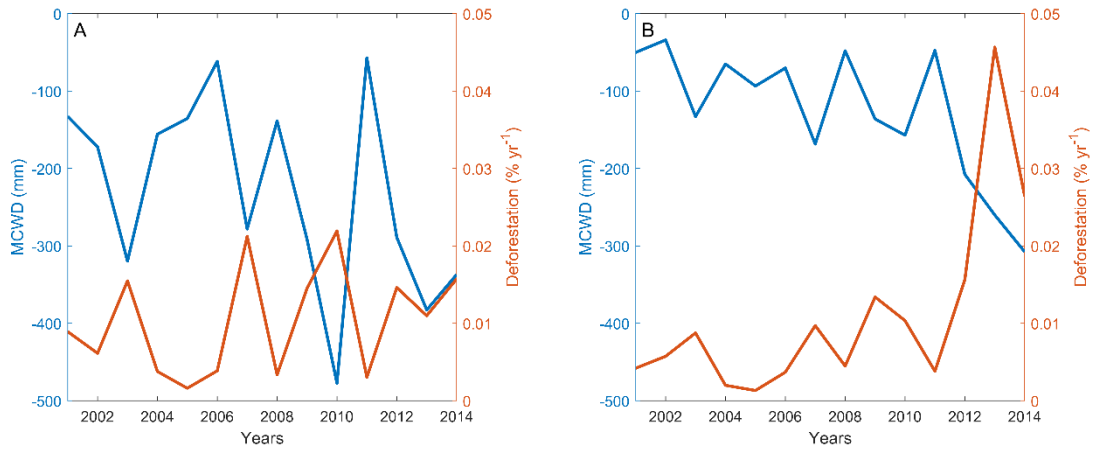
Figure S2: Two examples of time series of Maximum Climatological Water Deficit (MCWD in mm) and deforestation ( \% \text{ yr}^{-1} ), showing the negative correlation between the two. For illustrative purposes we took the two cells (Fig. 2D) with the lowest p value. A) Cell located at 1.5^{\circ}\text{N} , 64^{\circ}\text{W} . B) Cell located at 0.5^{\circ}\text{N} , 65^{\circ}\text{W} .
