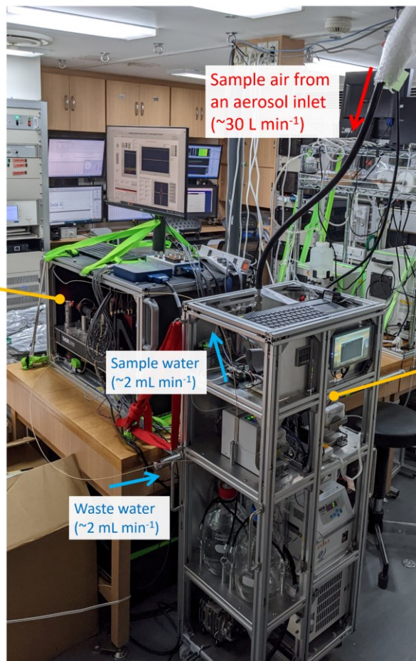
730 FIG. S2. Photo of the complex amplitude sensor connected to the aerosol-into-water collection system, installed in a cabin of research vessel SHINSEI MARU during the observation campaign.
