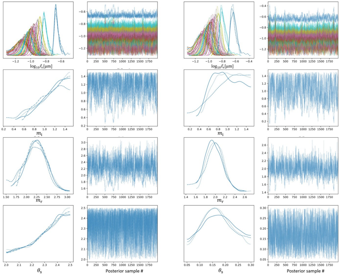
FIG. S10. Same as Figure S6 for ambient BC on July 27 th .
