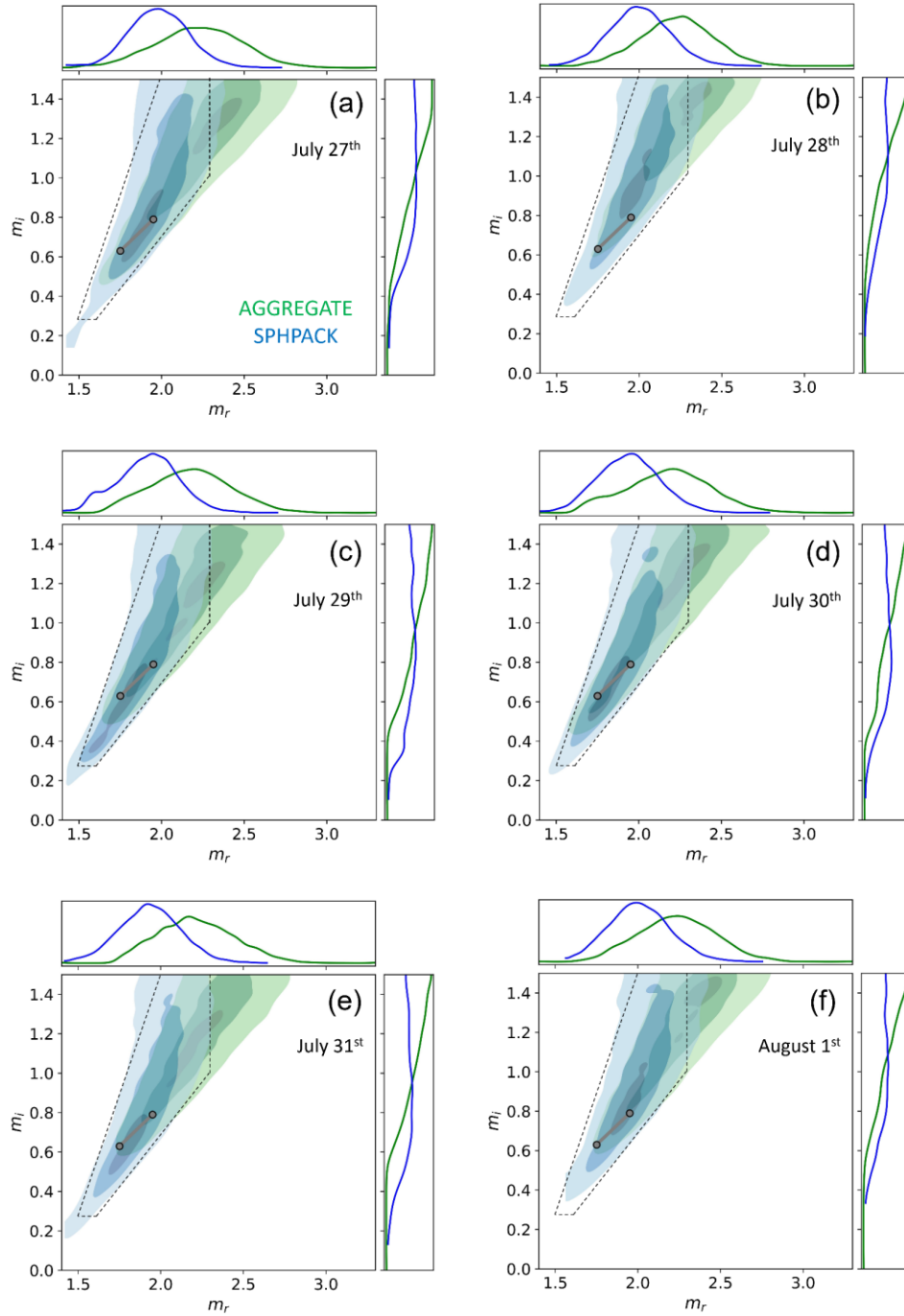
695 FIG. 9. Same plot as Figure 8 but for ambient BC results derived from the data shown in Figure 7. In each panel, the BB06-l and -h values were also shown by gray-filled circles for comparison. The dashed lines indicate the borderlines of our suggested plausible (m_r, m_i) domain for ambient BC refractive index. The SPHPACK is more realistic shape model than the AGGREGATE for the reasons explained in the main text.
