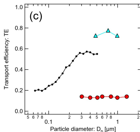
FIG. S4. Laboratory test results of the aerosol-into-water collection system using three different particulate materials (Polystyrene, Silica, and ambient BC). (a) Sampling efficiency (SE) is the number fraction of aerosol particles collected in water and transported to the outlet buffer tube. (b) Collection efficiency (CE) is the number fraction of aerosol particles removed from the sampled airflow. (c) Transport efficiency (TE) is the number fraction of removed aerosol particles transported to the outlet buffer tube. SE=CE \times TE . The particle-size dependence of CE would be due to the size dependence of the critical supersaturation and spatiotemporal inhomogeneity of supersaturation due to insufficient mixing of steam jet and sample airflow. The strong material dependence of TE would be due to the difference in the zeta potential of waterborne particles that determine the tendency of adsorption of waterborne particles on the inner wall of the spiral tube. Commercial-size standard microspheres (ThermoFisher Scientific) were used for polystyrene and silica samples. The number concentrations of each size standard particulate sample in air and water were respectively measured using an optical particle counter (SPS30, Sensirion) without and with a Marin-5 nebulizer (Teledyne CETAC Technologies). For ambient BC, size-resolved number concentrations in air and water are respectively measured using the single-particle soot photometer (SP2; Droplet Measurement Technologies) without and with a Marin-5 nebulizer. Ambient BC sampling was performed on the Hongo campus of the University of Tokyo on May 10, 2022.
