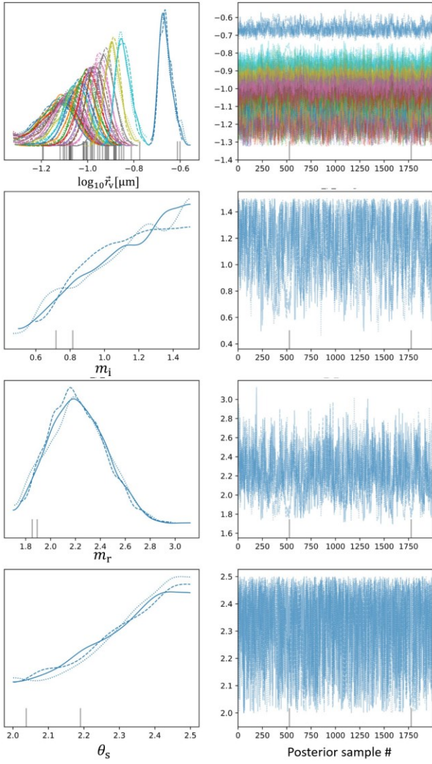
FIG. S14. Same as Figure S6 for ambient BC on July 31 st .
