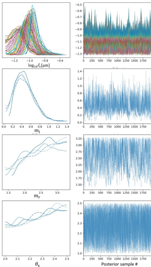
785 FIG. S8. Same as Figure S6 for Hematite-KJ.
