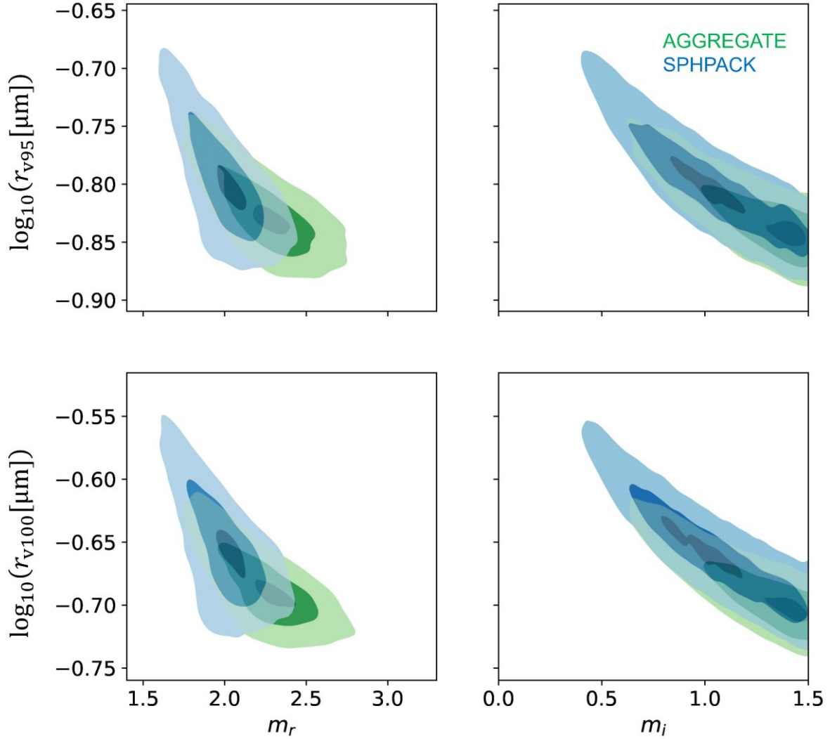
705 FIG. 10. Joint density plots of the posteriors of real and imaginary parts of refractive index, m_r , m_i , and the two volume-equivalent radii corresponding to the 95 th and 100 th percentiles of arclength coordinate of the principal curve, r_{v95} , r_{v100} for ambient BC sampled on August 1 st . The three-level contour shows the 90%, 50%, and 10% highest density credibility regions in each of the AGGREGATE (green) and SPHPACK (blue) models. The SPHPACK is more realistic shape model than the AGGREGATE for the reasons explained in the main text.
