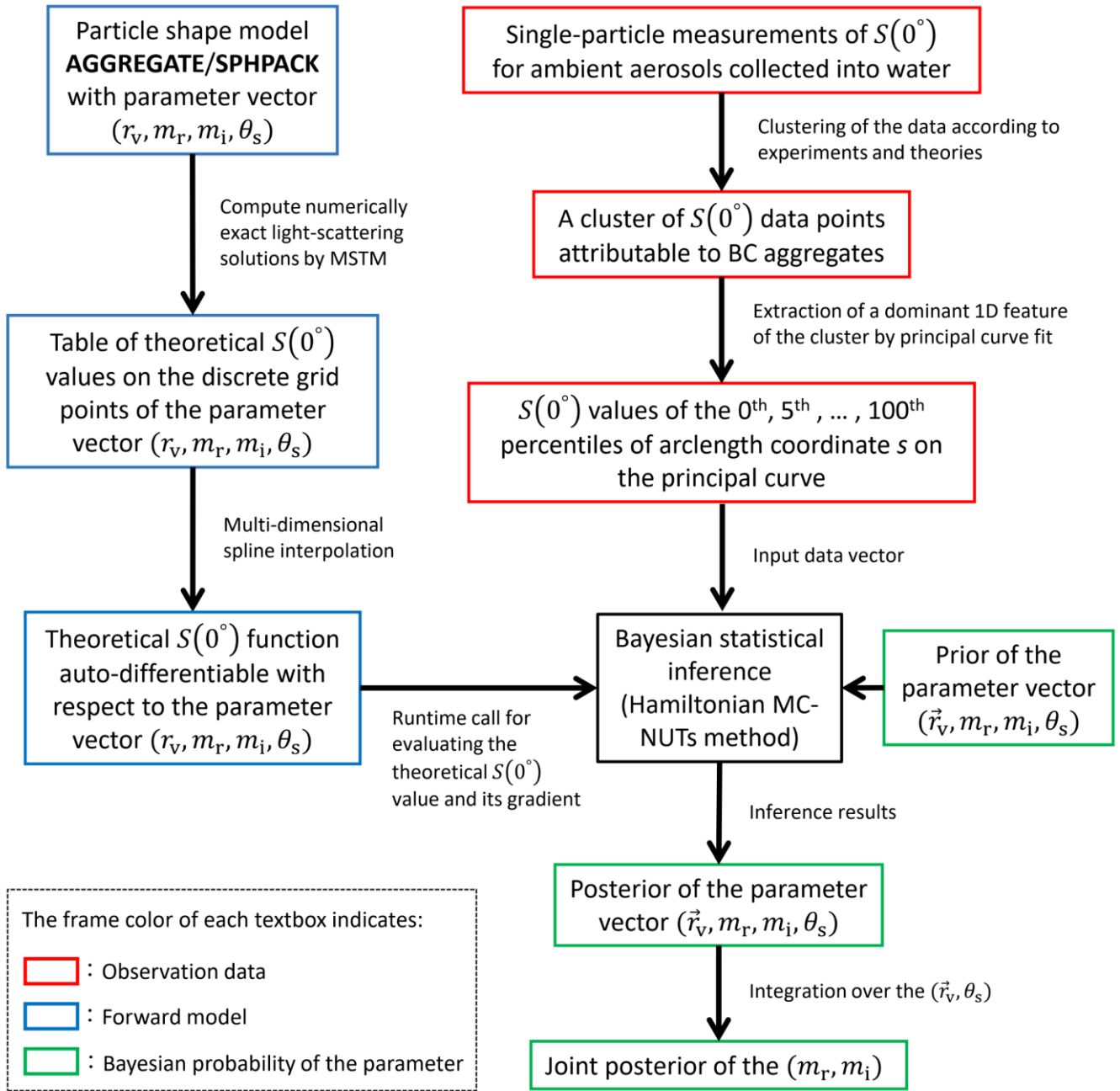
FIG. 3. Flow chart of the computational and data processing procedure in our method for constraining the refractive index of ambient BC from the complex forward-scattering amplitude measurements. The frame color shows either of data, forward model, or Bayesian probability as illustrated in the lower-left part of the Figure.
