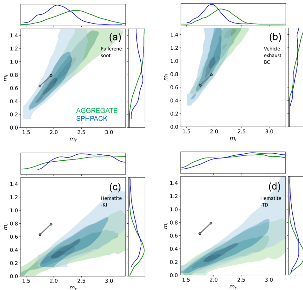
690 FIG. 8. Posterior of real and imaginary parts of complex refractive index ( m_r , m_i ) for each laboratory sample derived from the data shown in Figure 6. (a) Fullerene soot, (b) Vehicle exhaust BC, (c) Hematite-KJ, (d) Hematite-TD. The three-level contour shows the 90%, 50%, and 10% highest density credibility regions for each of the AGGREGATE (green) and SPHPACK (blue) models. Marginalized density distributions of m_r and m_i are also shown along horizontal and vertical axes, respectively. In each panel, the BB06-l and -h values were also shown by gray-filled circles for comparison. In panels (a) and (b), the SPHPACK is more realistic shape model than the AGGREGATE for the reasons explained in the main text.
