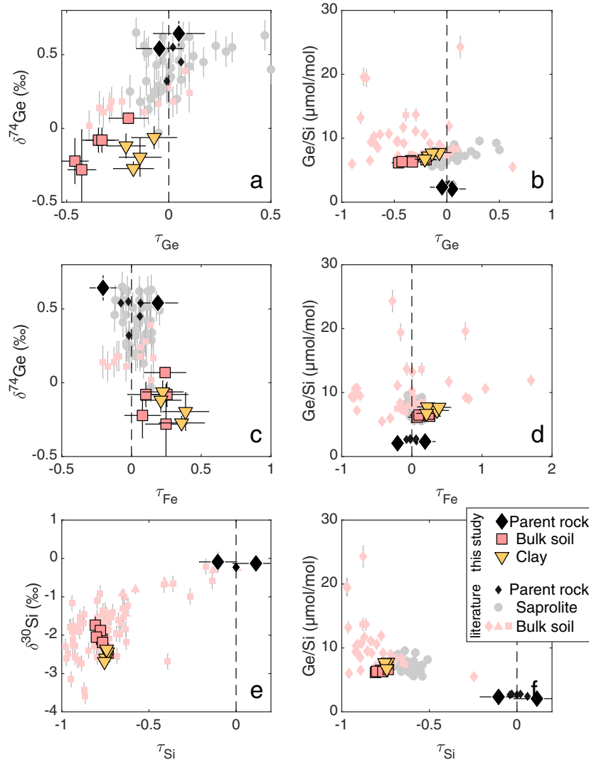
Figure 5. Relationships of \delta^{74}\text{Ge} , \delta^{30}\text{Si} , and Ge/Si vs. fractional elemental loss ( \tau < 0 ) or gain ( \tau > 0 ) of Ge, Fe, and Si in volcanic soils (Eq. S1). Small symbols are published values of Kurtz et al. (2002) (Ge/Si; diamonds) and Bern et al. (2010) ( \delta^{30}\text{Si} corrected for dust inputs; squares) for basaltic soils in Hawaii, Qi et al. (2019) for a basaltic weathering profile in Hainan island, China ( \delta^{74}\text{Ge} and Ge/Si; squares and circles), and Opfergelt et al. (2012) for an andesitic soil sequence in Guadeloupe island, French Indies ( \delta^{30}\text{Si} ; triangles).
