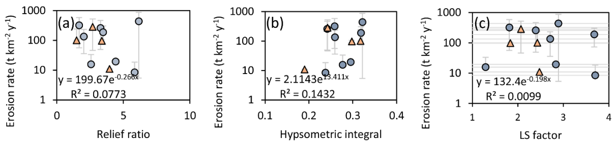
Fig. 9. Bivariate relationship between topographic variables and erosion rates in Peninsular Indian catchments. (a) relief ratio- erosion rate relation; (b) hypsometric integral-erosion rate relation; (c) slope-length factor- erosion rate relation.
