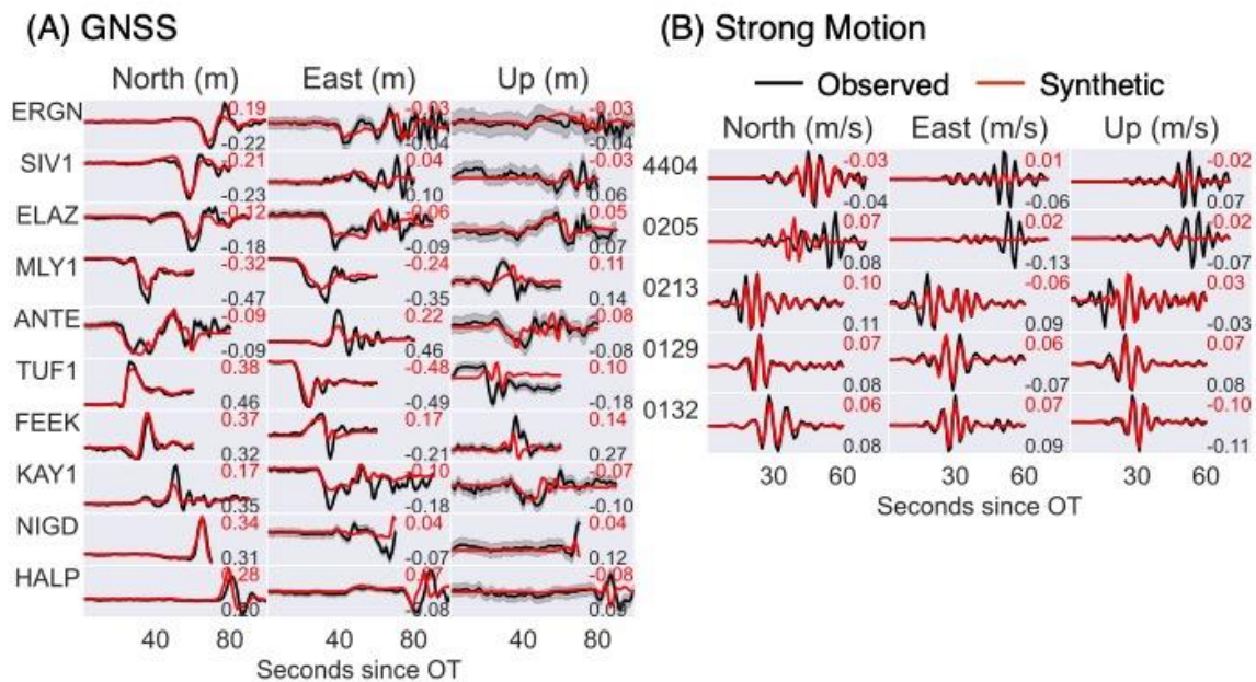
Figure 6. Fits to the HR-GNSS (A) and strong motion (B) for the best fitting M_w 7.6 model. Black is the observed and red the modeled waveforms. Labeled numbers show the peak amplitudes for each waveform.
