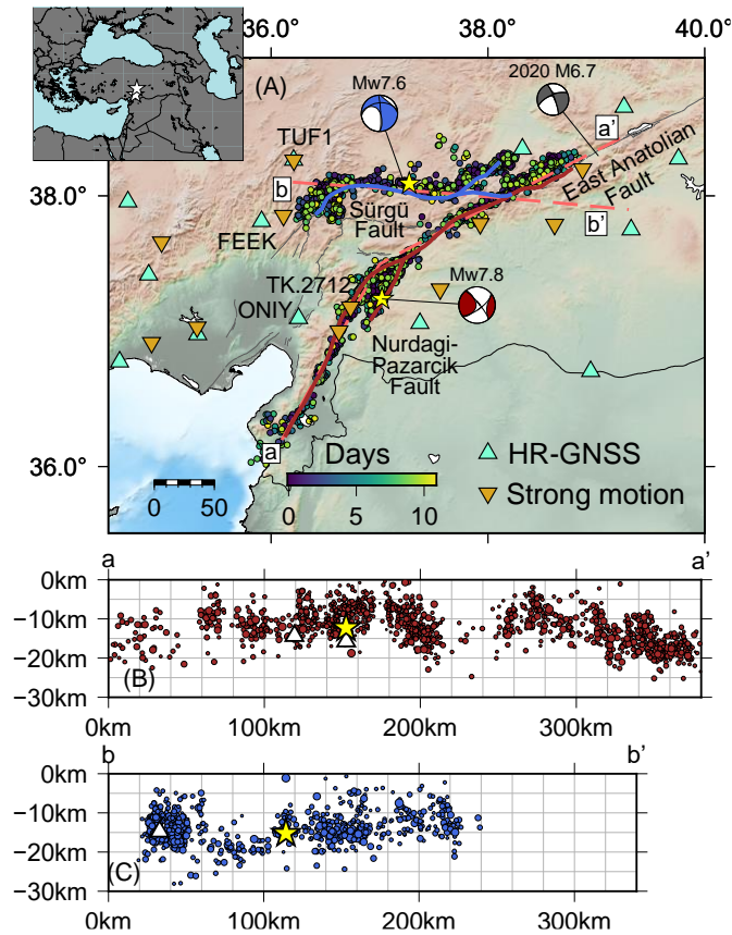
Figure 1. (A) Simplified map of the study region showing the focal mechanisms for both events in the earthquake doublet. Known and mapped fault surface traces are shown as dark grey lines. The East Anatolian fault and Sürgü fault are labeled. The inferred Nurdağı-Pazarcık Fault is labeled as well. The thick red line denotes the surface trace of the geometry used for inversion of the Mw 7.8 event. The thick blue line is the surface trace of the geometry assumed for the Mw7.6 earthquake. The first 11 days of relocated aftershocks are shown as filled circles (color varying according to days origin time). HR-GNSS and strong motion stations used in the inversions are depicted by triangles and inverted triangle respectively. The grey moment tensor is for the M6.7 2020 Doğanyol-Sivrice earthquake. (B) Aftershock cross section across profile a-a'. (C) Aftershock cross section across profile b-b'. In both (B) and (C) stars are the doublet hypocenters and triangles denote events with M_w > 6 .
