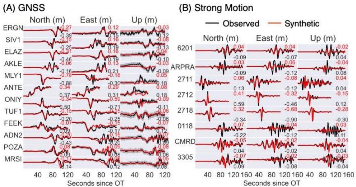
295 Figure 4. Fits to the HR-GNSS (A) and strong motion (B) for the best fitting M_w 7.8 model. Black is the observed and red the modeled waveforms. Labeled numbers show the peak amplitudes for each waveform.
