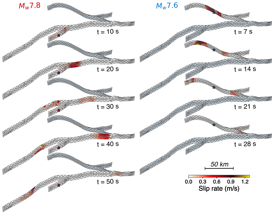
300 Figure 5. Snapshots of rupture propagation for both events. Plotted is slip rate on each subfault at specified instants in time. Star denotes relocated hypocenter location.
