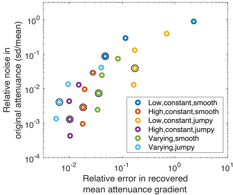
Figure 4. Relationship between the retrieved, mean \delta atn_c / \delta t and the amount of instrument noise in the original attenuation signal (tested levels were 1, 3, 10, and 30 \times 10^{-3} \text{ m}^2 \text{ m}^{-2} ). Relative noise is expressed as the standard deviation of the noise divided by the mean attenuation in the original simulated data. Symbol colors and short legend labels correspond to the simulated datasets shown in Fig. 3, upper left panel. Symbols outlined in black correspond to the timeseries shown in Fig. 3 (noise SD of 0.003 \text{ m}^2 \text{ m}^{-2} ).
