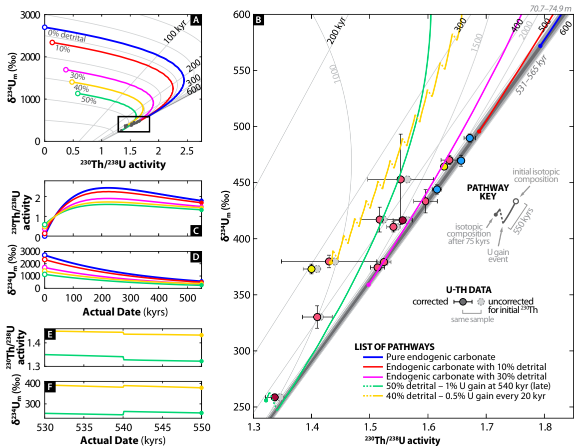
Figure 14: Possible pathways of uranium-thorium isotopic evolution that may explain the outlying data at \sim 70\text{--}75\text{ m} . See caption in Fig. 13 for explanation of symbology. [A] Plot showing initial isotopic composition and evolution of pathways over 550 kyr. [B] View of the isotopic evolution of samples within the extent represented by the rectangular box in Panel A. The gray triangular wedges representing the expected age range of samples from this depth range occupies a much narrower area in ^{230}\text{Th}/^{238}\text{U} activity- \delta^{234}\text{U} space compared to Fig. 13. The starting composition of the pure endogenic carbonate is 1.8 ppm ^{238}\text{U} and 2700‰ for \delta^{234}\text{U}_{\text{initial}} . The detrital component has the same composition as that from Fig. 13, 30% limestone and 70% aluminosilicate material. These calculations assume that uranium gain occurs with a \delta^{234}\text{U} ratio equal to the \delta^{234}\text{U}_{\text{initial}} of the sample. [C] and [D] Change in isotopic evolution as the proportion of detrital material increases. [E] and [F] Change in isotopic evolution after uranium gain.
