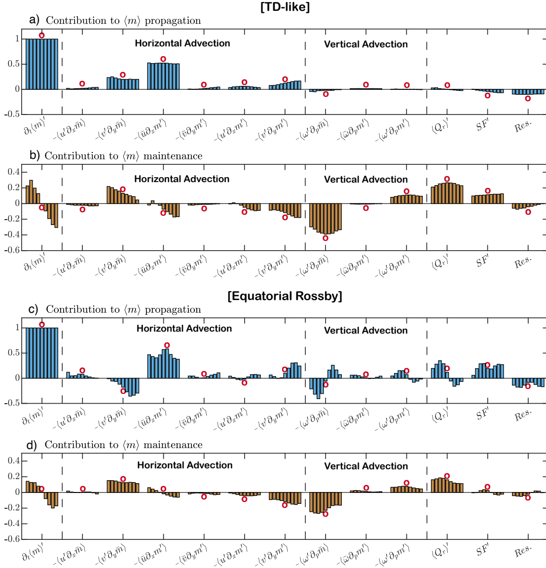
Fig. 9. The average contribution of each term in the MSE budget Eq. (6) to the propagation (blue bars) and maintenance (brown bars) of the TD-like and Equatorial Rossby waves over the tropics. The contribution of each horizontal and vertical MSE advection term is delimited by dashed black lines. Red circles represent the peak of convection at the base point at day 0. The four bins before and after of peak of convection represent the lag regressions from day -2 to day +2 at every 12 hours for TD-like waves and from day -8 to day +8 at every 2 days for Equatorial Rossby waves.
