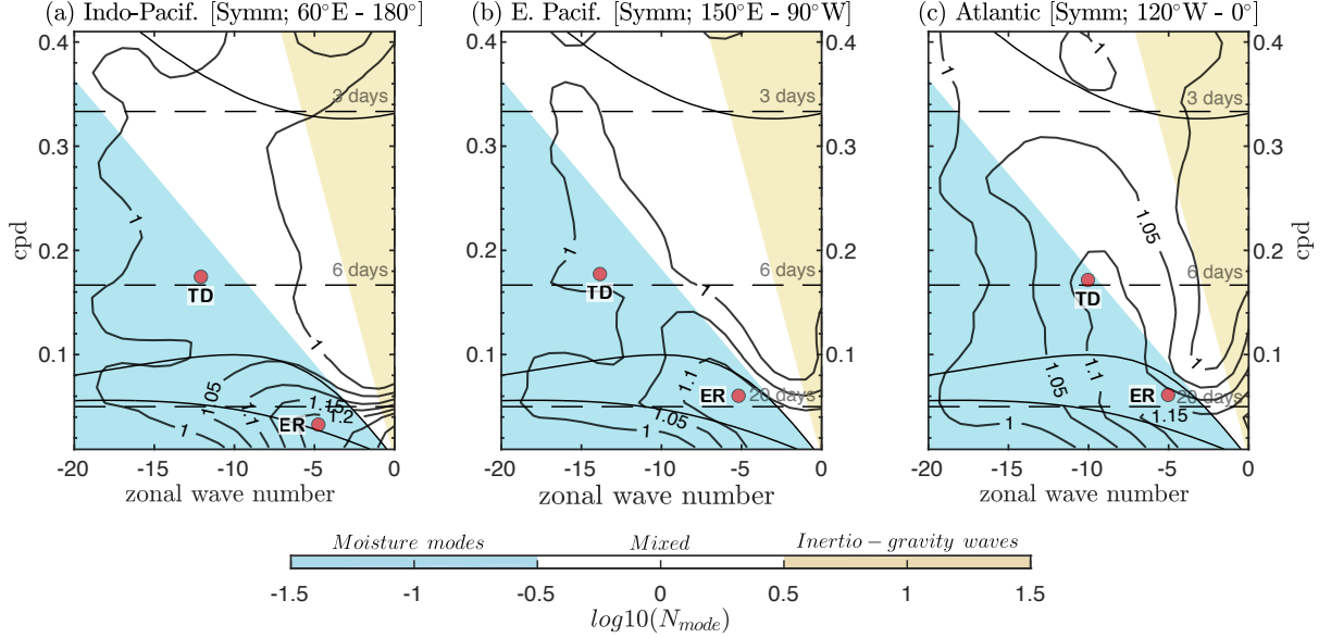
FIG. 7. Regional wavenumber-frequency power spectrum (contours) of the symmetric component of CLAUS T_b calculated for three different regions of the tropics between 10^\circ\text{N} – 10^\circ\text{S} : (a) Indo-Pacific ( 60^\circ\text{E} – 180^\circ ), (b) Eastern-Pacific ( 150^\circ\text{E} – 90^\circ\text{W} ), and (c) Atlantic ( 120^\circ\text{W} – 0^\circ ). The solid dispersion curves correspond to 8 and 70 m equivalent depths. The functional form of the tapering window is the same as described in Wheeler and Kiladis (1999). Background spectra were estimated separately for the regional domain, using the smoothing procedure of Dias and Kiladis (2014). Contour interval is 0.05. Shadings represent wavenumber-frequency distribution of base 10 logarithm of N_{mode} following a similar procedure of Adames (2022). Blue shading represents tropical systems that can be categorized as moisture modes, yellow can be considered inertio-gravity waves, and white represents mixed systems. Orange circles approximately represent the average zonal wavenumber and frequency of the corresponding TD-like and Rossby wave for the different regions.
