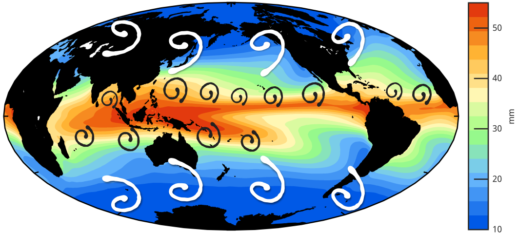
FIG. 1. Annual mean distribution of column-integrated water vapor ( \langle q \rangle ). The black whirls denote tropical eddies that stir column moisture ( q ) in the tropics, behaving as a tropical analog to mid-latitude eddies (white whirls).
