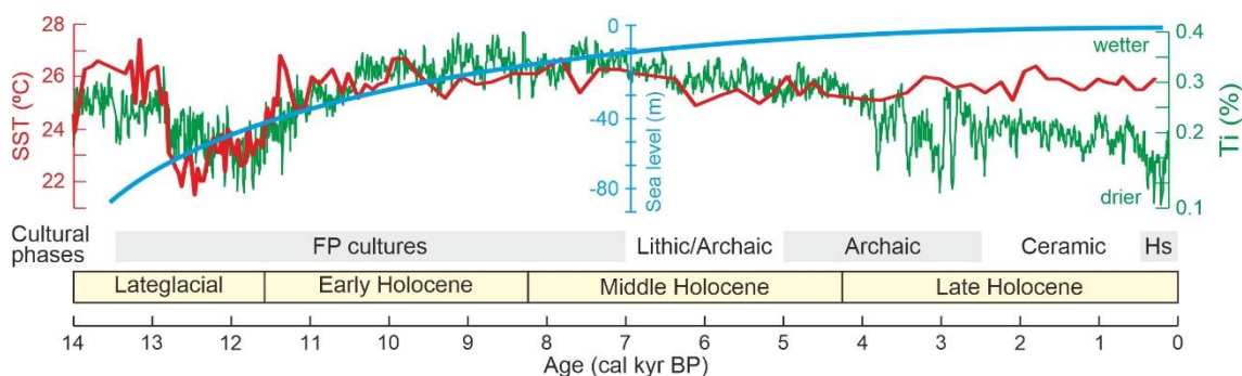
Figure 5. Holocene paleoclimatic (Haug et al., 2002, Lea et al., 2003), paleoestatic (Khan et al., 2017) and cultural trends and events (Rull, 2022b). SST, Sea Surface Temperature; Ti, Titanium concentration as a moisture proxy.
