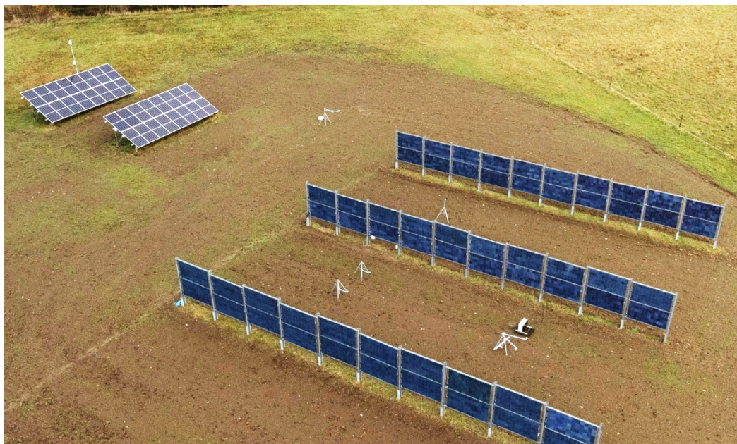
Figure 3. Aerial picture of the first agrivoltaic system in Sweden comprising of three vertical bifacial PV rows. Photo credit: IVAR Studios AB.
