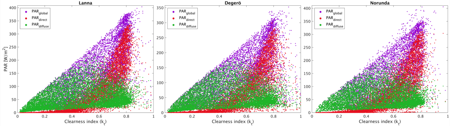
Figure 7. Scatterplots between the clearness index and PAR_{global} , PAR_{direct} and PAR_{diffuse} for the period 2016 – 2018 at the studied ICOS Sweden network stations: Lanna (left), Degerö (middle), and Norunda (right). Hourly values at midpoint are used.
