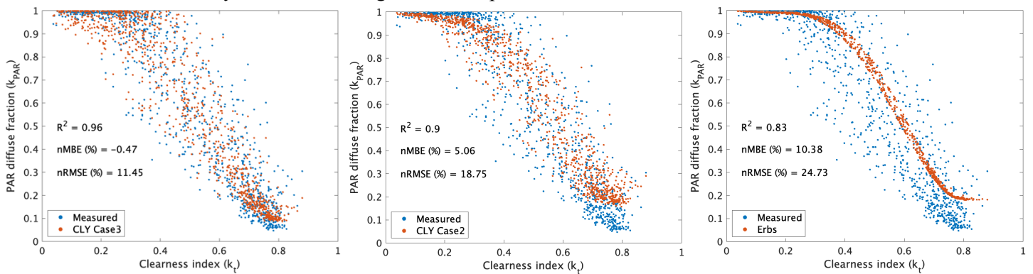
Figure 10. PAR diffuse fraction measured data plotted against the clearness index for the agrivoltaic site close to Västerås. The estimated results from the proposed PAR separation model CLY are overlaid. The total number of data points (994) in each plot refers to 1/3 of the dataset described in Section 2.3, where 2/3 of the dataset (1930 data points) are used for model calibration. The nRMSE [%], nMBE [%] and R^2 are displayed. Left: results of applying CLY model with locally calibrated coefficients – Case 3. Middle: results of applying CLY model with coefficients calibrated to the combined data of 3 ICOS-Sweden stations – Case 2. Right: results of applying ERBS model.
