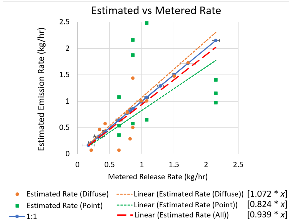
Figure 7: Estimated emission vs. metered release rates for all detections, separated by release method (point – green squares, diffuse – orange circles). This plot illustrates the fit relationships between metered and estimated rates for the entire set of detections achieved during this testing as well as for the detections separated by release method. Linear fits with no intercept indicate bias of +7.2% and -17.6% for diffuse (orange dotted line) and point (green dotted line) releases, respectively, while the fit to the entire dataset indicates a bias of -6.1% (red dashed line).
