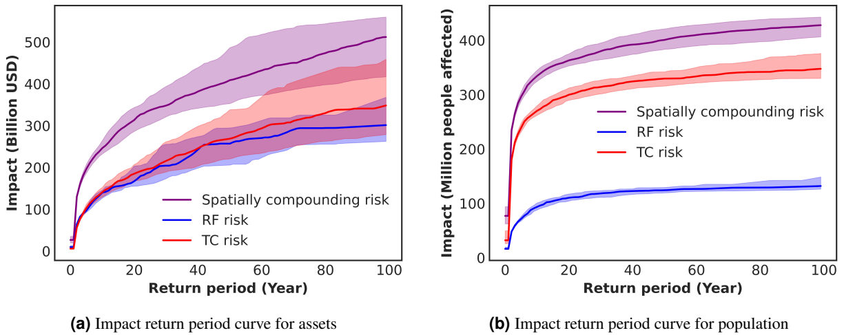
Figure 3. Impact return period curves of RF, TC and the spatial compounding of both, at 1.0 °C. The shaded area is the 90th confidence interval for 1000 samples of 500 years, while the full lines represent the median of all samples.
