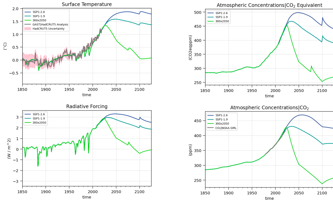
Figure 2. Pathways SSP1 2.6 5,6 , SSP1 1.9 5,6,7,8 , and 300 x 2050 show emissions and emissions reductions starting in 2010 through 2125. Historical emissions through 2020 are included in the pathway 300 x 2050.
