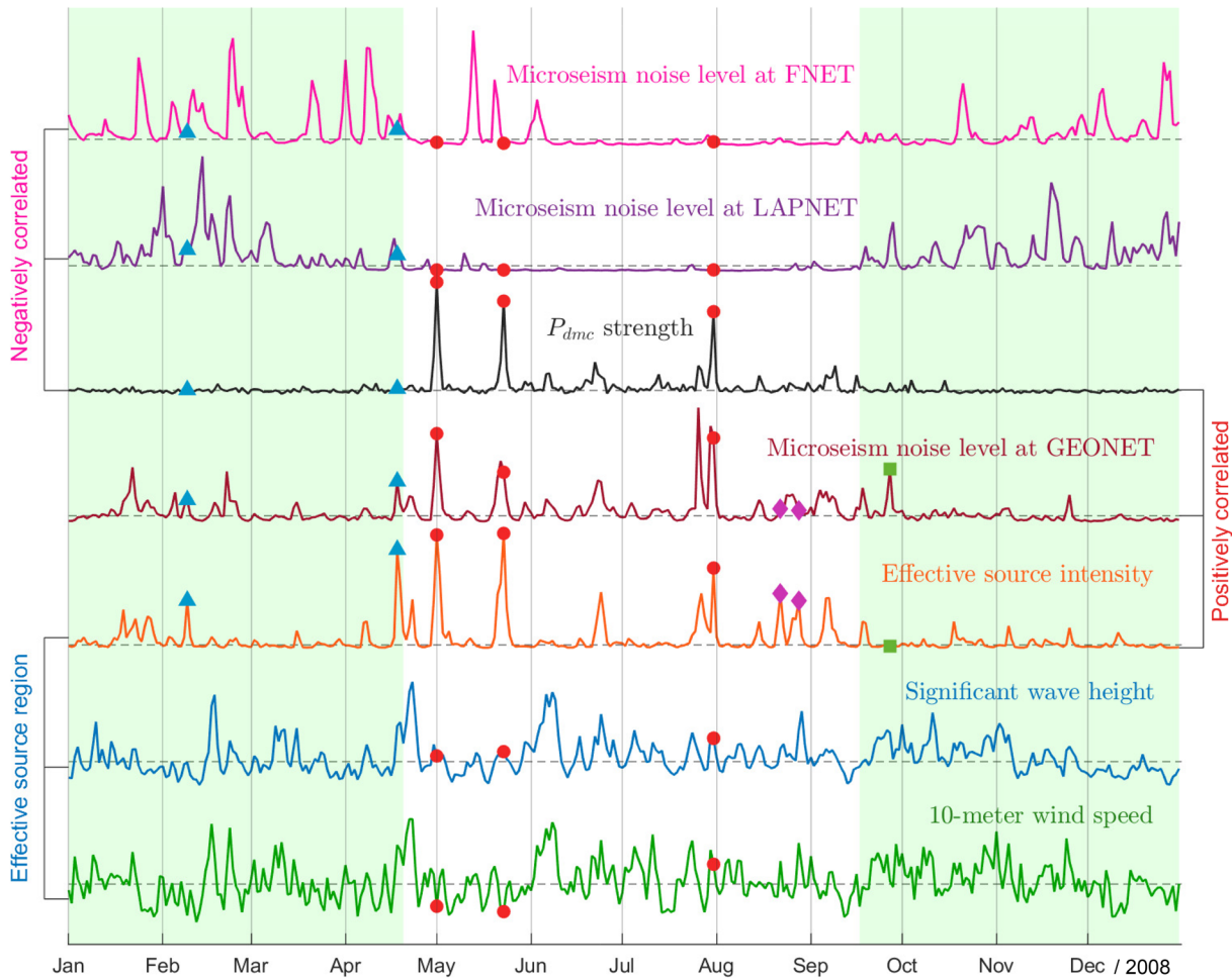
Figure 6. Temporal variations of daily P_{dmc} strength, microseism noise levels at three networks, and average wind speeds, wave heights, and microseism excitations in the effective source region. The curves are normalized by their own maximums. Dashed horizontal lines denote their respective medians. Symbols mark some dates cited in the main text. When computing the effective source intensity, the bathymetric factors in Figure 5b and weights in Figure 5c are used. When computing the average wind speeds and wave heights, weights in Figure 5c are used.
