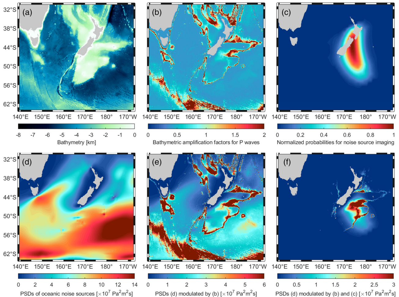
Figure 5. (a) Bathymetry around NZ. (b) Bathymetric amplification factors for P -type waves. (c) Imaging of effective sources obtained from the backprojection of the FNET-LAPNET noise correlations. (d) Annual average of source PSDs in 2008. (e) Source PSDs in (d) modulated by the factors in (b). (f) Source PSDs in (e) further modulated by the weights in (c).
