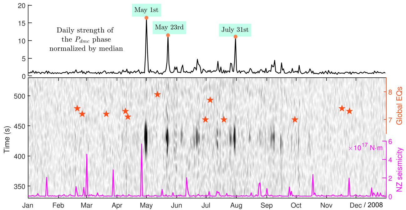
Figure 2. Temporal variations in the strength of daily P_{dmc} signals, in comparison with the daily cumulative seismic moments in NZ (pink line at bottom; for earthquake magnitudes above 2.0 in GEONET catalog) and global large earthquakes (stars; magnitudes above 7.0 in USGS catalog; see Table S1 for a full list of earthquakes in 2008 above magnitude 5.5). The background image is composed of columns of daily envelopes of beamed FNET-LAPNET noise correlations. Darker color represents larger amplitude. The curve on the top shows the daily P_{dmc} strength derived from the daily envelopes. Dates of the three largest peaks are labeled.
