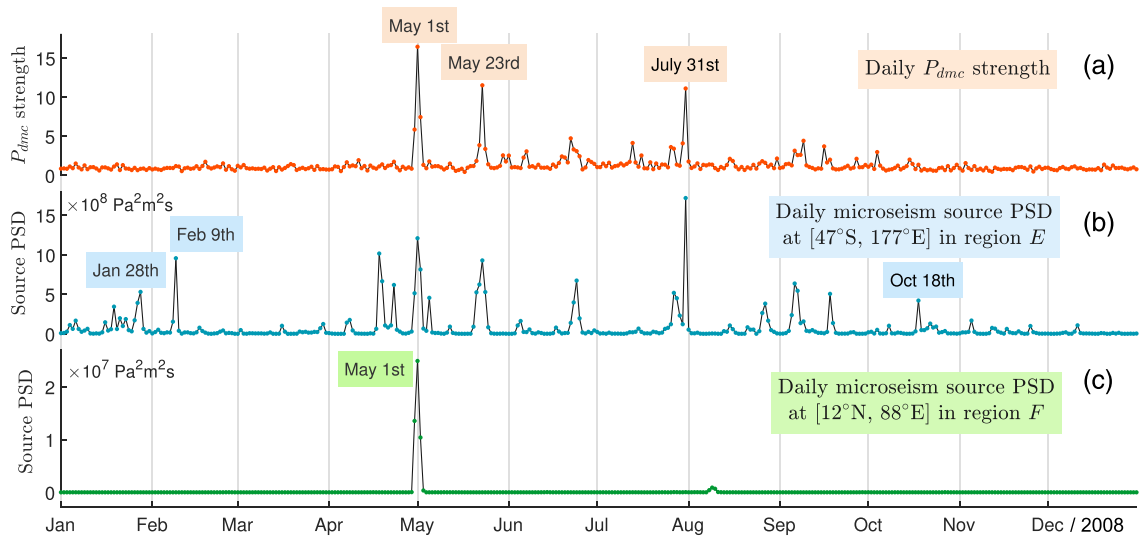
Figure 4. True correlation ( r = 0.73 ) between (a) the P_{dmc} strength from Figure 2 and (b) the power of source at [47^{\circ}\text{S}, 177^{\circ}\text{E}] in the effective source region (E in Figure 3c), and spurious correlation ( r = 0.71 ) between P_{dmc} and (c) the power of source at [12^{\circ}\text{N}, 88^{\circ}\text{E}] in the Bay of Bengal (F in Figure 3c).
