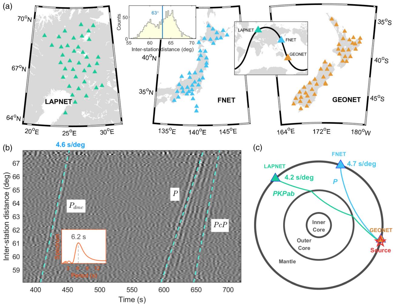
Figure 1. (a) Three regional broadband seismic networks used in this study: (left) the LAPNET array in Finland (38 stations); (center) the FNET array in Japan (41 stations); (right) the GEONET array in New Zealand (46 stations). The histogram inset shows the distribution of the separation distances between the 1,558 FNET-LAPNET station pairs. The center-to-center distance is 63^\circ between LAPNET and FNET and 85^\circ between FNET and GEONET. The global inset shows the geographical locations of the three networks that are aligned on a great circle (dark line). (b) Annual FNET-LAPNET noise correlations that are filtered between 5 and 10 s and stacked over time and in 0.1^\circ interstation distance bins. The spectrum inset indicates that the P_{dmc} phase has a 6.2 s peak period. (c) Ray paths of the interfering waves that generate the P_{dmc} phase. The effective source region is close to GEONET.
