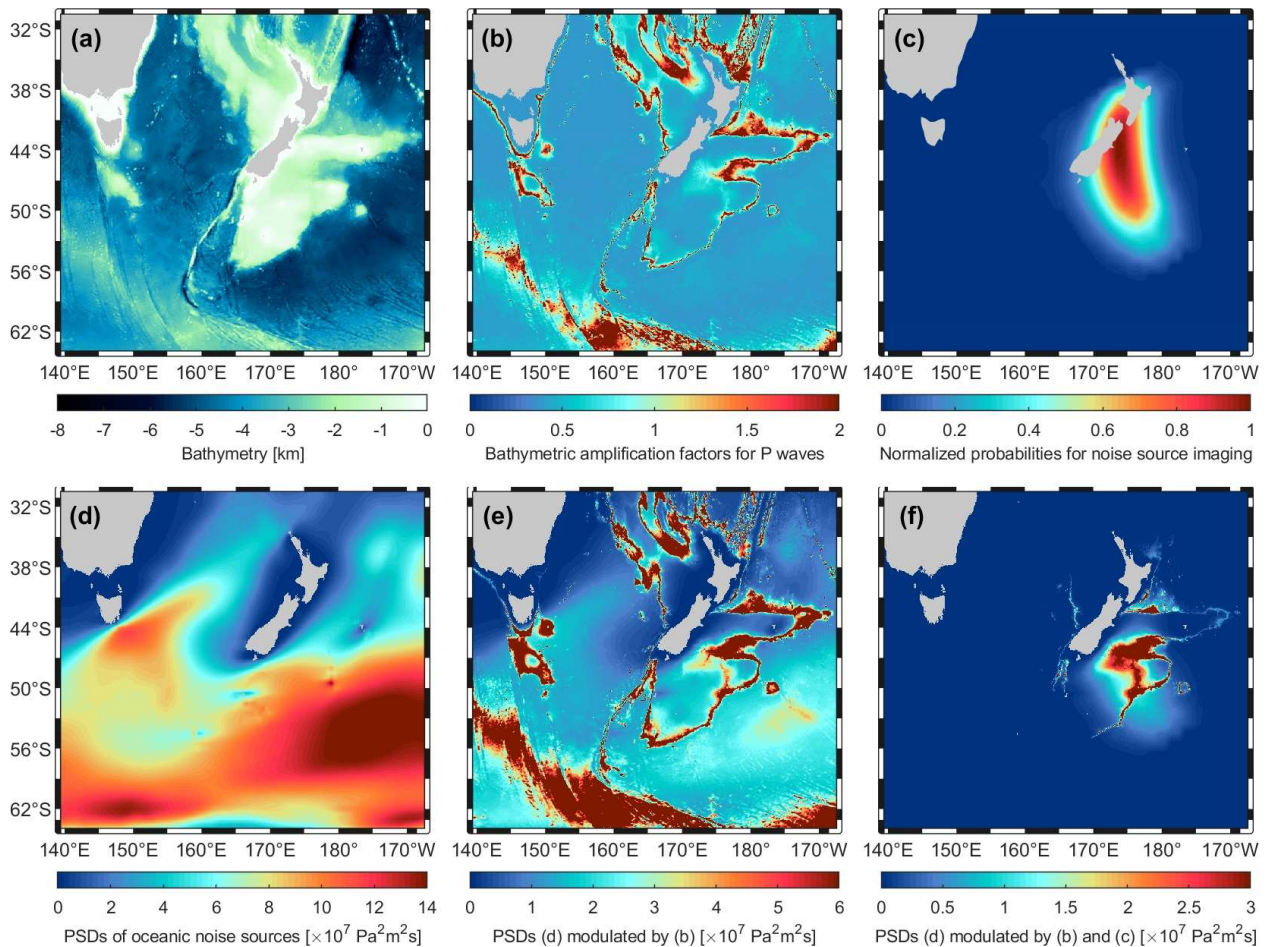
Figure 5. (a) Bathymetry around NZ. (b) Bathymetric amplification factors for P -type waves. (c) Imaging of effective sources obtained from the back-projection of the FNET-
