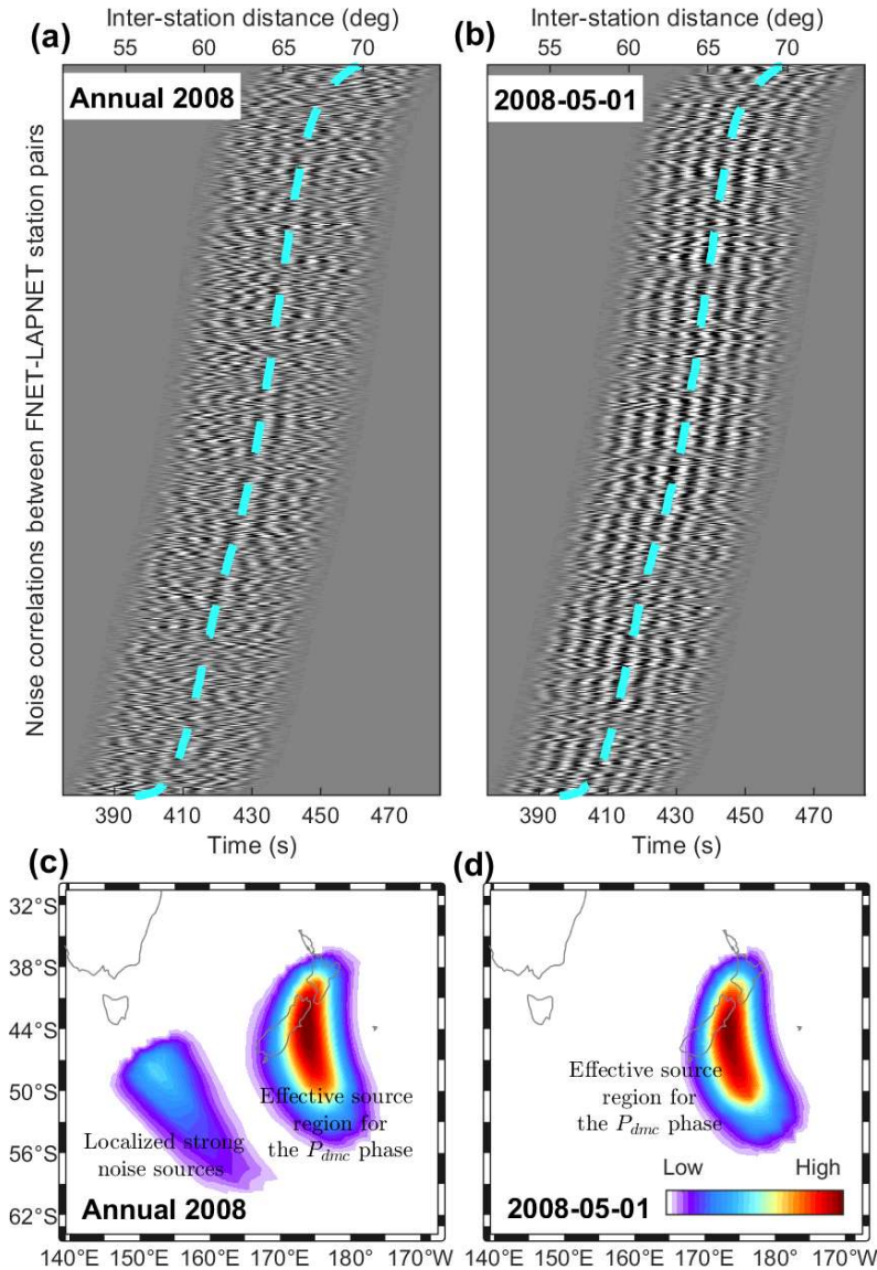
Figure S2. Inter-receiver noise correlations for all FNET-LAPNET station pairs: (a) stacked over the year of 2008; (b) on single day of 2008-05-01. The waveforms are windowed around
