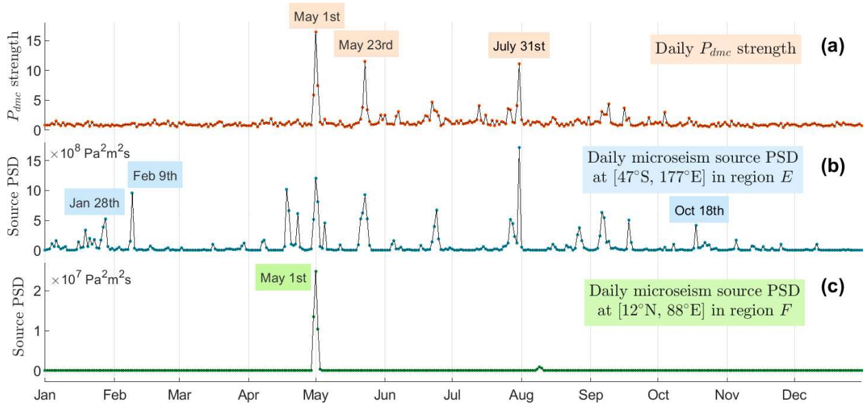
Figure 4. True correlation ( r = 0.73 ) between (a) the P_{dmc} strength from Fig. 2 and (b) the power of source at [47^\circ\text{S}, 177^\circ\text{E}] in the effective source region ( E in Fig. 3c), and spurious correlation ( r = 0.71 ) between P_{dmc} and (c) the power of source at [12^\circ\text{N}, 88^\circ\text{E}] in the Bay of Bengal ( F in Fig. 3c).
