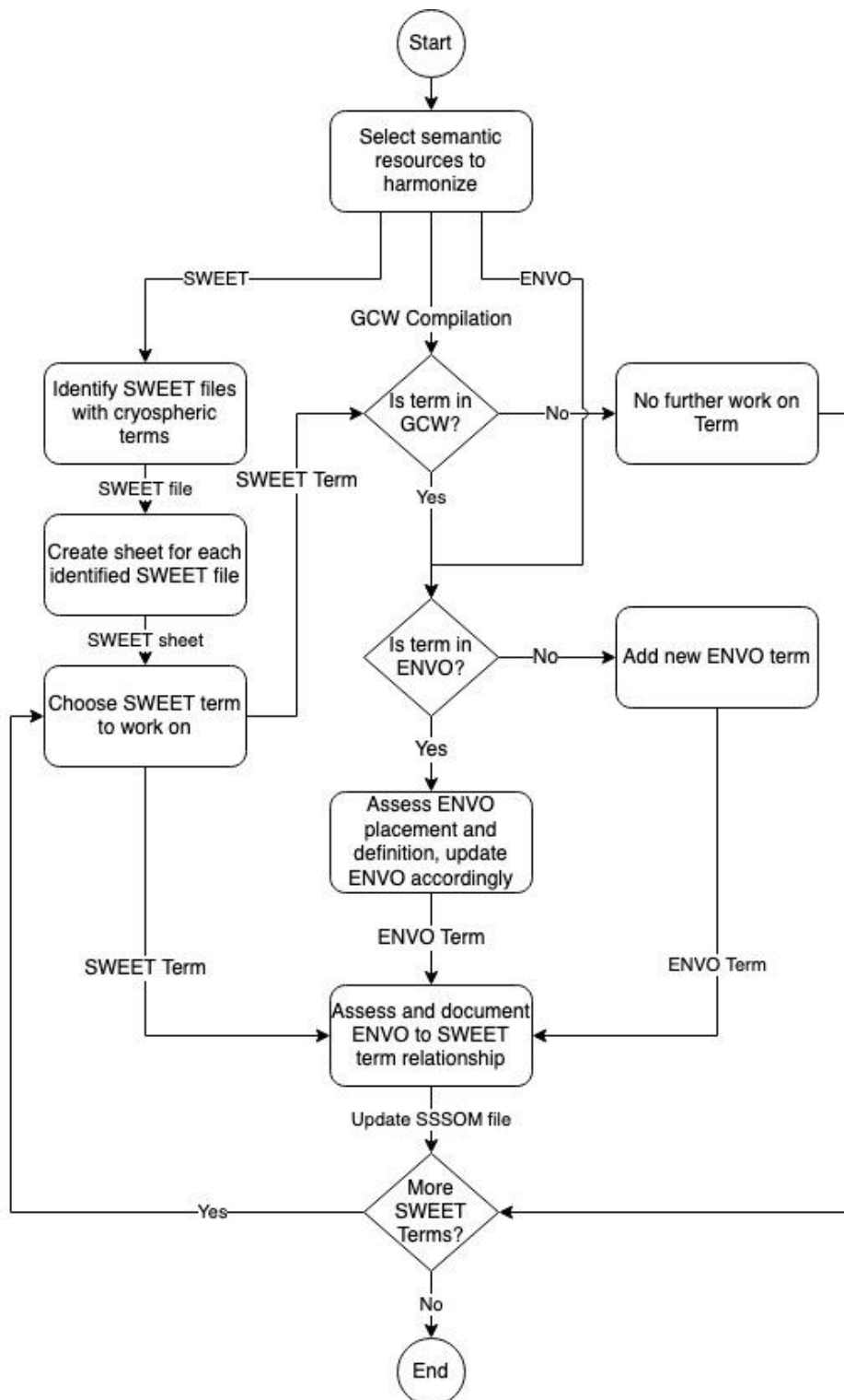
Figure 2: Overview of the harmonization process used in the project and described below. It should be noted that boxes with rounded corners represent processes, while diamonds represent decisions and labeled arrows represent inputs to, triggers for or outputs from a process.
