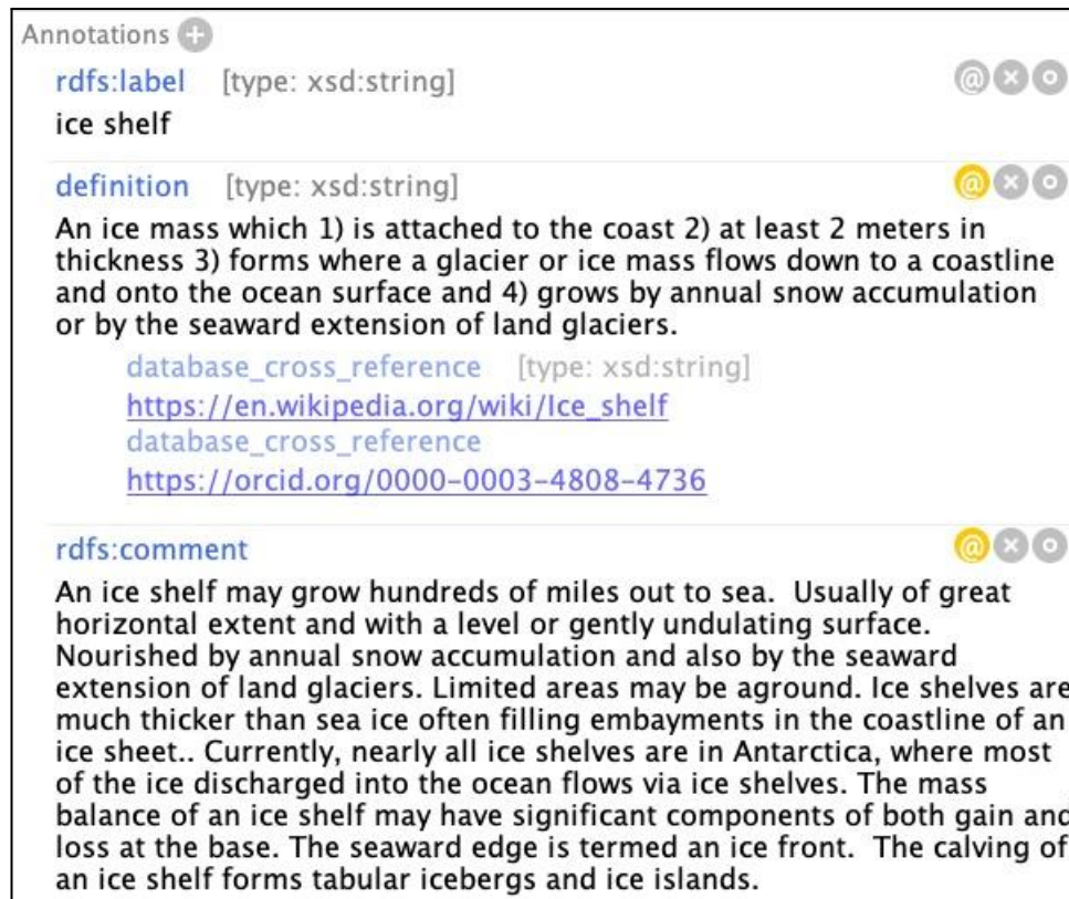
Figure 3: Term added to the ENVO ontology using a GCW derived definition with additional comments.
