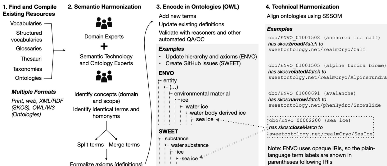
Figure 8: A Generalized Harmonization Workflow.
