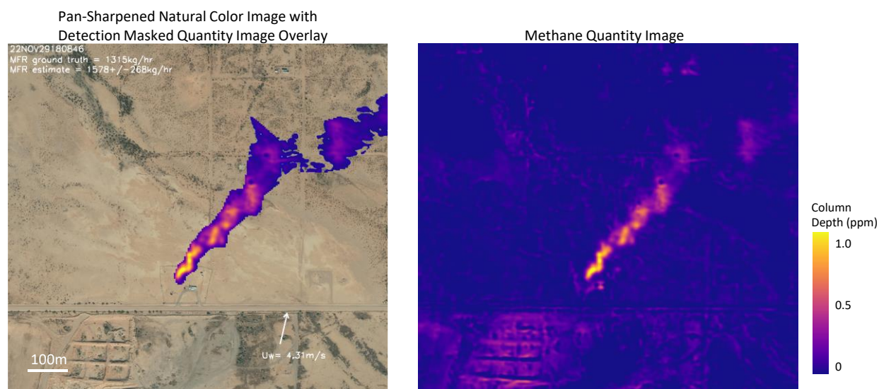
Figure 13. Methane quantity image from November 29, 2022. Ground truth MFR: 1315 kg/hr.
