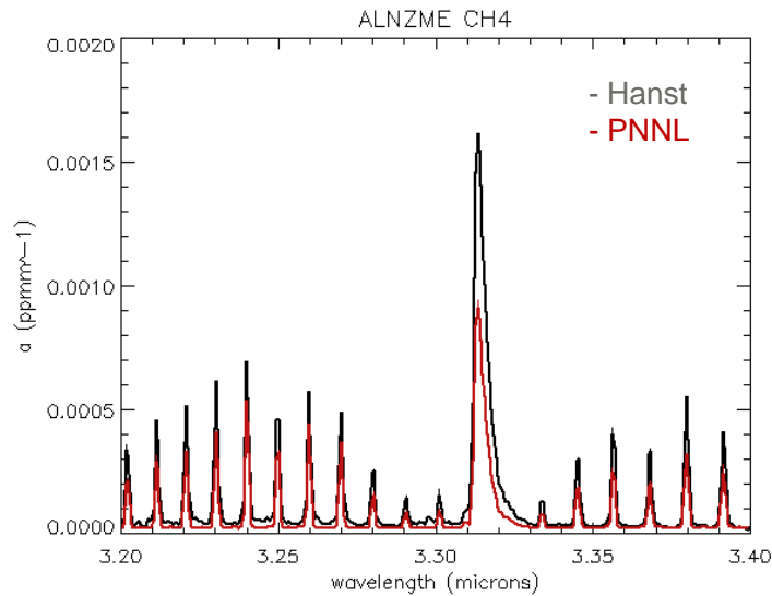
Figure 2. This comparison of the Hanst and the PNNL methane absorption curves reveals the factor-of-2 error.
