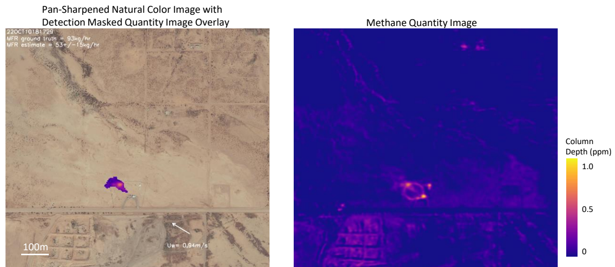
Figure 6. Methane quantity image from October 10, 2022. Ground truth MFR: 93 kg/hr.
