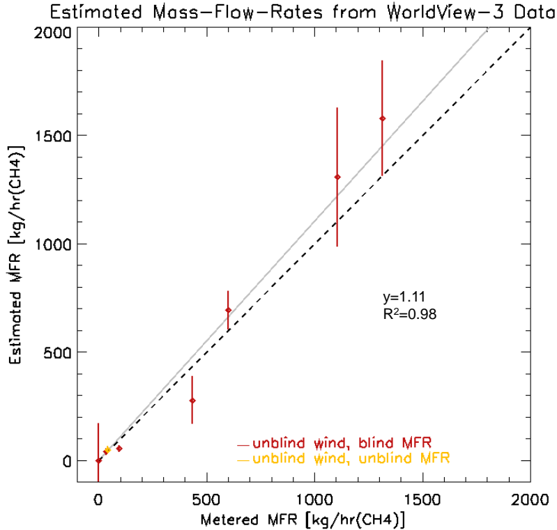
Figure 5. Quantification performance of methane emissions from WorldView-3 data. Metered MFR-rate shows good agreement with single blind and the single fully unblind MFR estimation results.
