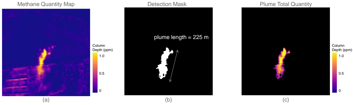
Figure 4. Contributors to MFR estimate using IME. (a) methane quantity map (CEQ=0.08 parts per million [ppm]), (b) pixels above clutter level (detection mask), (c) sum of methane quantity in detection mask.
