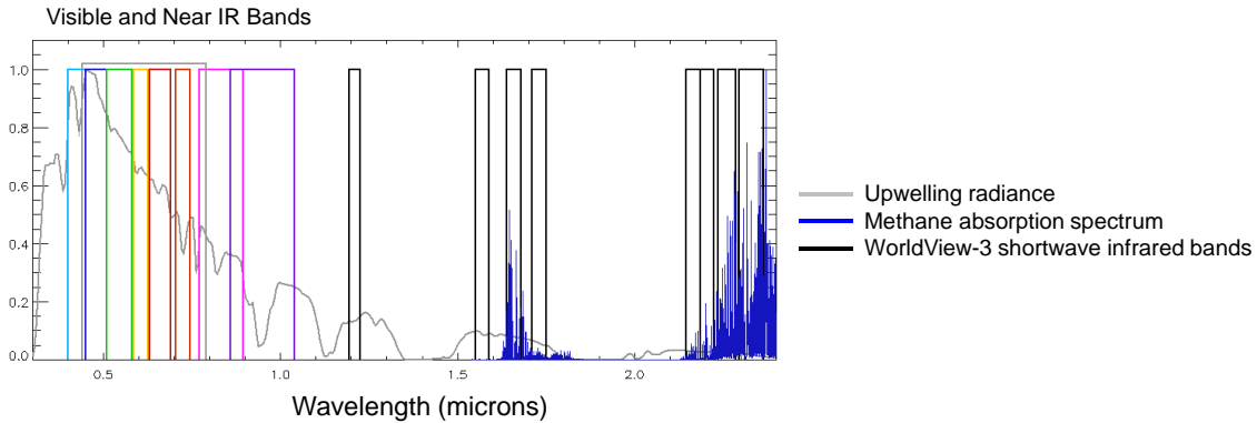
Figure 1. Wavelengths of WorldView-3 visible, near infrared (IR) and shortwave IR bands include key portions of the methane absorption spectrum. The y-axis units are arbitrary. All plots are scaled to a peak value of one.
