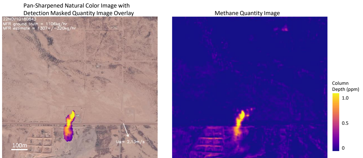
Figure 9. Methane quantity image from November 10, 2022. Ground truth MFR: 1106 kg/hr.
