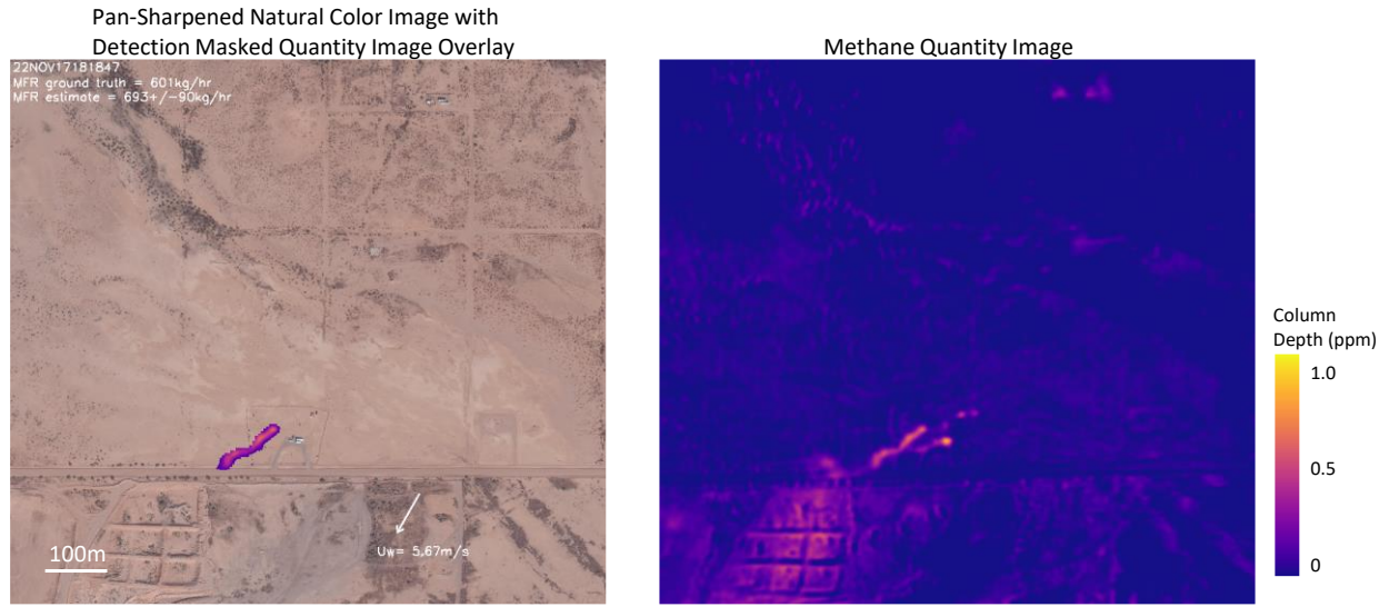
Figure 10. Methane quantity image from November 17, 2022. Ground truth MFR: 601 kg/hr.
