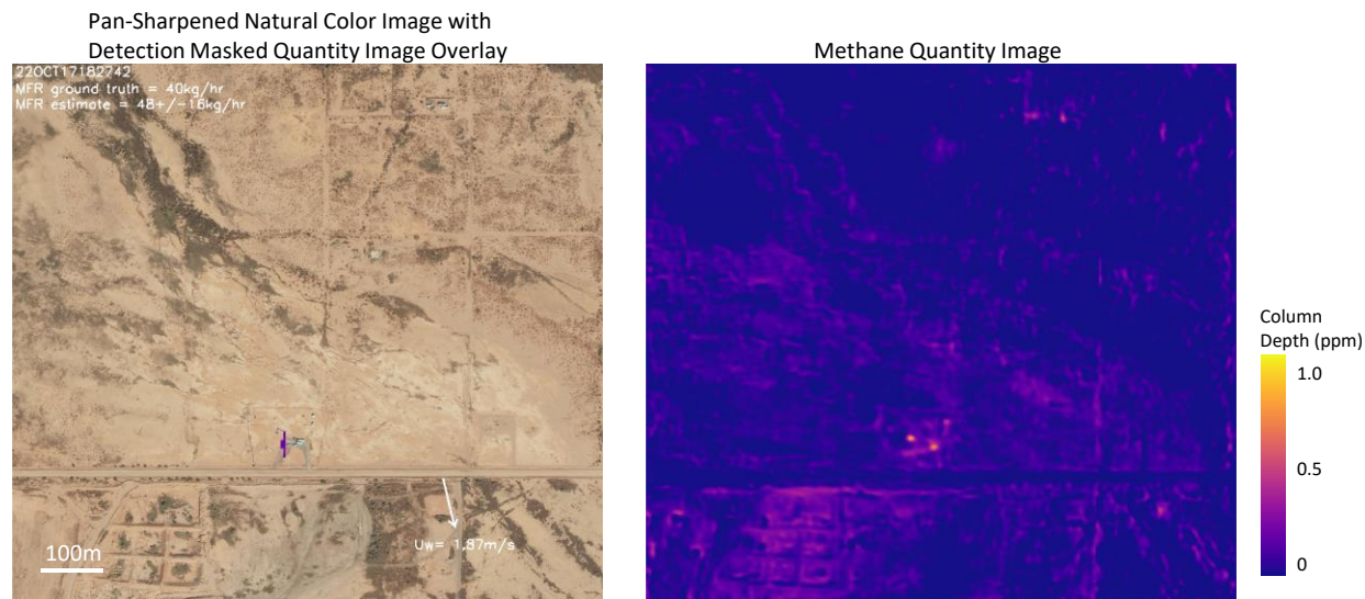
Figure 14. Methane quantity image from October 17, 2022 (post-MFR unblind). Ground truth MFR: 40 kg/hr.
