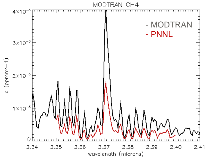
Figure 3. This comparison of the MODTRAN and the PNNL methane absorption curves reveals the factor-of-2 error.
