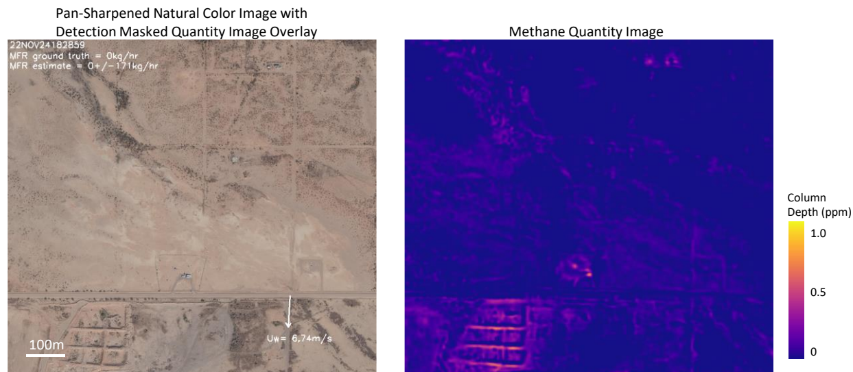
Figure 12. Methane quantity image from November 24, 2022. Ground truth MFR: 0 kg/hr.
