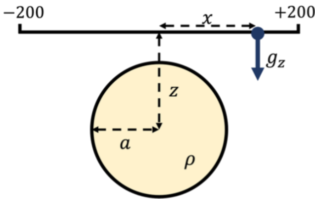
Figure 4. Setup for the synthetic gravity example.
