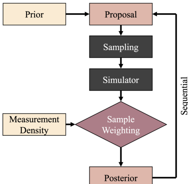
Figure 2. Workflow for the proposed SMC algorithm. The posterior is updated by training a generative probabilistic model from the proposal samples and their weights.
