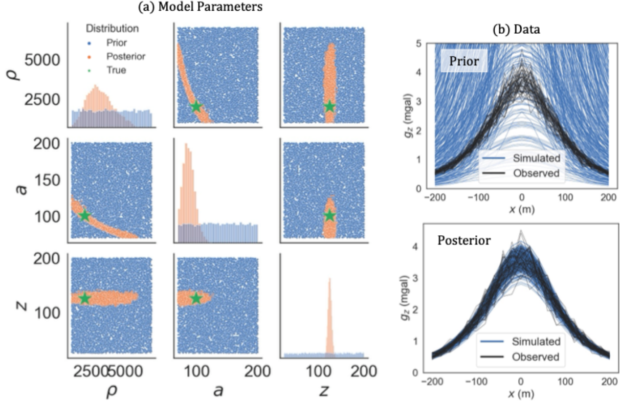
Figure 5. (a) 10,000 model parameter samples from the uniform prior distribution (blue) and data-consistent posterior distribution (orange), compared to the true value (green star) used to generate the posterior. (b) 200 samples from the pushed-forward prior (blue, top) and the pushed-forward posterior (blue, bottom) compared to the measurement distribution (black, both).
