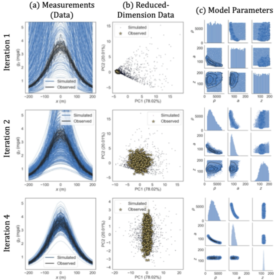
Figure 6. Three iterations of the SMC algorithm on the gravity example. (left) 1000 realizations of d from the proposal. (middle) Realizations of d after being projected into a 2D space using PCA. (right) Cross plots of proposal samples. Larger dots have larger weights. Black contours are from KDE applied to the weighted samples.
