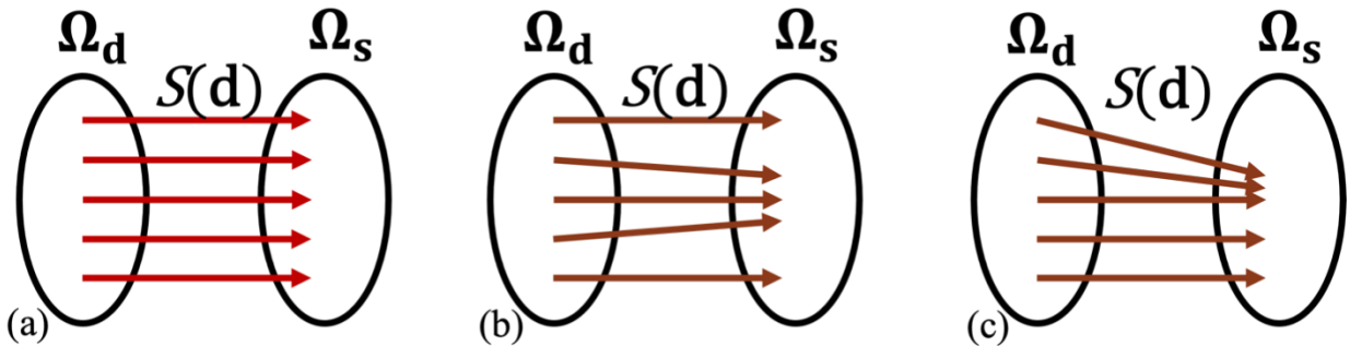
Figure 3. Conceptual diagram of how the dimension reduction function S may impact posterior information loss and bias. (a) No information loss and no bias, (b) Information loss but no bias, (c) both information loss and bias.
