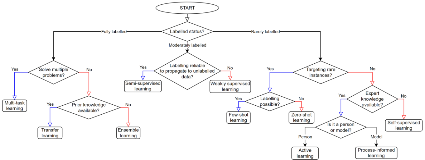
Figure 3. Practical flowchart for selecting an appropriate deep learning technique (as of May 2023) to address the small data problem in remote sensing applications.
