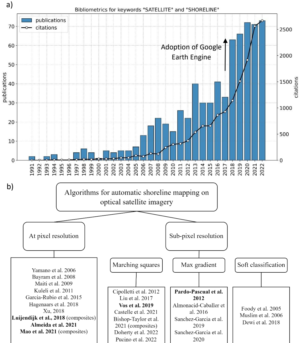
Fig. 1 | Rapid evolution of satellite-derived shoreline methods. a) Number of publications and citations per year for articles that include keywords “satellite” and “shoreline”. This was retrieved from the Web of Science database with the following query: Tl = ("satellite*" AND "shoreline*") OR AB = ("satellite*" AND "shoreline*") OR AK = ("satellite*" AND "shoreline*") , where Tl stands for Title, AB for Abstracts and AK for Author’s Keywords. b) Present methods to automatically map shorelines on optical imagery, divided into ‘at pixel resolution’ and ‘sub-pixel resolution’. This figure was adapted from 16 . The references in bold are evaluated in this study.
