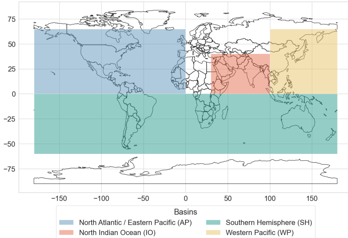
Figure 2 Tropical cyclone basins used in this research based on Meiler et al., 2022. Together the four basins represent the spatial extent of the hazard data, and thus, by extension, the population and habitat data used (i.e. the study are for this research).
