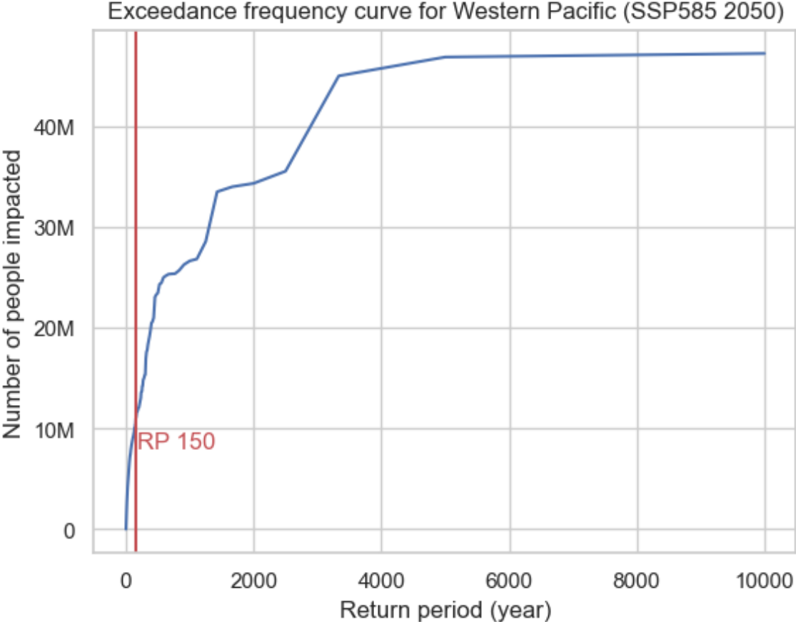
Figure 2. Exceedance frequency curve for Category 5 windspeeds in the Western Pacific basin under climate change (SSP585 2050). The red line indicates a return period of 150 years, for which the number of people impacted corresponds to 10 million.
