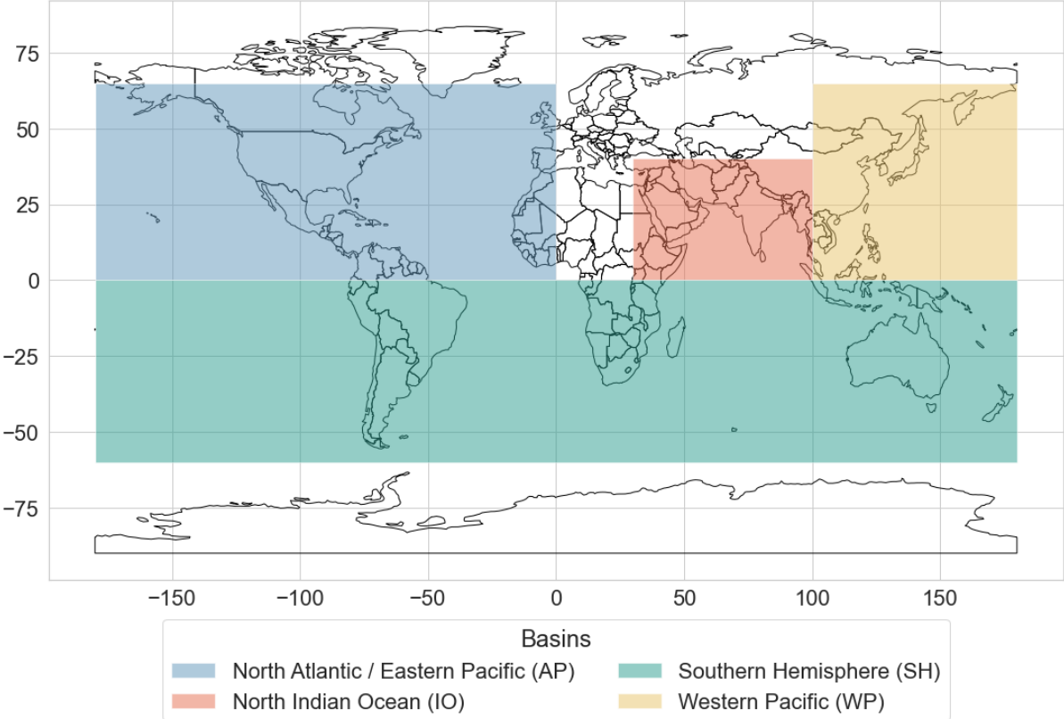
Figure 3. Tropical cyclone basins used in this research based on Meiler et al., 2022. Together the four basins represent the spatial extent of the hazard data, and thus, by extension, the population and habitat data used (i.e. the study are for this research).
