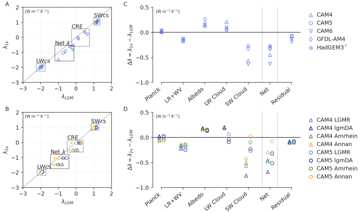
Fig. S6. Feedback decomposition of Last Glacial Maximum (LGM) and 2\times\text{CO}_2 climate feedbacks in atmospheric general circulation models (AGCMs).
