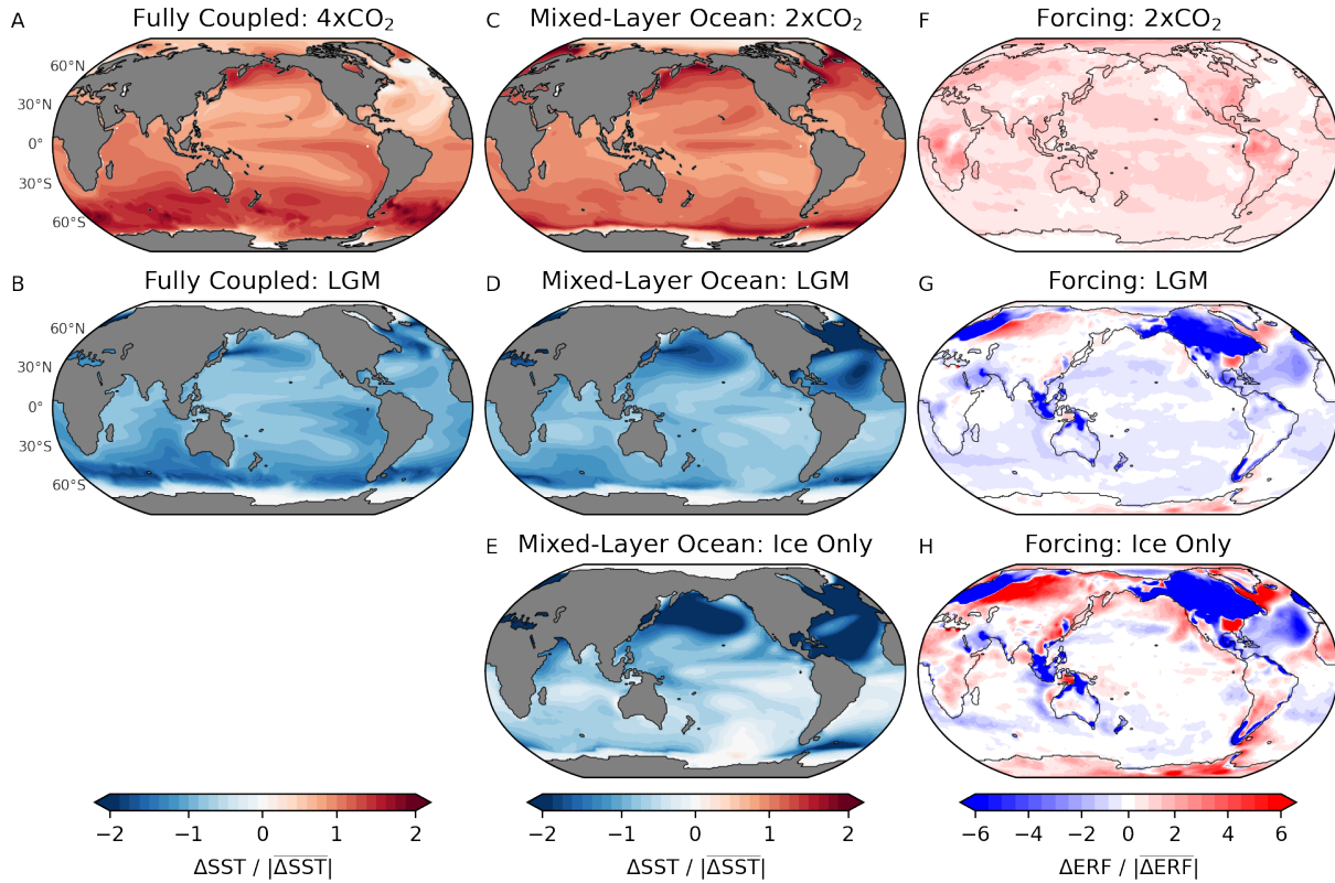
Fig. S5. Spatial patterns of sea-surface temperature (SST) response and effective radiative forcing (ERF) in CESM1-CAM5 model simulations from Zhu & Poulsen (22).
