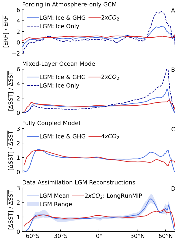
Fig. 3. Zonal-mean patterns of effective radiative forcing (ERF) and sea-surface-temperature (SST) anomalies. All anomalies are normalized through division by global-mean anomalies. (A–C) Model simulations in CESM1-CAM5 from Zhu & Poulsen (22). (A) ERF directly from three fixed-SST simulations using atmospheric general circulation model with LGM greenhouse-gas (GHG) and ice-sheet (Ice) forcing, 2xCO 2 , and LGM ice-sheet forcing alone (22) (including coastline changes). (B) Equilibrium SST patterns, corresponding to panel (A), in coupled mixed-layer ocean model. (C) Quasi-equilibrium SST patterns from fully coupled atmosphere-ocean model, comparing LGM forcings (22) with abrupt-4xCO 2 forcing (46); no long-run 2xCO 2 simulation is available. Note vertical-axis scales. (D) Mean and range of SST patterns from four data-assimilation reconstructions (3, 31–33) of the LGM compared to 2xCO 2 multi-model mean from LongRunMIP (34).
