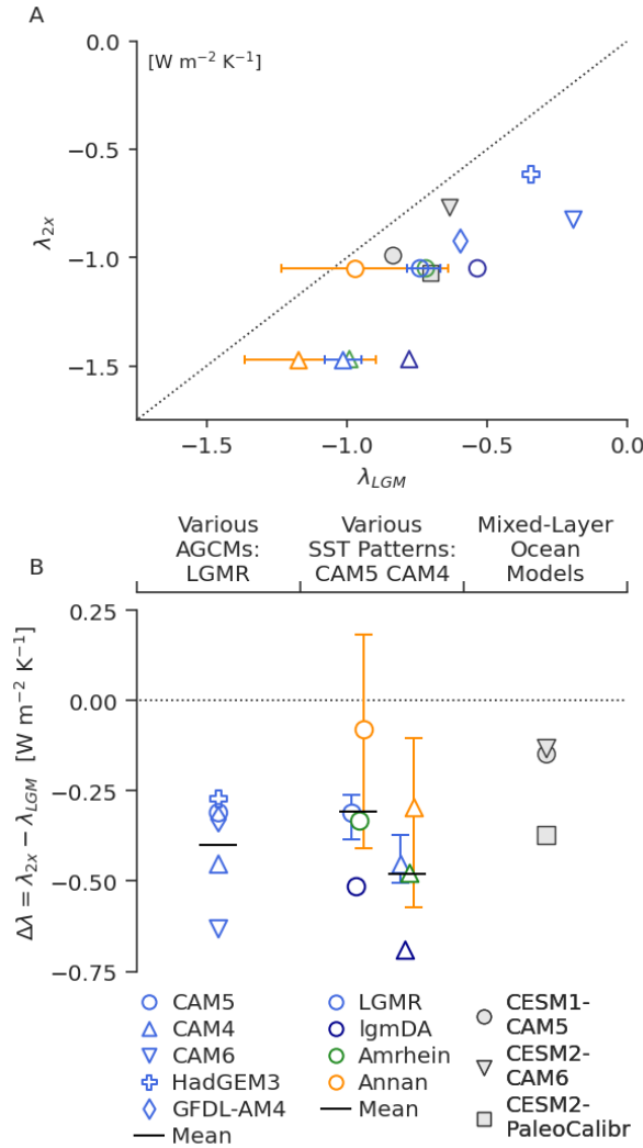
Fig. 2. Last Glacial Maximum (LGM) and 2xCO 2 climate feedbacks and LGM pattern effect ( \Delta\lambda ).
