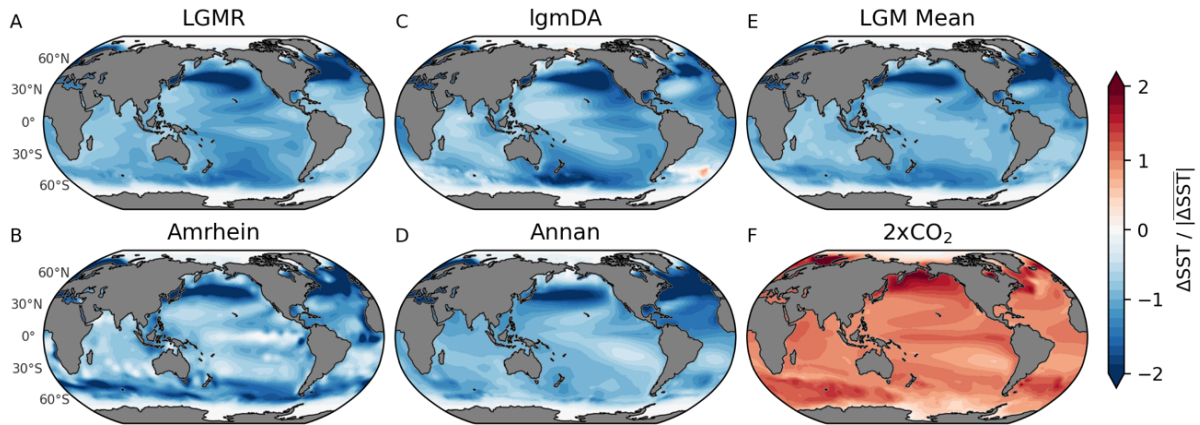
Fig. 1. Patterns of sea-surface-temperature (SST) anomalies from data assimilation at the Last Glacial Maximum (LGM) compared to modern-day doubling of CO 2 (2xCO 2 ). LGM reconstructions include (A) Last Glacial Maximum Reanalysis (LGMR) (31), (B) Amrhein (33), (C) lgmDA (3), (D) Annan (32), and (E) the mean of the four LGM patterns. (F) Pattern of the multi-model mean from near-equilibrium 2xCO 2 simulations in LongRunMIP (34), initialized from pre-industrial control. To show SST patterns, local SST anomalies are divided by absolute values of global-mean SST anomalies (consistent with feedbacks being radiative responses divided by temperature anomalies). All panels show annual means. LGM reconstructions are infilled to modern coastlines (Materials and Methods).
