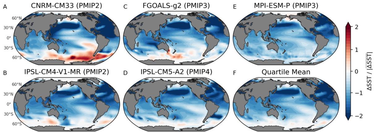
Fig. S10. Patterns of SST anomalies from Annan (32) ensemble members in quartile with strongest negative climate feedback ( \lambda ).
