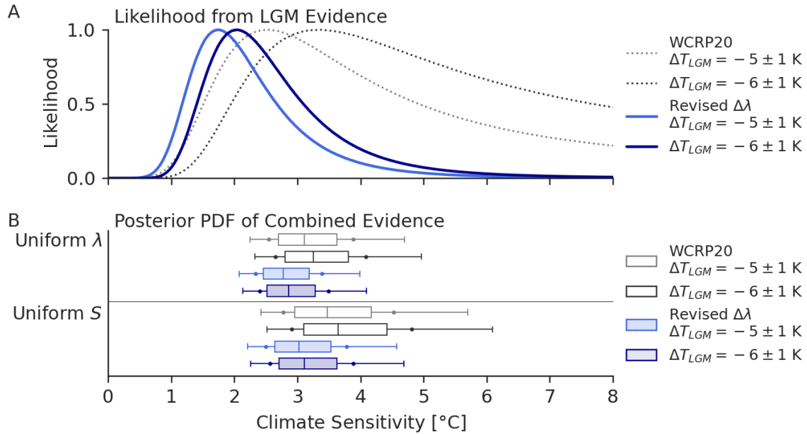
Fig. 4. Inference of modern-day climate sensitivity including the LGM pattern effect. Results from WCRP20 (1) with no LGM pattern effects and original assumption of \Delta T_{LGM} \sim N(\mu = -5, \sigma = 1) ^{\circ}C (gray) and with revised \Delta T_{LGM} \sim N(-6, 1) ^{\circ}C (black) based on IPCC AR6 (2). Revised climate sensitivity including LGM pattern effects from this study (light and dark blue) assuming \Delta\lambda \sim N(\mu = -0.37, \sigma = 0.23) Wm^{-2}K^{-1} . Climate sensitivity shown is effective sensitivity ( S ) representing 150-year response, as in WCRP20 (1). (A) Likelihood functions for S based on only the LGM line of evidence. (B) Posterior PDF after combining LGM with other lines of evidence, assuming a uniform- \lambda prior (upper panel) or a uniform- S prior (lower panel). Outlier lines indicate 5–95 th percentiles, dots indicate 66% likely range, and box indicates 25–75 th percentiles and median.
