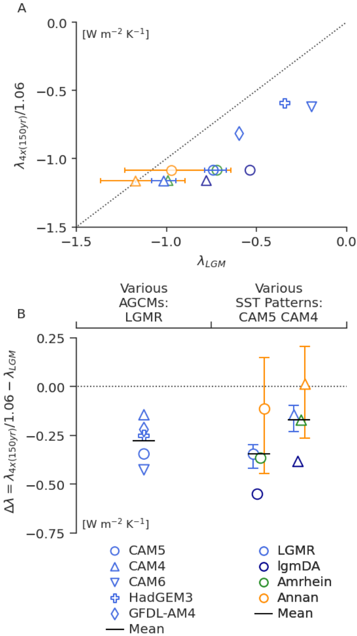
Fig. S3. LGM pattern effect ( \Delta\lambda ) based on LGM climate feedbacks in AGCMs and \text{CO}_2 climate feedbacks from 150-yr regression of abrupt- 4x\text{CO}_2 in coupled models.
