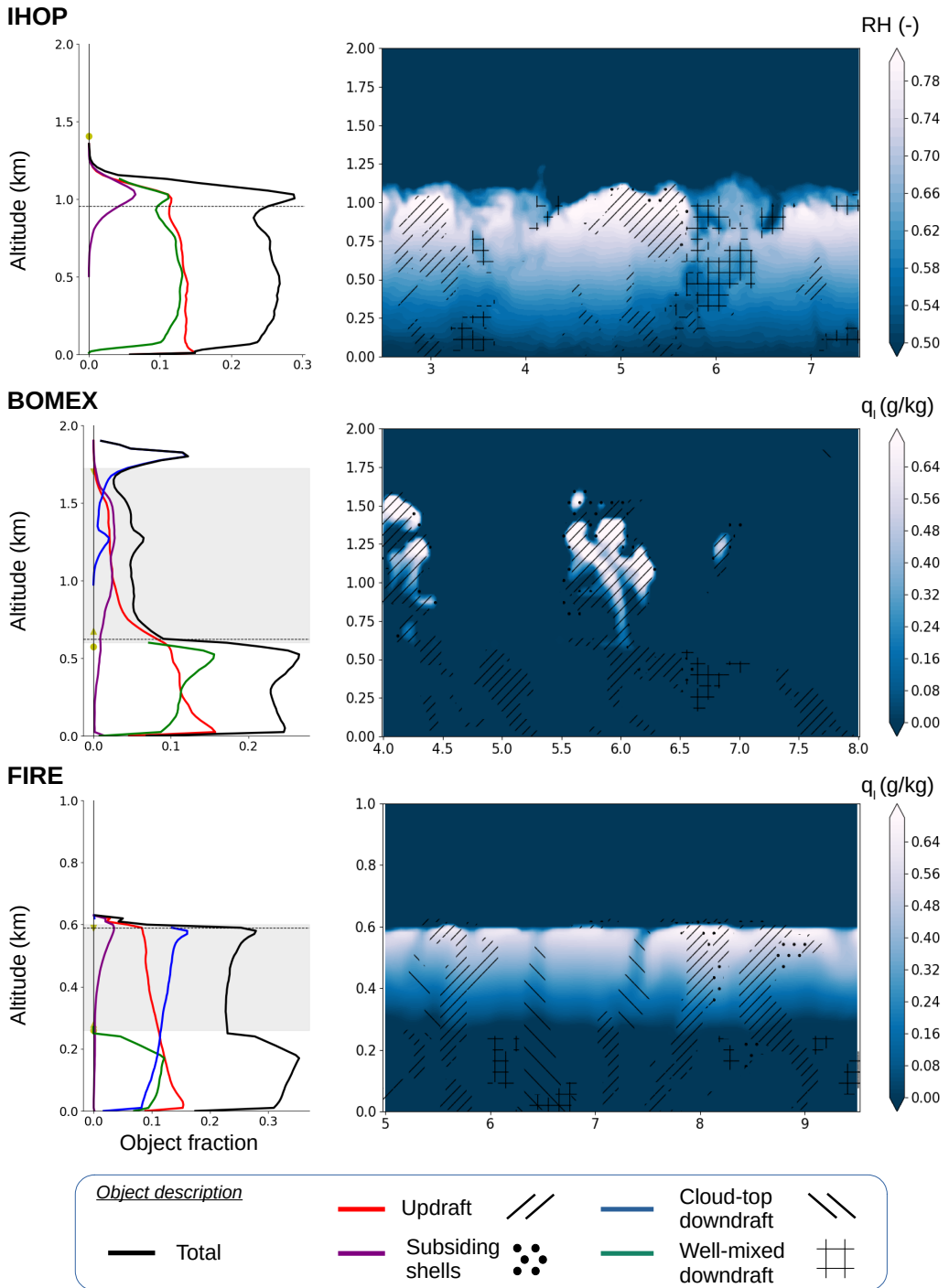
FIGURE 3 Object characteristics for the 3 boundary-layer simulations: IHOP ( t=12h ), BOMEX ( t=8h ), FIRE ( t=21h ). Left panels show the domain-mean object coverage and right panels show cross sections for relative humidity (IHOP) and liquid water content (BOMEX, FIRE) over segments shown in Figure 2. Coverage by updrafts, subsiding shells, cloud-top downdrafts and well-mixed downdrafts are represented as red (/ /), purple (· ·), blue (\ \), and green (+) colors (symbols) for the domain-mean profile (cross section). On the left panel, the circle represents the domain-mean Lifting Condensation Level (LCL), upside and downside triangles are the Level of Free Convection (LFC) and Level of Neutral Buoyancy (LNB), and the horizontal dotted line represents the well-mixed layer top z_i (see main text). The grey area represent the cloud layer.
