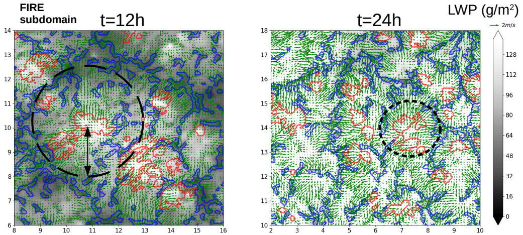
FIGURE 11 Liquid water path ( \text{g/m}^2 ) over FIRE subdomains shown in Figure 10 at t=12\text{h} (day) and t=24\text{h} (night). Updrafts and downdrafts are represented in red and blue contours respectively, and horizontal winds as green arrows for the altitude z=0.95z_i . Black circles show regions influenced by one updraft's divergence.
