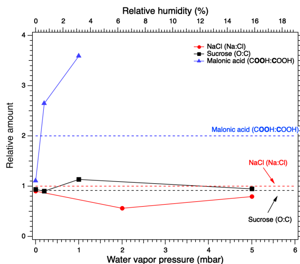
Figure 4. Relative peak areas for NaCl (Na:Cl, red circles), sucrose (O:C, black squares) and malonic acid (COOH:COOH, blue triangles). The dashed horizontal red, black and blue lines show the expected stoichiometric ratio for NaCl, sucrose and malonic acid, respectively. Relative ratios differing from the stoichiometric ratio indicate changes in the chemical composition of the surface of the aerosol.
