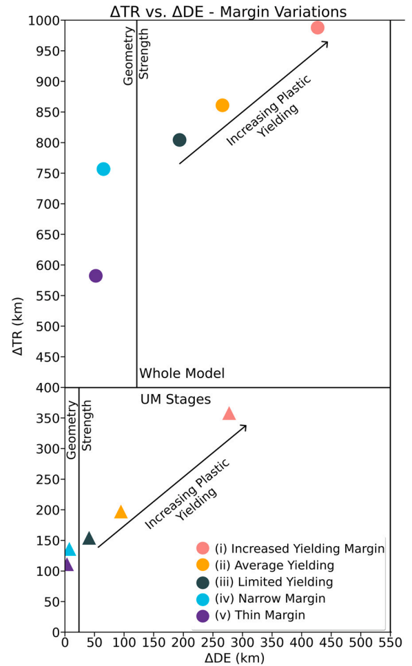
Fig. 7. Trench retreat ( \Delta TR ) vs. width of deformed area ( \Delta DE ) along the continental plate margin for margin variations for the whole model (top) and upper mantle stages (bottom).
