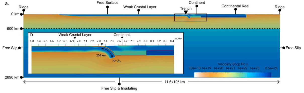
Fig. 1. a) Model set-up with a free surface top boundary condition and a continental keel with inset b), showing a zoomed-in view of the subducting and overriding plates, the weak crustal layer, and the initial condition at the start of our models for reference-keel case 4.
