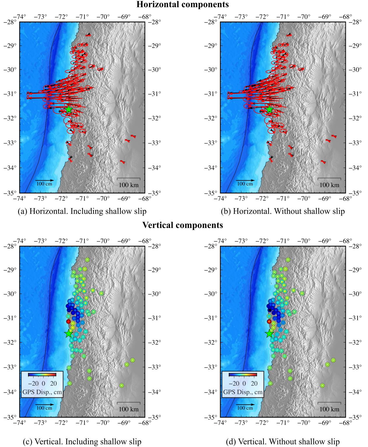
Figure A16. Comparison between models with shallow slip and imposing a zero slip at shallow depth. Observed horizontal GPS (black arrows) and predictions for the posterior mean model (red arrows) using a 2nd order approximation C_p including shallow slip (a) and without shallow slip (b). Observed vertical GPS (outer circle) and predictions for the posterior mean model (inner circle) including a shallow slip (c) and without shallow slip (d). The colormap indicates the corresponding vertical displacements.
