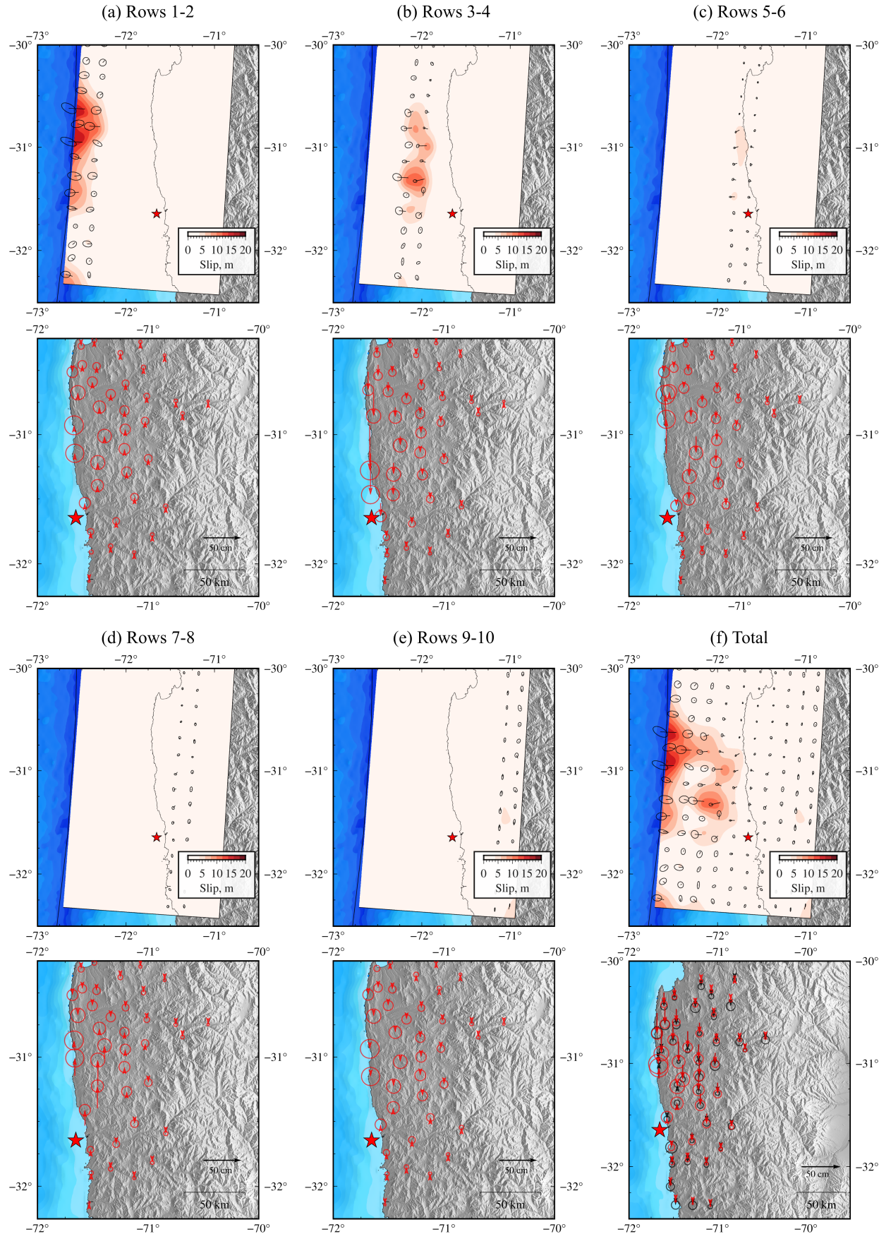
Figure A15. Vertical displacement predictions for the posterior mean model (red arrows) calculated for different subfault slips (a-e) and total displacement (f). The observed vertical GPS (black arrow) is shown in (f).
