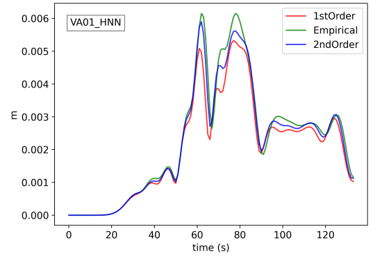
Figure 4. Covariance matrix comparison for HRGPS records (a) and Strong Motion stations (b). The green line represents the diagonal of the empirical covariance matrix (i.e., the matrix created from an ensemble of models). The red and blue line represents the diagonal of the matrix calculated using the 1st and 2nd order approximation approach.
