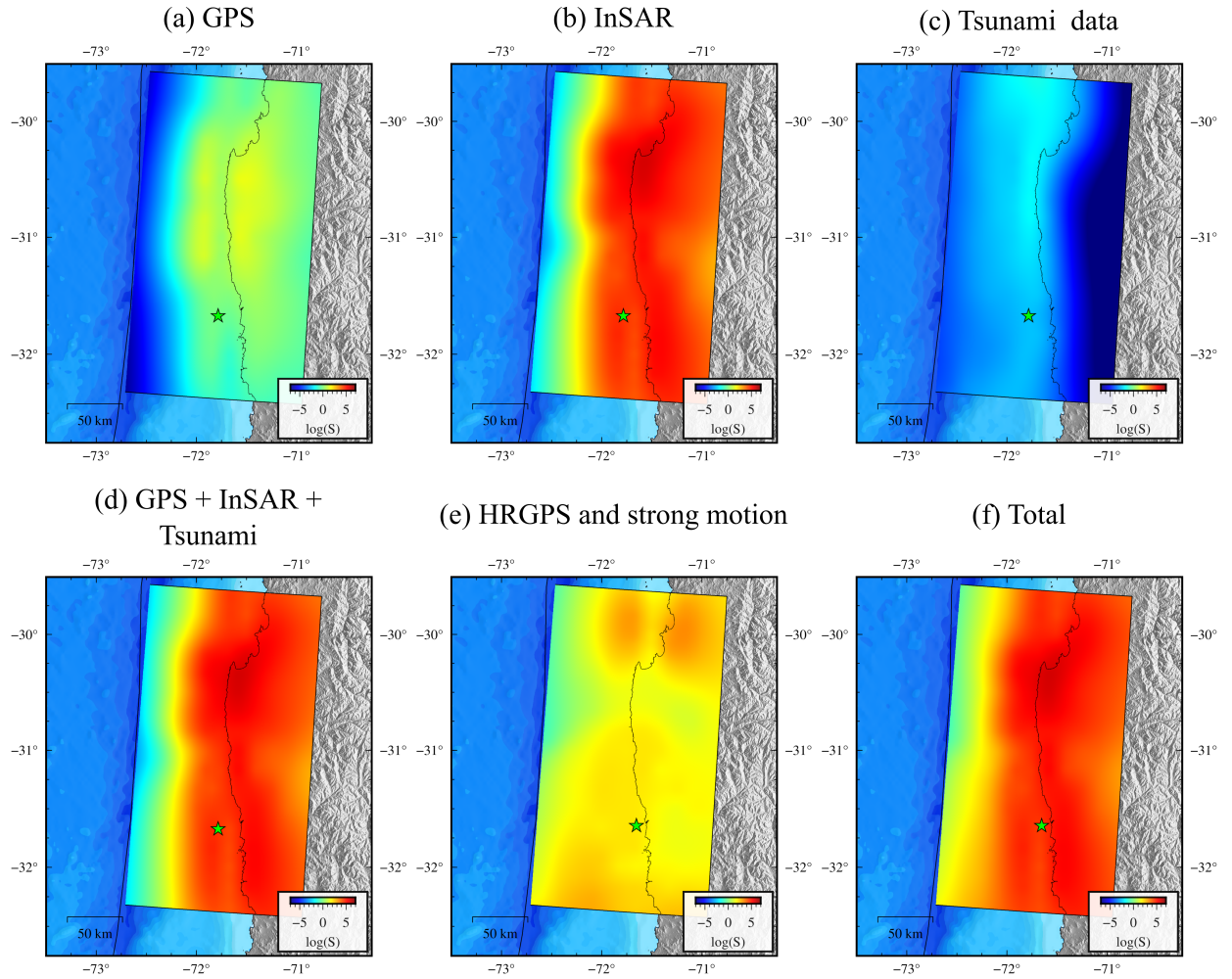
Figure A7. Sensitivity for each data set. The sensitivity is shown for (a) GPS, (b) InSAR, (c) tsunami data, (d) tsunami, InSAR, and GPS, (e) high rate GPS and strong motion, and (f) the ensemble of all data sets. /mThe sensitivity corresponds to a theoretical response given a one meter slip in each sub-fault.
