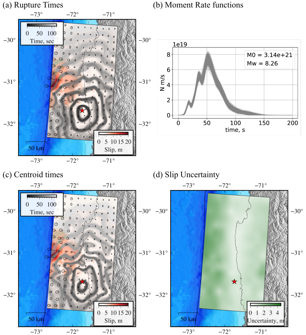
Figure A11. Impact of using a 1st order approximation C_p in slip inversion. (a) Posterior mean coseismic slip model, arrows represent the slip directions and the ellipses their uncertainties. Contours show stochastic rupture fronts samples from the a posteriori distribution every 10 seconds. (b) Stochastic moment rate functions. (c) Posterior mean coseismic slip model with contours that represent stochastic centroid time fronts samples from the a posteriori distribution. (d) Uncertainty of the ensemble of coseismic slip models. The red star in the figures represents the inverted hypocenter location.
