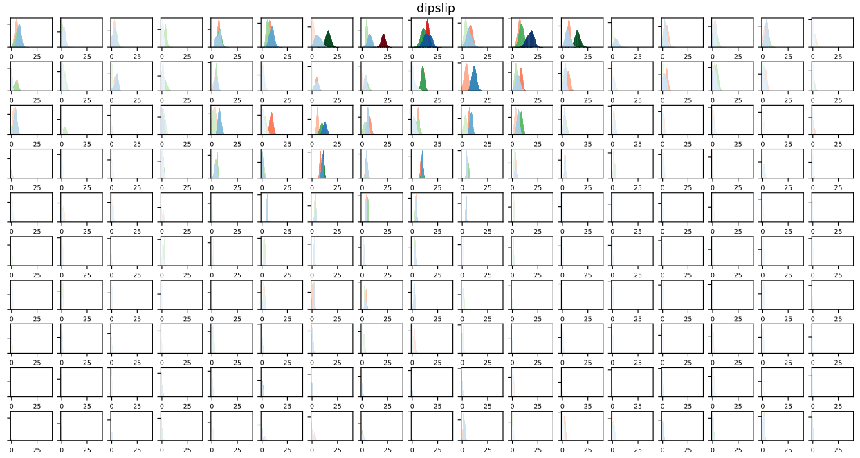
Figure A8. Posterior mean distributions for the dip slip parameters for various covariance matrices. The colors indicate which covariance matrix is used: the empirical C_p matrix (green), the first order approximation matrix (red), and the second order approximation matrix (blue). The strength of the colors are proportional to the magnitude of the slip.
