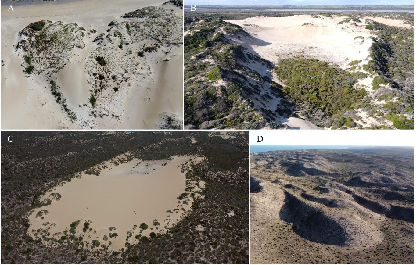
Figure 11: A: Blowout at Maurpetuis Bay, Kangaroo Island, South Australia. B: Parabolic dune near Cantara, Youngusband Peninsula, South Australia. C: Long-walled parabolic dune near Port Lincoln, South Australia. D: Nested, long-walled parabolic dunes at Snake lagoon, Kangaroo island, South Australia. Credits: P. Hesp.
