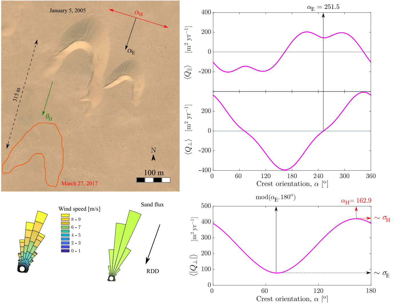
Figure 17: Barchan dune on a starved bed in Western Sahara in Morocco ( 27.5^\circ\text{N} , 13.1^\circ\text{W} ). The red contour shows location of the main barchan 12 years after the snapshot was taken. See caption of fig. 12 for an explanation of parameters and plots.
