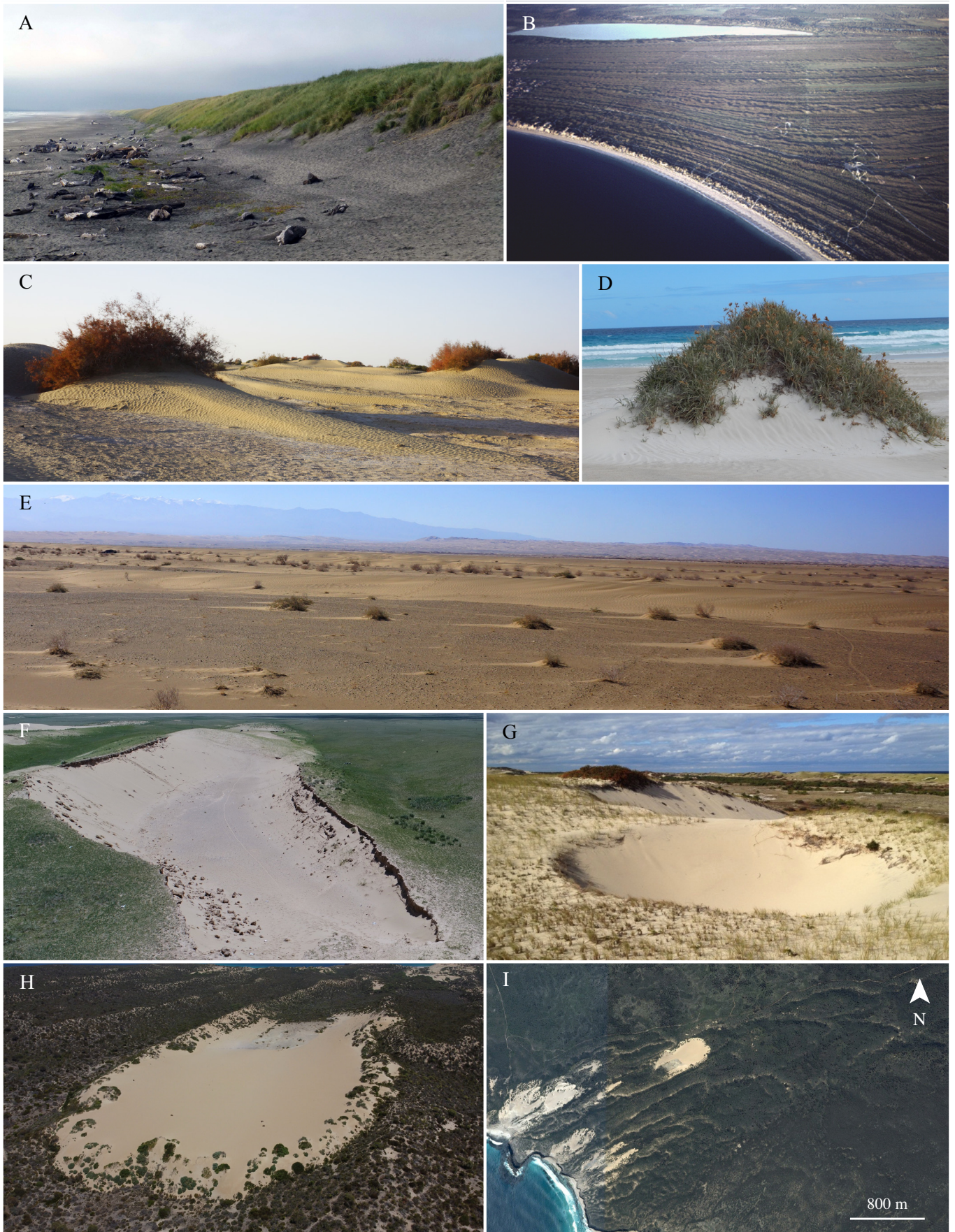
Figure 4: Dunes associated with vegetation. A: Fore-dune at Fort Steven, Oregon ( 46.182^{\circ}\text{N} , 123.982^{\circ}\text{W} ). B: Fore-dune plain comprising multiple foredunes formed by coastal progradation. C-E: Nebkhas. F: Trough blowout 12 m deep and 600 m long on the Tibet plateau ( 35.992^{\circ}\text{N} , 100.415^{\circ}\text{E} ). G: Bowl blowout 3 m deep at Cape Cod ( 42.075^{\circ}\text{N} , 70.189^{\circ}\text{W} ). H & I: Parabolic dune in south Australia ( 34.912^{\circ}\text{S} , 135.89^{\circ}\text{E} ) in 9/2016 (I). Credits: C. Bristow (A), P. Hesp (B, D, F, G, H), C. Narteau (C, E), CNES/Airbus (I).
