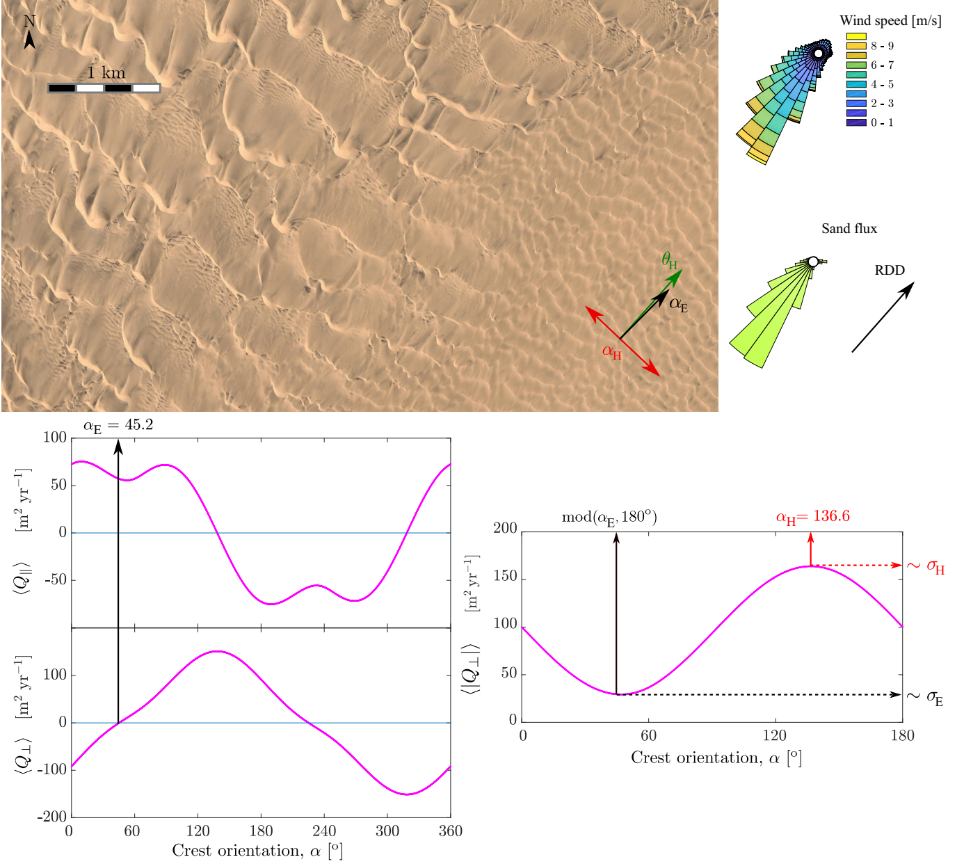
Figure 12: Transverse long-crested dunes on sand-covered bed in the Moçâmedes desert in Angola (16.6°S, 11.9°E). Roses, which point upwind, show the wind regime and the corresponding sand flux regime from 2010 to 2020. See Sections 5.2 and 7 for an explanation of parameters and details of calculations. Graphics show the calculated characteristic sand flux components \langle Q_{\perp} \rangle , \langle Q_{\parallel} \rangle and \langle |Q_{\perp}| \rangle over a dune with orientation \alpha . Angles are measured relative to east direction. \alpha_I , the dune orientation that maximizes \langle |Q_{\perp}| \rangle , \alpha_E , the dune direction for elongation ( \langle Q_{\parallel} \rangle > 0 ) without migration ( \langle Q_{\perp} \rangle = 0 ), and \theta_I , the direction of the sand flux over a dune of orientation \alpha_I , are shown by arrows in the image.
