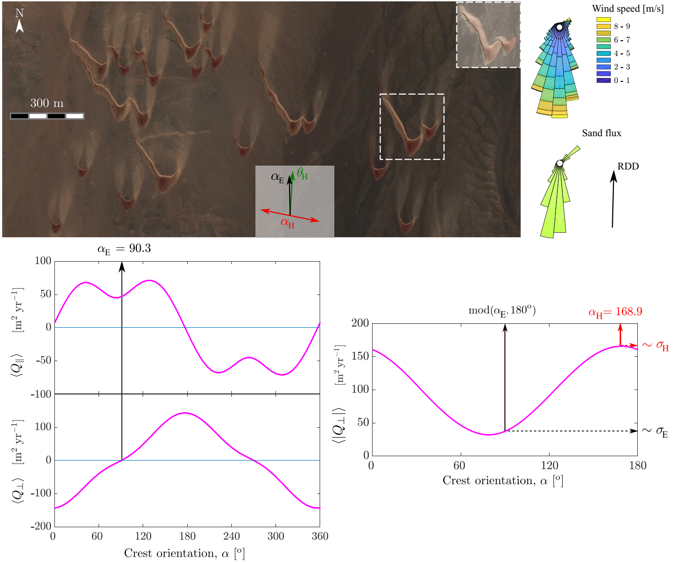
Figure 18: Asymmetric barchan dune with an elongated horn on a starved bed on the Skeleton coast in Namibia (20.1°S, 13.3°E). The inset shows the dunes in the white dashed box after a secondary wind event. See caption of fig. 12 for an explanation of parameters and plots.
