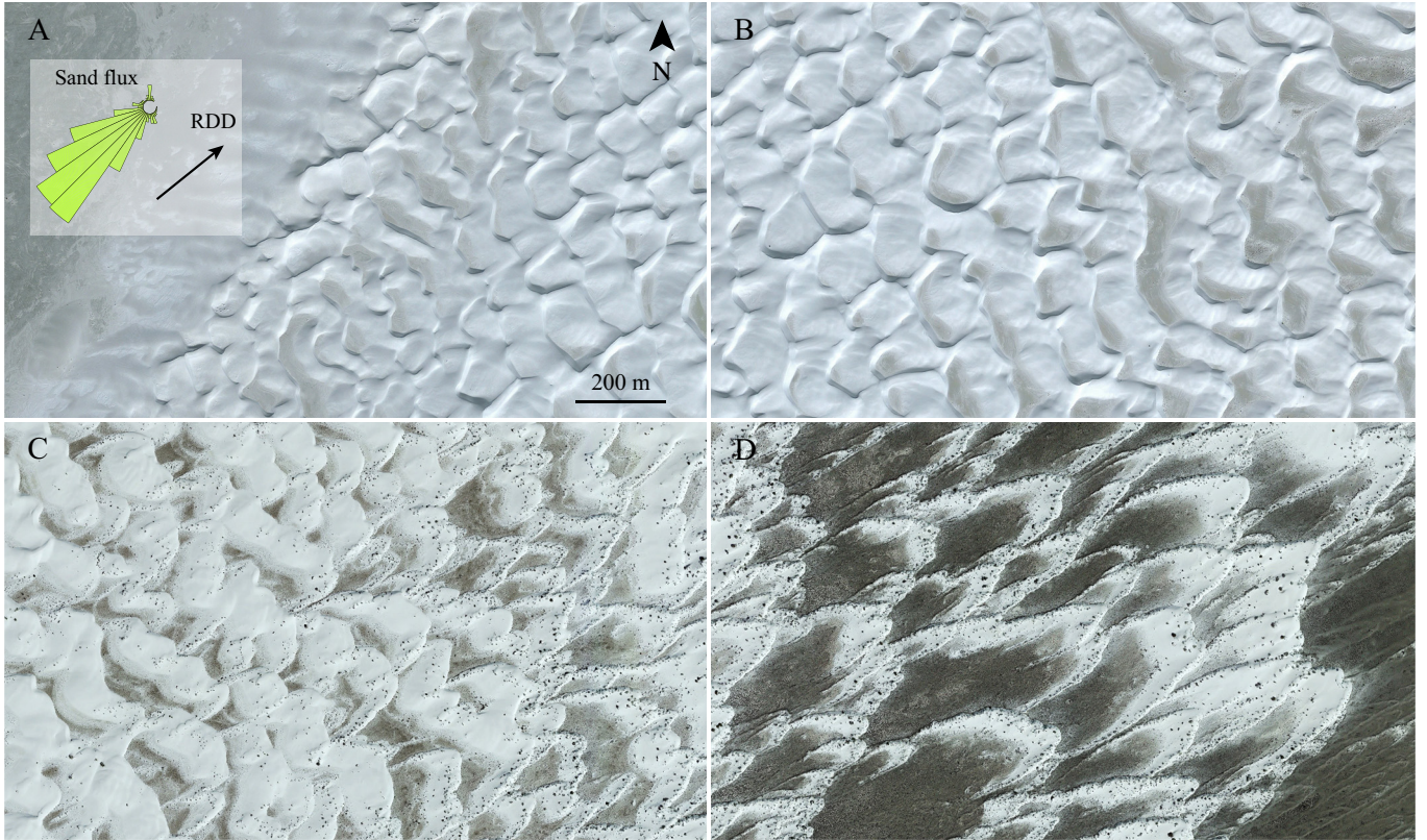
Figure 10: A west-to-east along-RDD ( 30^\circ\text{N} of East) evolutionary sequence across the White Sands dunefield starting at ( 32.802^\circ\text{N} , 106.302^\circ\text{W} ) and ending at ( 32.848^\circ\text{N} , 106.204^\circ\text{W} ), which corresponds to a distance of approximately 11 km. Sand sheets and proto dunes (A) evolve into transverse barchanoid ridges (B) and downwind into parabolic dunes (D). Scale is the same for all snapshots. Sand flux rose points upwind. See Section 7 for details of calculations. After the publication [105], we used a density \rho_s = 2300 \text{ kg}\cdot\text{m}^{-3} and a grain diameter d = 670 \mu\text{m} in the calculations for this particular case. Credit: Maxar Technologies.
