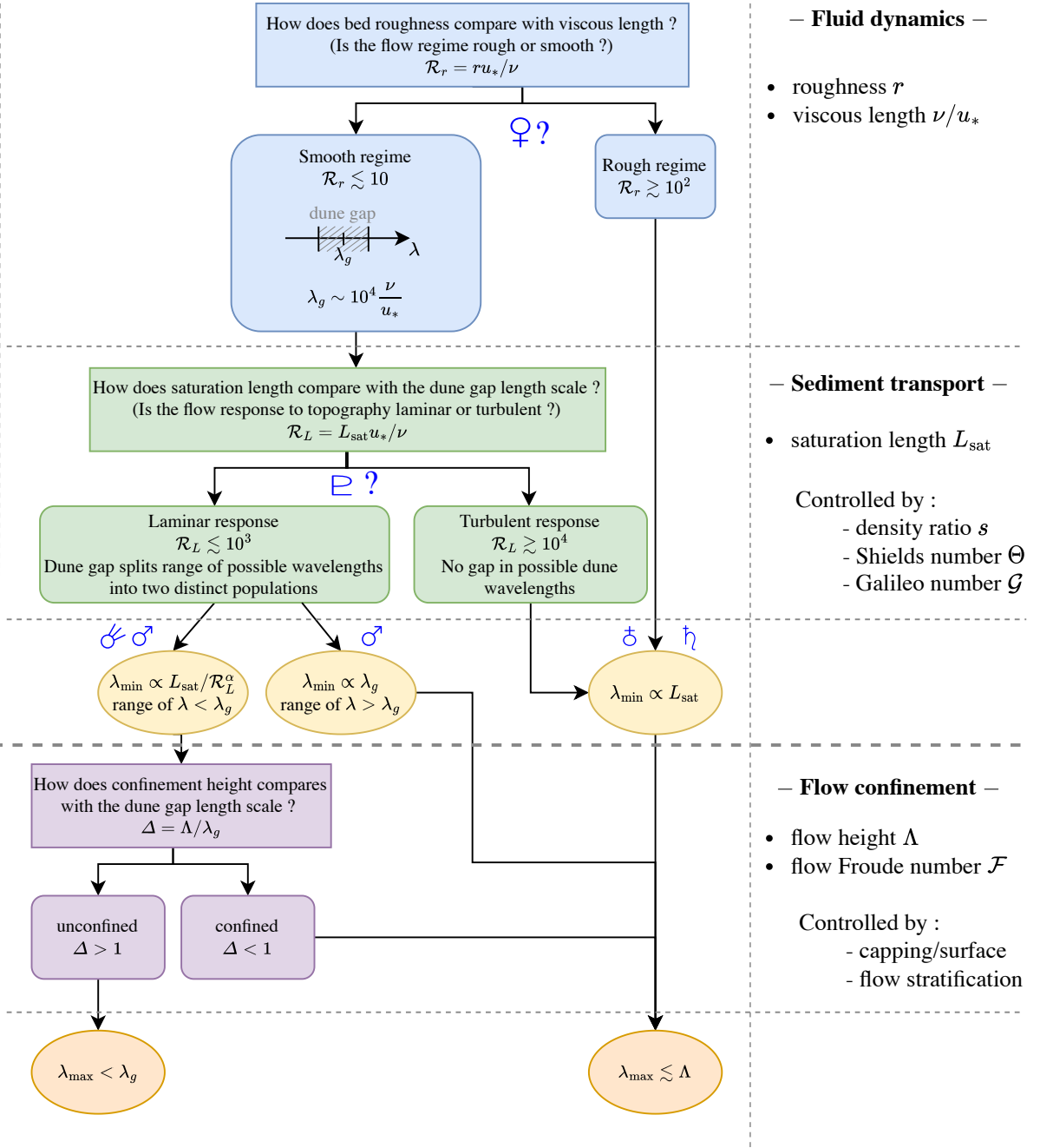
Figure 8: Identification tree for dune classification based on fluid mechanics and sediment transport. Notations: roughness length scale r , shear velocity u_* , fluid kinematic viscosity \nu , fluid to particle density ratio s = \rho_f/\rho_p ; Shields number \Theta = u_*^2/[(s-1)gd] where g is the gravitational acceleration and d is the grain size, Galileo number \mathcal{G} = \sqrt{(s-1)gd^3}/\nu . Several Froude numbers can be associated with flow confinement or stratification, e.g. \mathcal{F} = U/\sqrt{g\Lambda\Delta\rho_f/\rho_f} where U is the flow velocity and \Delta\rho_f is the fluid density jump, both evaluated at altitude \Lambda . Blue symbols: astronomical representations of planetary bodies ( \text{♀} Venus, \text{♁} Earth, \text{♂} Mars, \text{♃} Titan, \text{♇} Pluto, \text{☄} comets (e.g., 67P/Churyumov-Gerasimenko)).
