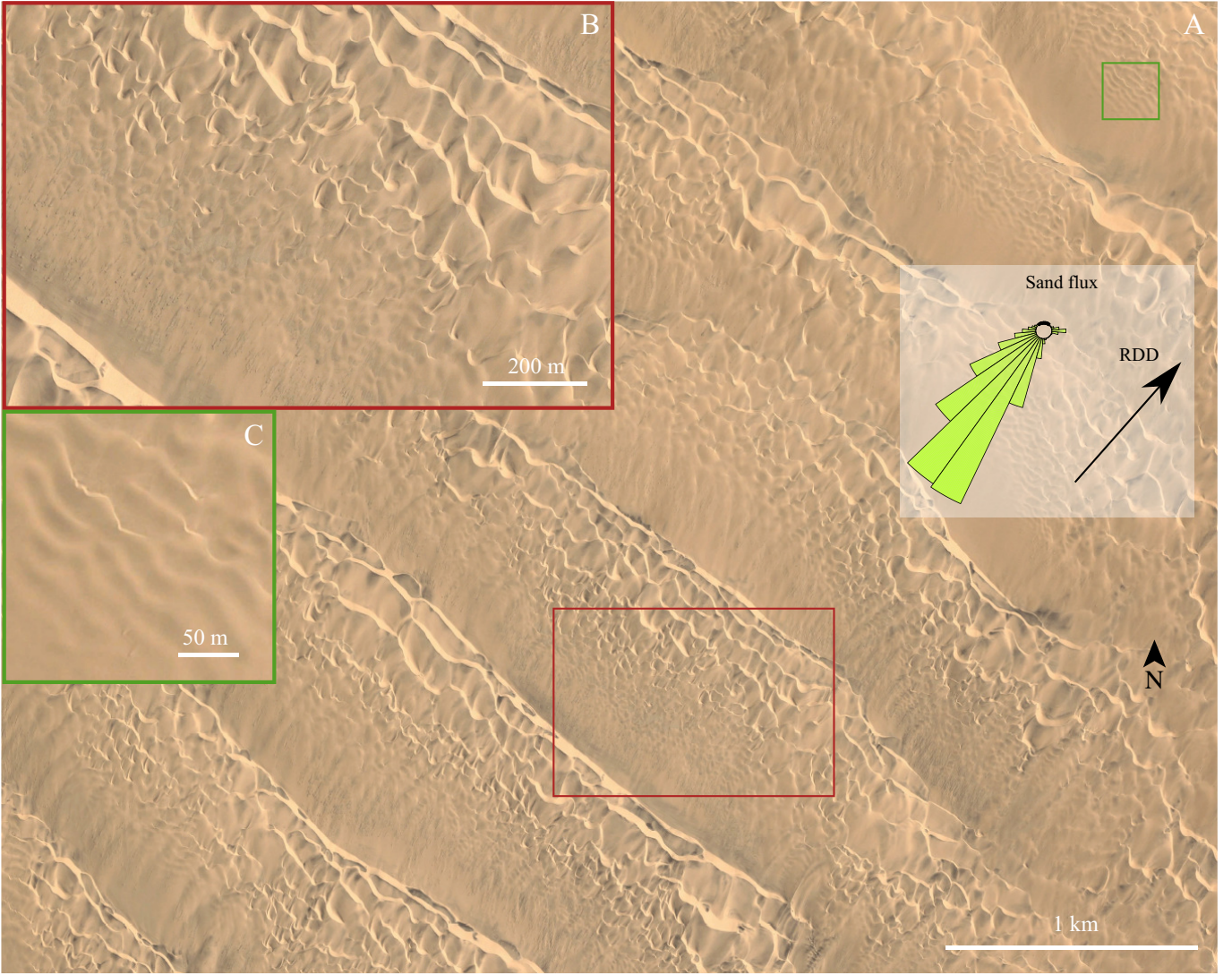
Figure 21: Illustration of the rough case with terrestrial dunes ( \mathcal{R}_r \simeq 80 ). Photographs of a coastal dune field in southwest Angola (16.4°S, 11.9°E). The parameters for calculating the sand flux distribution from wind data are the same as in Figures 12-20 (Section 7). The spokes point upwind. Local winds are approximately unidirectional (see flux rose), and the dunes, with fairly straight crests perpendicular to the resultant drift direction (RDD), can be denominated as ‘linear transverse’. Sand availability is high (no cohesive interdune). The dunes form at the elementary scale \lambda_{\min} \simeq 20 m (panel c, green frame), interact and coarsen in the course of their migration downwind (panel b, red frame) and the large-scale dune pattern has a wavelength \lambda_{\max} \simeq 850 m (panel a). Credit: Maxar Technologie (2022).
