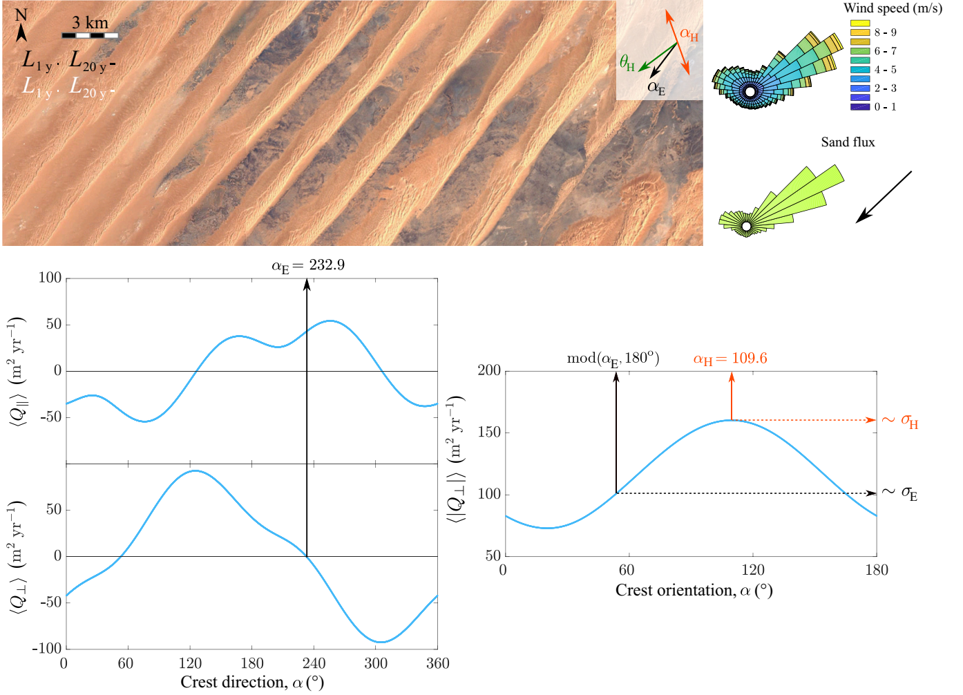
Figure 16: Periodic longitudinal linear dunes with partially starved interdune area in the Chech desert in Mali (24.3°N, 4.3°W), date: 12/2015, credit: Landsat / Copernicus. See caption of Figure 12 and 15 for an explanation of parameters and plots.
