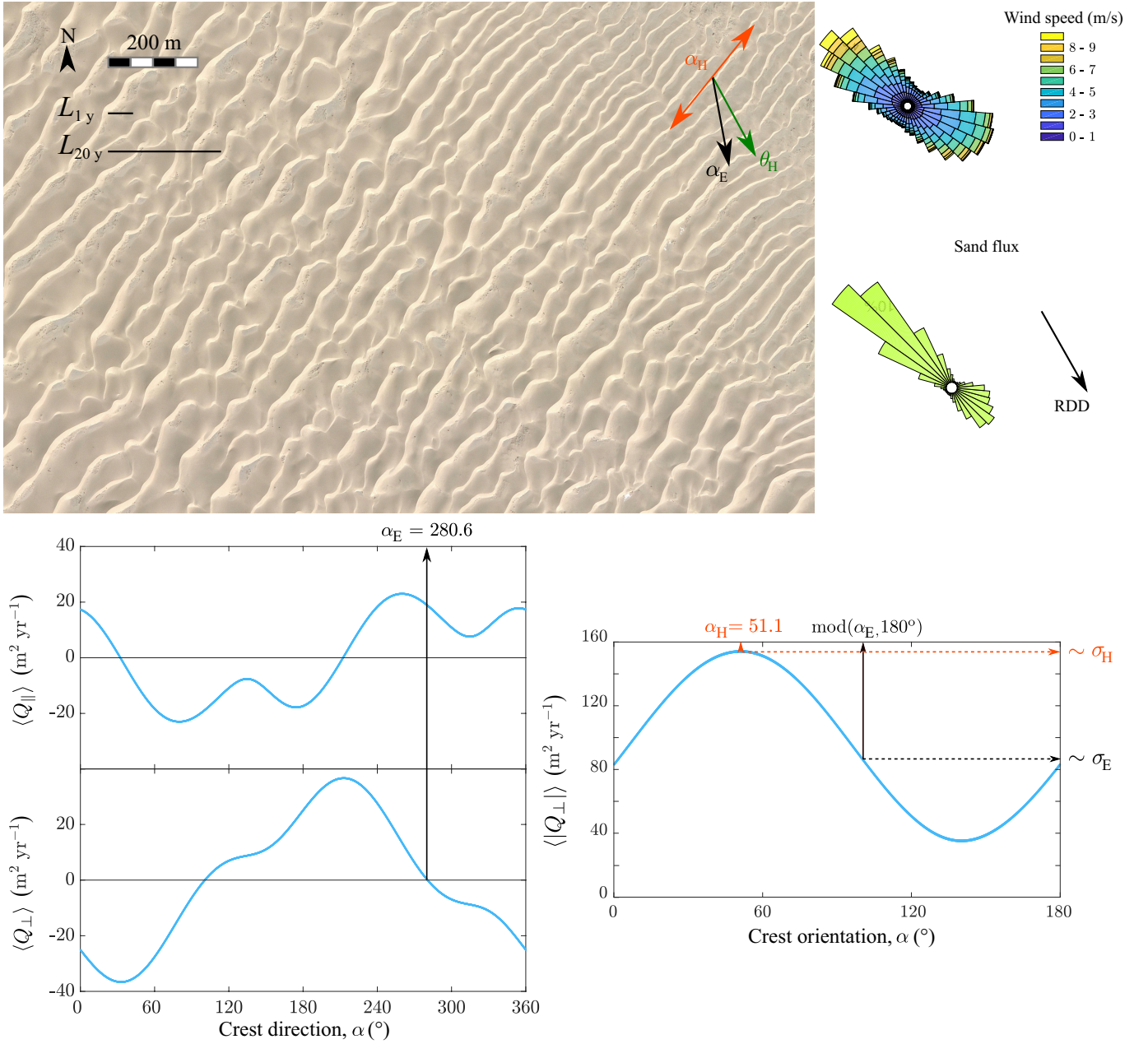
Figure 13: Oblique long-crested dunes in the Tengger desert in China (37.7°N, 105.1°E), date: 03/2009, credit: Maxar Technologies. See caption of Figure 12 for an explanation of parameters and plots.
