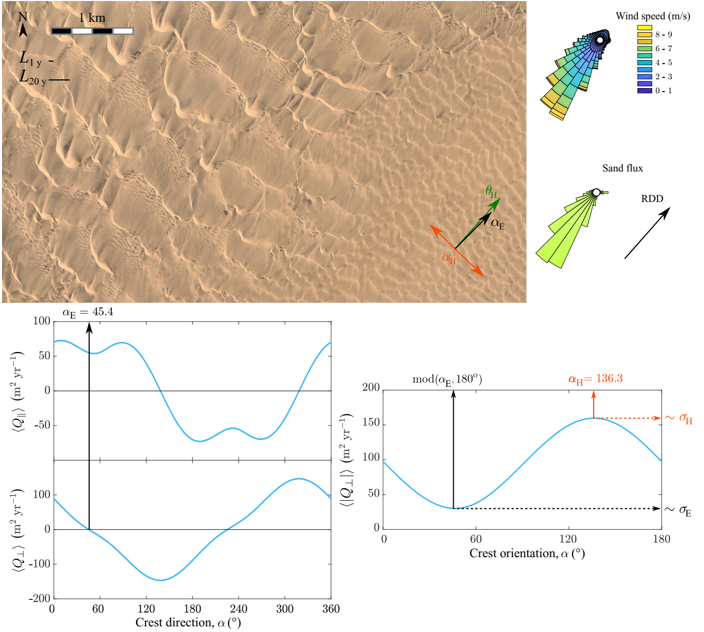
Figure 12: Transverse long-crested dunes on sand-covered bed in the Moçâmedes desert in Angola (16.6°S, 11.9°E), date: 03/2004, credit: Maxar Technologies. Roses, which point upwind, show the wind regime at 10 m above ground level and the corresponding sand flux regime from 2000 to 2020. See Sections 5.2 and 7 for an explanation of parameters and details of calculations. Graphics show the calculated characteristic sand flux components \langle Q_{\perp} \rangle , \langle Q_{\parallel} \rangle , and \langle |Q_{\perp}| \rangle over a dune with direction \alpha . Angles are measured relatively to east direction. \alpha_H , the dune orientation that maximizes \langle |Q_{\perp}| \rangle , \alpha_E , the dune direction for elongation ( \langle Q_{\parallel} \rangle > 0 ) without migration ( \langle Q_{\perp} \rangle = 0 ), and \theta_H , the direction of the sand flux over a dune of orientation \alpha_H , are shown by arrows in the image. The characteristic lengths L_{1yr} and L_{20yr} are shown to scale for comparison with cross-sectional lengths of dunes.
