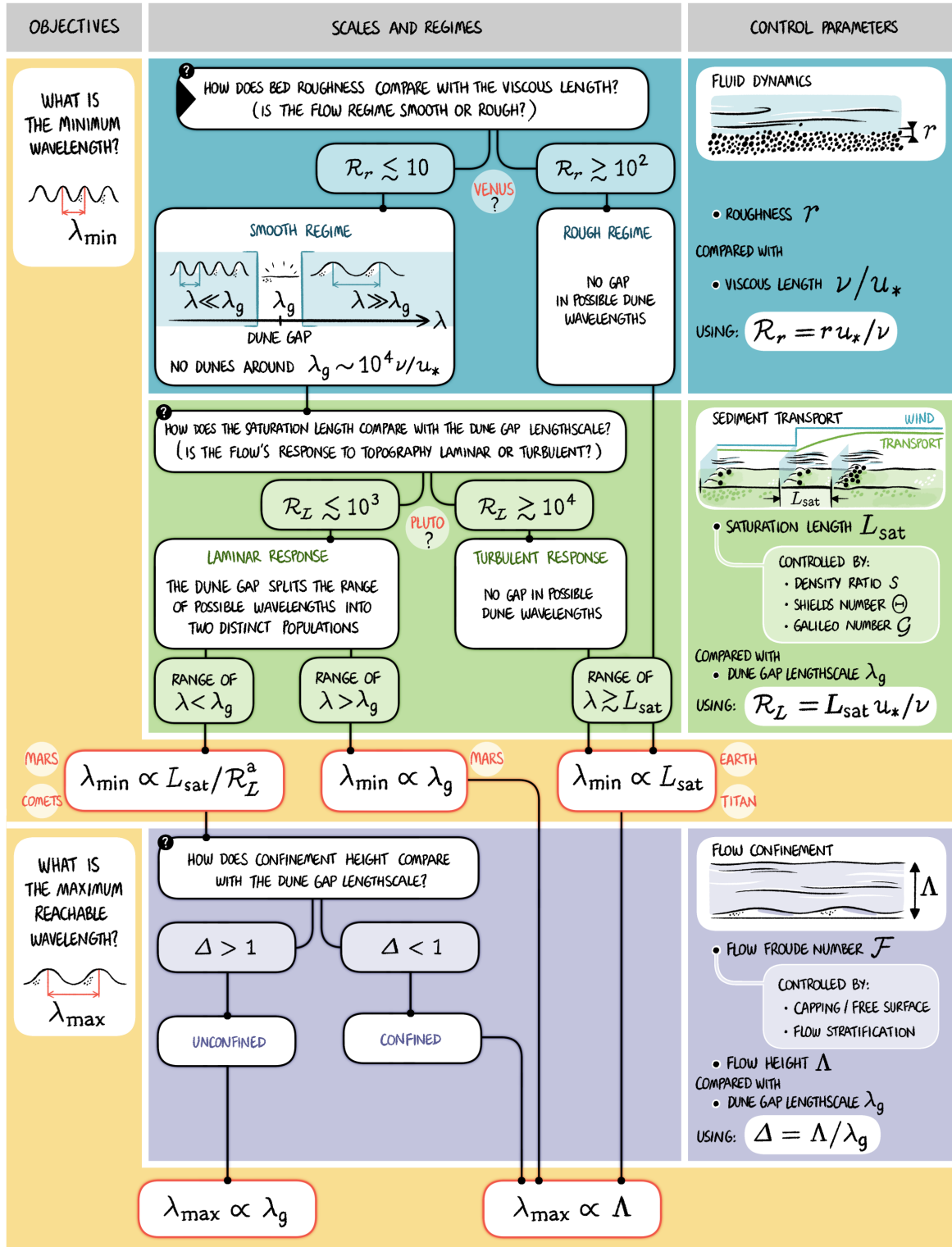
Figure 8: Identification tree for dune classification based on fluid mechanics and sediment transport. Notations: roughness length scale, r , shear velocity, u_* , fluid kinematic viscosity, \nu , fluid to particle density ratio, s = \rho_f / \rho_p ; Shields number, \Theta = u_*^2 / [(s-1)gd] , where g is the gravitational acceleration and d is the grain size, Galileo number, \mathcal{G} = \sqrt{(s-1)gd^3} / \nu . Several Froude numbers can be associated with flow confinement or stratification, e.g., \mathcal{F} = U / \sqrt{g\Lambda\Delta\rho_f/\rho_f} where U is the flow velocity and \Delta\rho_f is the fluid density jump, both evaluated at altitude \Lambda . We also show the regimes and scales expected in the different environments of planetary bodies and comets (e.g., 67P/Churyumov-Gerasimenko).
