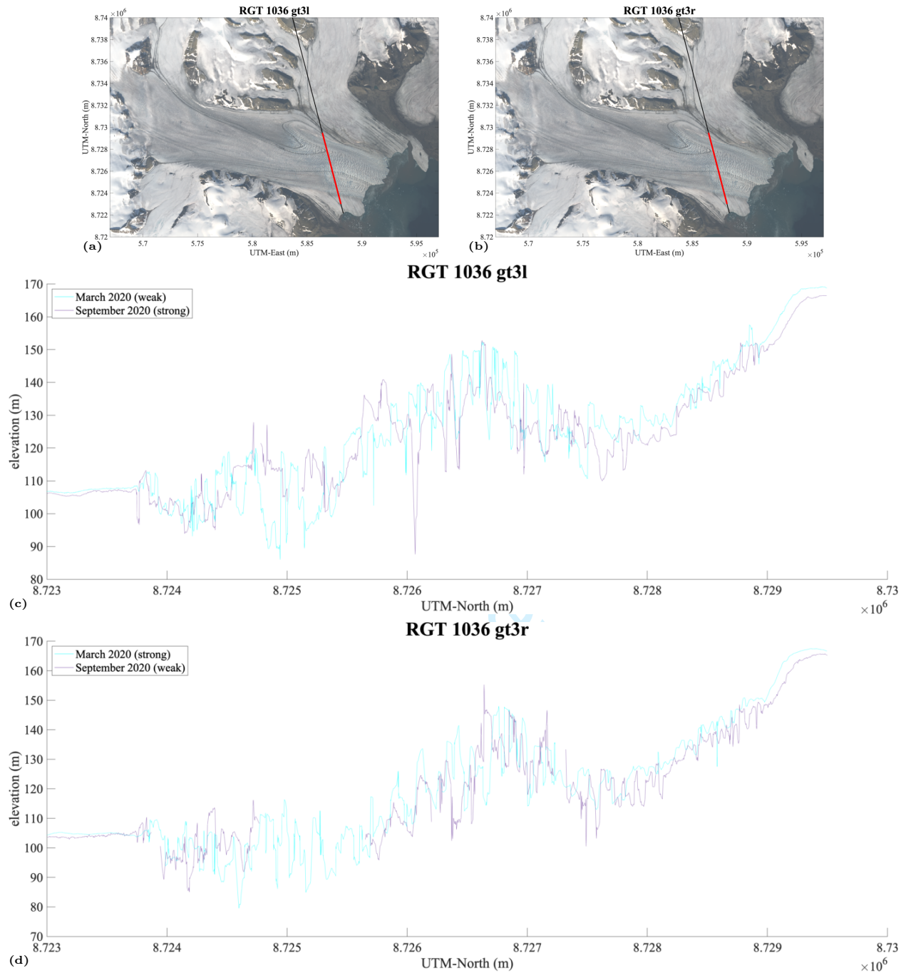
Figure 22: ICESat-2/DDA-ice surface height time series for RGT 1036 beam pair 3 over Negribreen, 2019-2020. (a) Location of RGT 1036 gt3l segment over Negribreen, (b) Location of RGT 1036 gt3r segment over Negribreen, (c) surface height time series of RGT 1036 gt3l, and (d) surface height time series of RGT 1036 gt3r.
