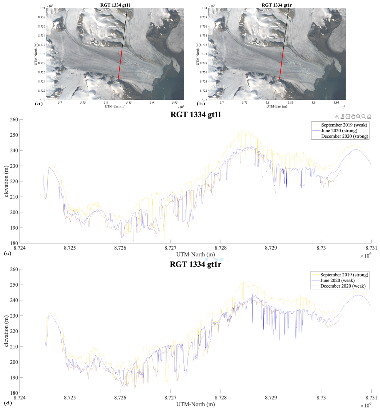
Figure 23: ICESat-2/DDA-ice surface height time series for RGT 1334 beam pair 1 over Negribreen, 2019-2020. (a) Location of RGT 1334 gt1l segment over Negribreen, (b) Location of RGT 1334 gt1r segment over Negribreen, (c) surface height time series of RGT 1334 gt1l, and (d) surface height time series of RGT 1334 gt1r.
