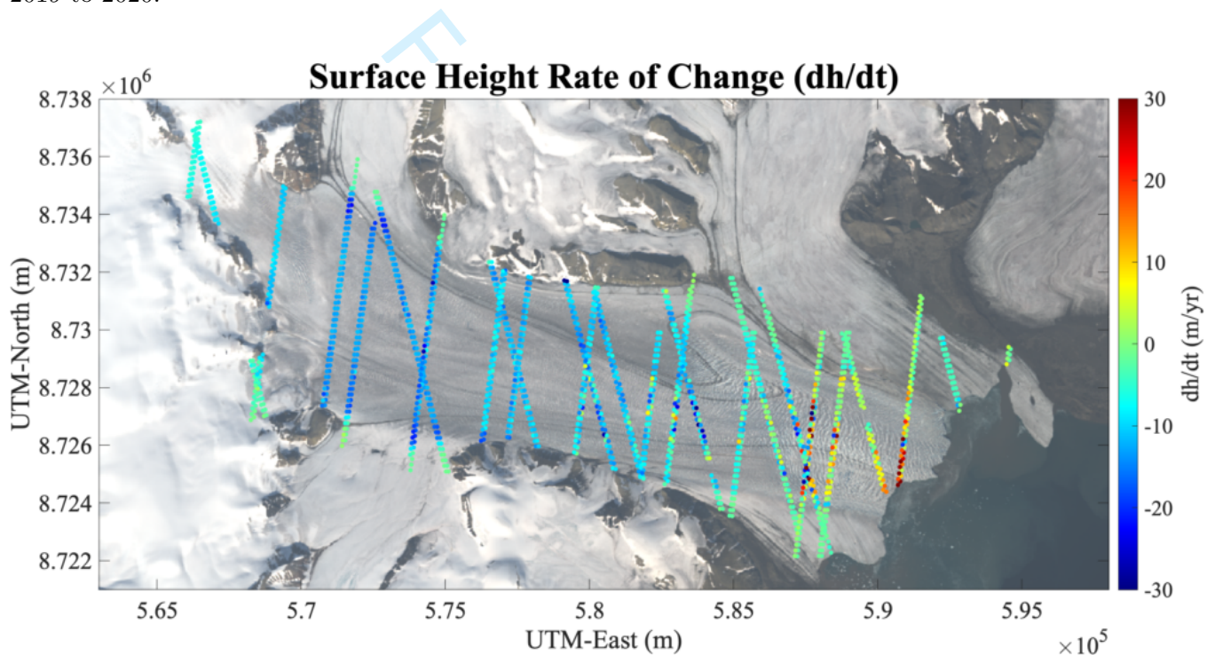
Fig. 8. Rates of change of glacier surface height during the 2019-2020 part of the recent Negribreen surge. Surface height change rate in meters per year.
