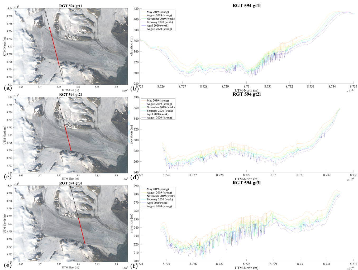
Fig. 12. DDA-ice results for RGT 594 over the Negribreen's major surge-affected area, 2019-2020. (a)-(b) RGT 594 gt11, (c)-(d) RGT 594 gt21, and (e)-(f) RGT 594 gt31.
