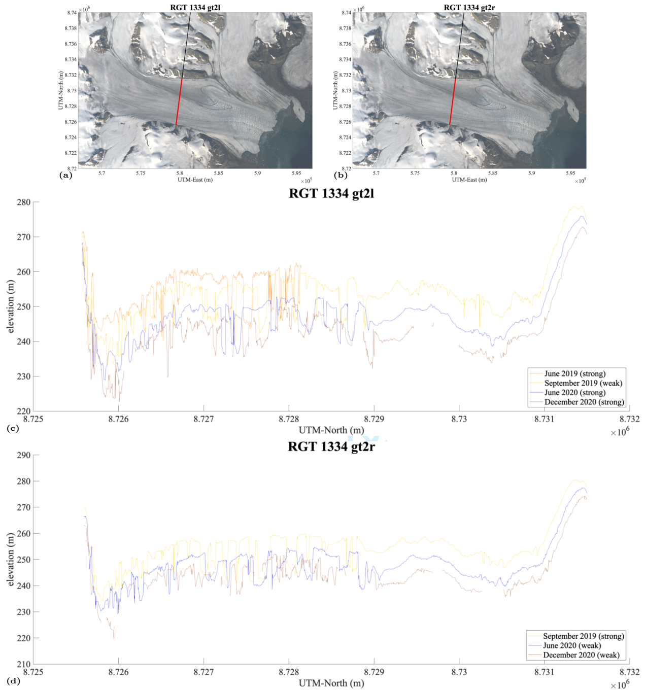
Figure 24: ICESat-2/DDA-ice surface height time series for RGT 1334 beam pair 2 over Negribreen, 2019-2020. (a) Location of RGT 1334 gt2l segment over Negribreen, (b) Location of RGT 1334 gt2r segment over Negribreen, (c) surface height time series of RGT 1334 gt2l, and (d) surface height time series of RGT 1334 gt2r.
