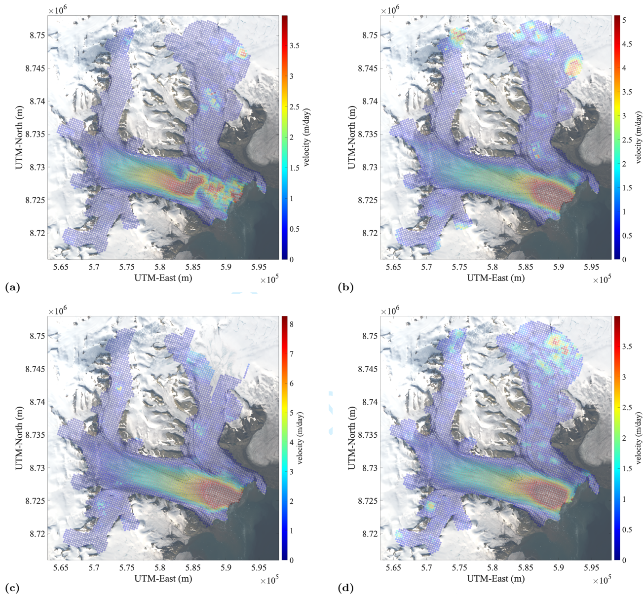
Fig. 5. Negribreen velocity maps from 2019-2020. Maps are derived from Sentinel-1 SAR data. (a) Mean surface velocities between 2019-01-05 to 2019-03-30 (m/day). Over a longer \sim 3 month baseline, velocity information can become lost or skewed in areas of high deformation as seen near the terminus. (b) Mean surface velocities between 2019-08-11 to 2019-08-23 (m/day). This baseline spans the 2019 airborne campaigns in August 2019. (c) Mean surface velocities between 2020-07-10 to 2020-07-22 (m/day) with peak surge speeds exceeding 8 m/day. July typically sees the fastest ice-surface speeds in Negribreen. (d) Mean surface velocities between 2020-12-19 to 2020-12-31 (m/day) at the end of the study period in December 2020 which shows typical velocities during the winter months of 2019 and 2020.
