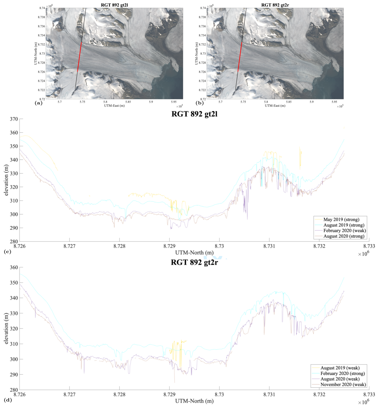
Figure 18: ICESat-2/DDA-ice surface height time series for RGT 892 beam pair 2 over Negribreen, 2019-2020. (a) Location of RGT 892 gt2l segment over Negribreen, (b) Location of RGT 892 gt2r segment over Negribreen, (c) surface height time series of RGT 892 gt2l, and (d) surface height time series of RGT 892 gt2r.
