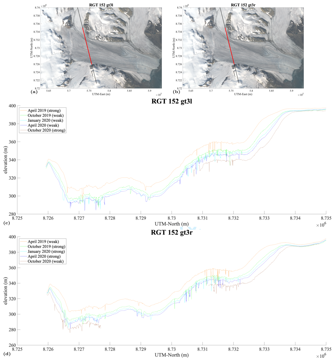
Figure 7: ICESat-2/DDA-ice surface height time series for RGT 152 beam pair 3 over Negribreen, 2019-2020. (a) Location of RGT 152 gt3l segment over Negribreen, (b) Location of RGT 152 gt3r segment over Negribreen, (c) surface height time series of RGT 152 gt3l, and (d) surface height time series of RGT 152 gt3r.
