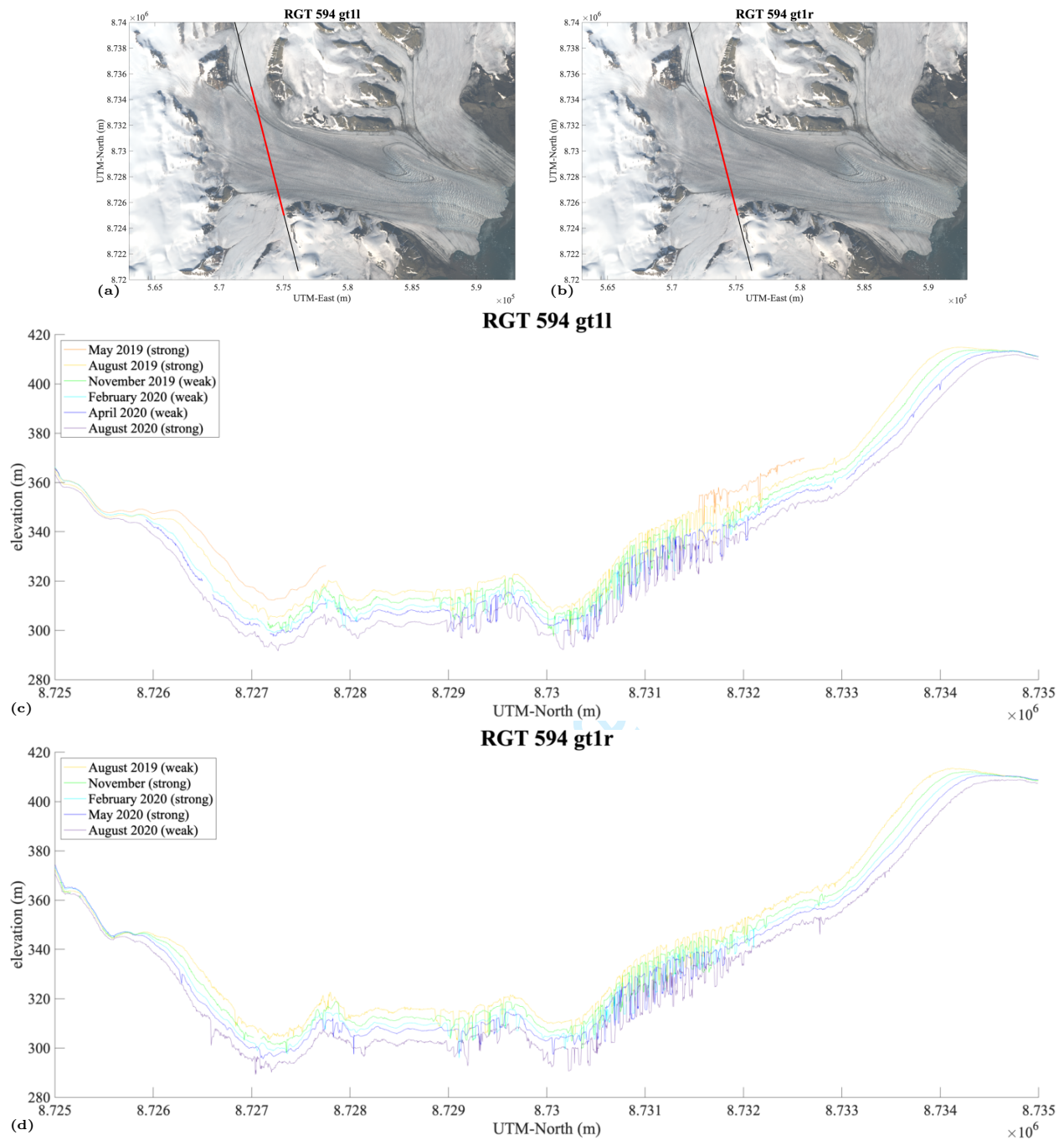
Figure 14: ICESat-2/DDA-ice surface height time series for RGT 594 beam pair 1 over Negribreen, 2019-2020. (a) Location of RGT 594 gt1l segment over Negribreen, (b) Location of RGT 594 gt1r segment over Negribreen, (c) surface height time series of RGT 594 gt1l, and (d) surface height time series of RGT 594 gt1r.
