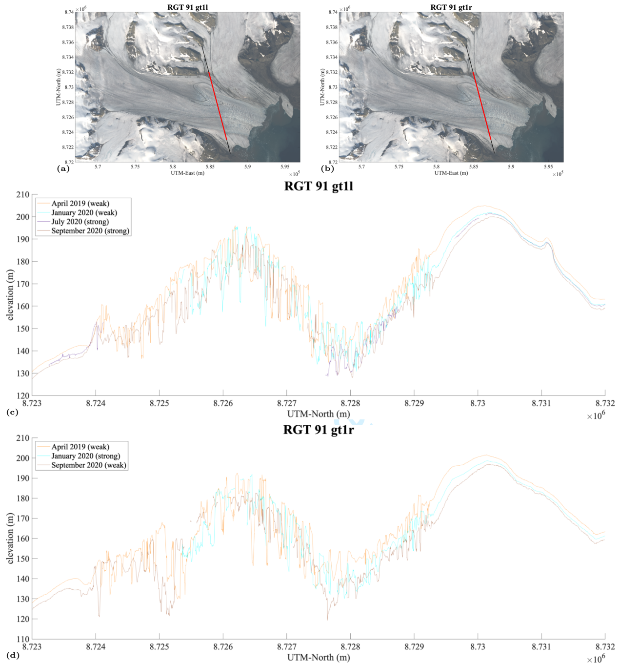
Figure 2: ICESat-2/DDA-ice surface height time series for RGT 91 beam pair 1 over Negribreen, 2019-2020. (a) Location of RGT 91 gt1l segment over Negribreen, (b) Location of RGT 91 gt1r segment over Negribreen, (c) surface height time series of RGT 91 gt1l, and (d) surface height time series of RGT 91 gt1r.
