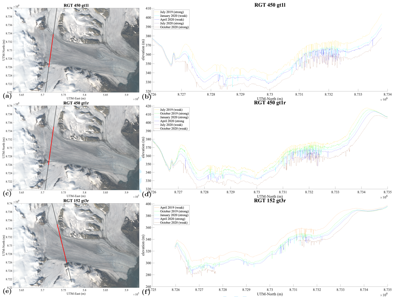
Fig. 13. Further expansion of crevasses in upper Negribreen as given by ICESat-2's RGT 450 and 152, 2019-2020. (a)-(b) RGT 450 gt11, (c)-(d) RGT 450 gt1r and (e)-(f) RGT 152 gt3r.
