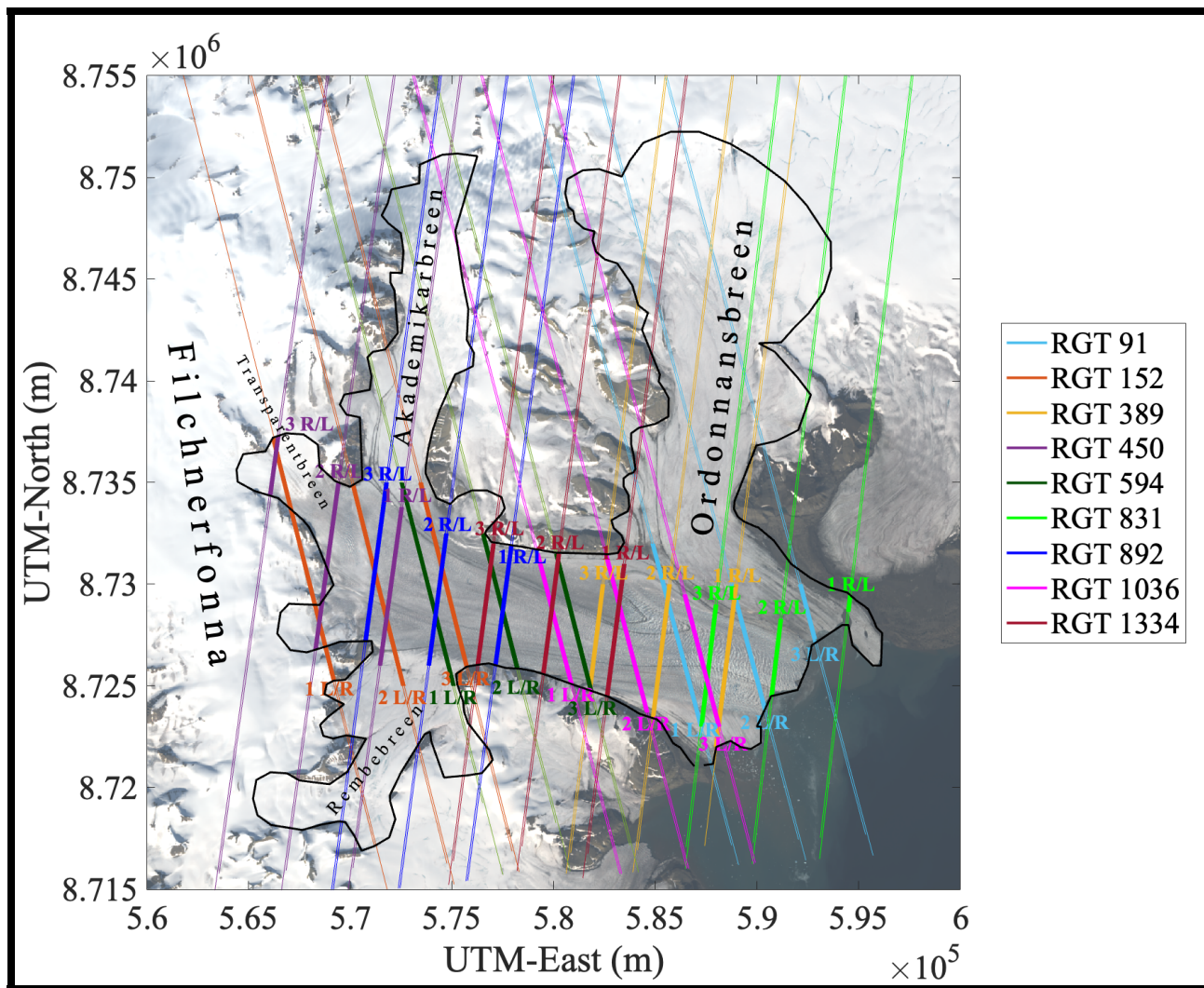
Fig. 2. ICESat-2 survey lines over the Negribreen Glacier System. The survey lines for each of ICESat-2's three beam-pairs are color coded by their Reference Ground Track (RGT) while the NGS borders are given by the black line. The thick lines correspond to the part of the track that is analyzed in this paper which is mostly equivalent to the boundaries of Negribreen Glacier. Left/Right (L/R) beam-pairs are separated by \sim 90 m on-ice which is within line thickness over Negribreen in this figure. Background image from Landsat-8 acquired 2019-08-05.
