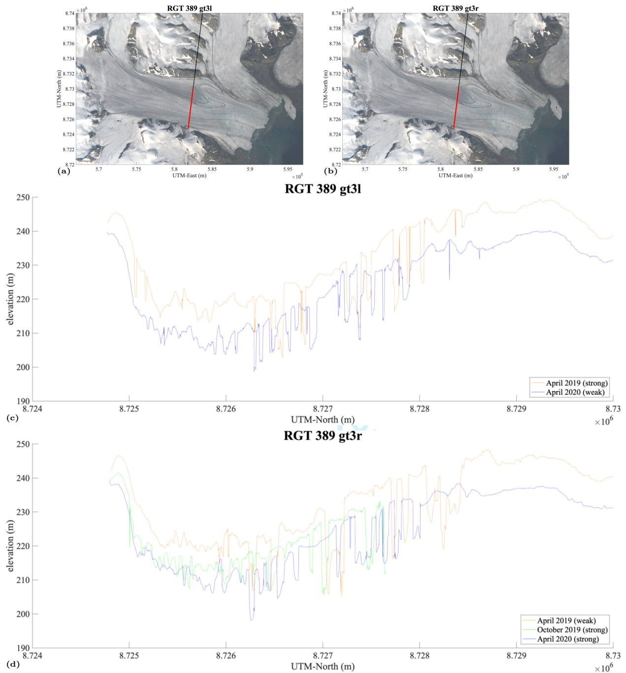
Figure 10: ICESat-2/DDA-ice surface height time series for RGT 389 beam pair 3 over Negribreen, 2019-2020. (a) Location of RGT 389 gt3l segment over Negribreen, (b) Location of RGT 389 gt3r segment over Negribreen, (c) surface height time series of RGT 389 gt3l, and (d) surface height time series of RGT 389 gt3r.
