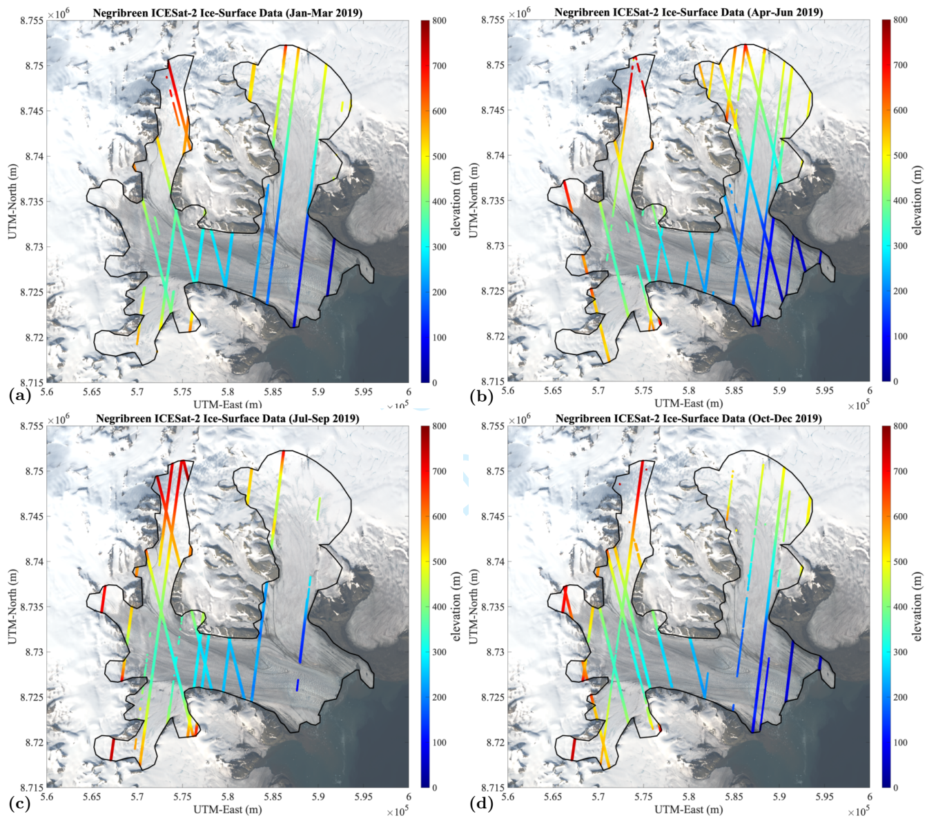
Fig. 6. 2019 Negribreen ice-surface height data from the DDA-ice for single ICESat-2 cycles (91 days).
