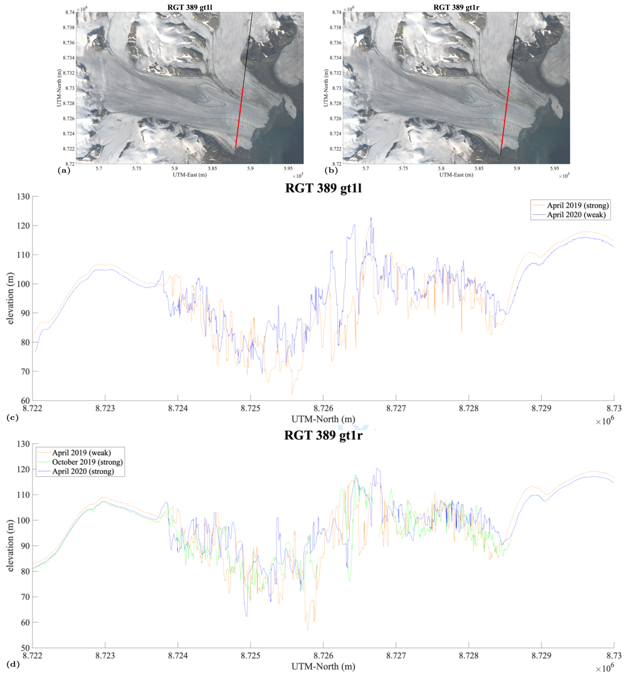
Figure 8: ICESat-2/DDA-ice surface height time series for RGT 389 beam pair 1 over Negribreen, 2019-2020. (a) Location of RGT 389 gt1l segment over Negribreen, (b) Location of RGT 389 gt1r segment over Negribreen, (c) surface height time series of RGT 389 gt1l, and (d) surface height time series of RGT 389 gt1r.
