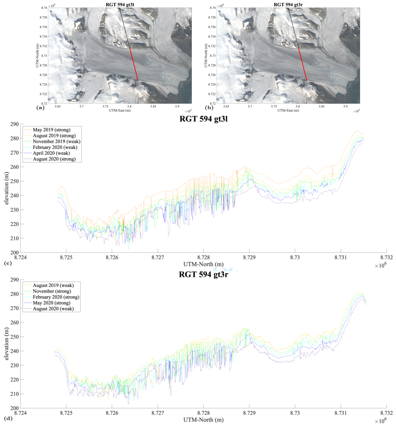
Figure 16: ICESat-2/DDA-ice surface height time series for RGT 594 beam pair 3 over Negribreen, 2019-2020. (a) Location of RGT 594 gt3l segment over Negribreen, (b) Location of RGT 594 gt3r segment over Negribreen, (c) surface height time series of RGT 594 gt3l, and (d) surface height time series of RGT 594 gt3r.
