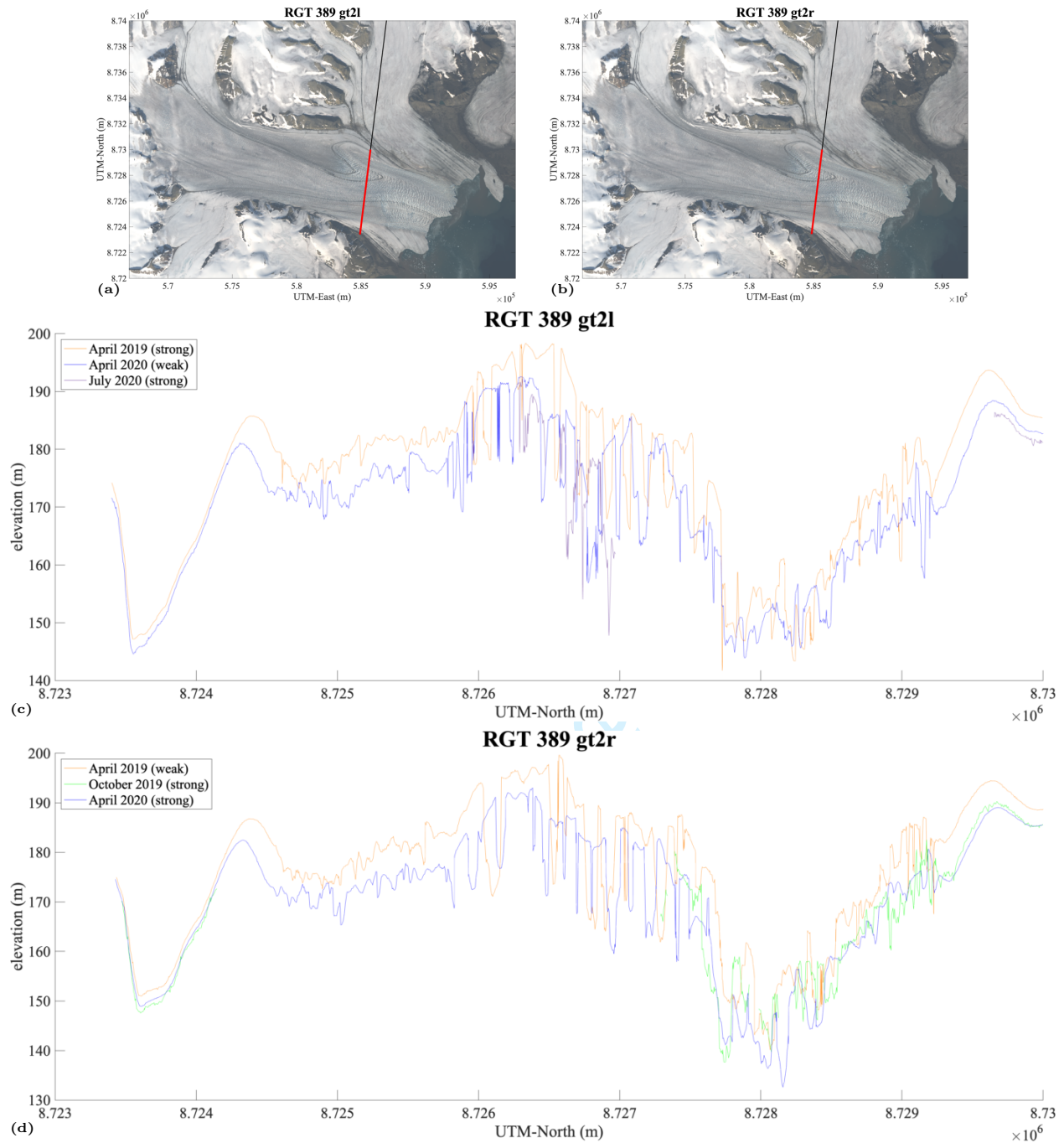
Figure 9: ICESat-2/DDA-ice surface height time series for RGT 389 beam pair 2 over Negribreen, 2019-2020. (a) Location of RGT 389 gt2l segment over Negribreen, (b) Location of RGT 389 gt2r segment over Negribreen, (c) surface height time series of RGT 389 gt2l, and (d) surface height time series of RGT 389 gt2r.
