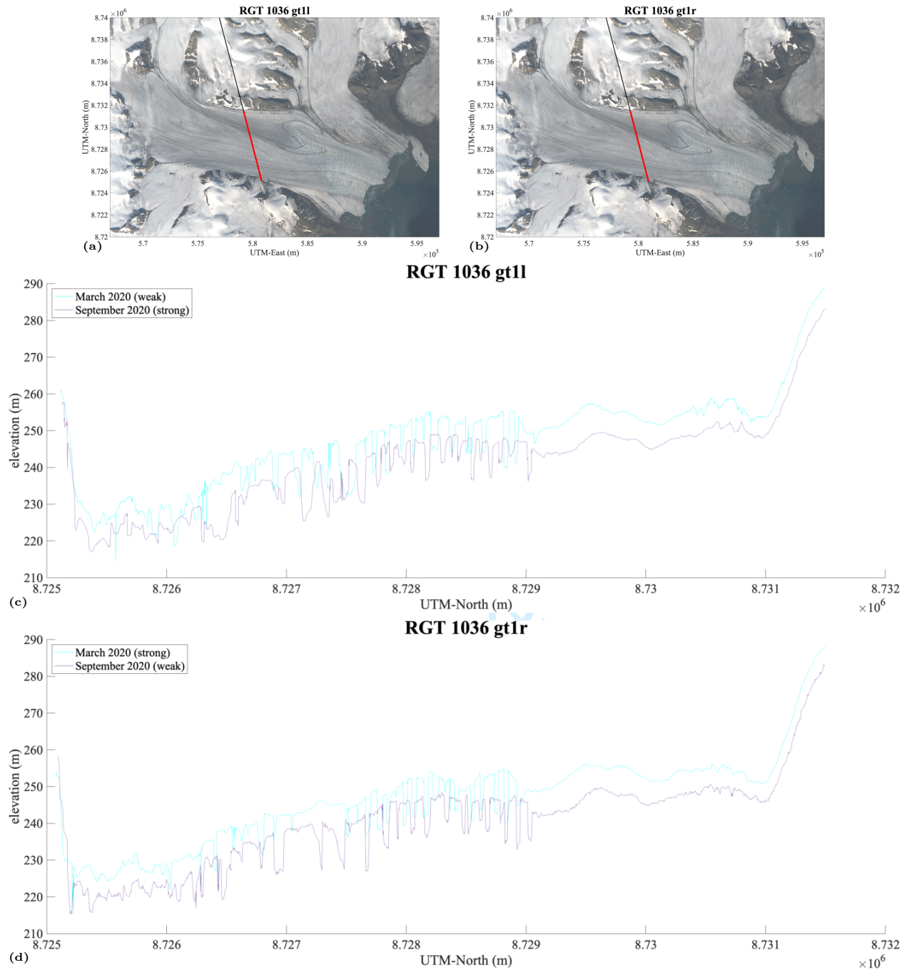
Figure 20: ICESat-2/DDA-ice surface height time series for RGT 1036 beam pair 1 over Negribreen, 2019-2020. (a) Location of RGT 1036 gt1l segment over Negribreen, (b) Location of RGT 1036 gt1r segment over Negribreen, (c) surface height time series of RGT 1036 gt1l, and (d) surface height time series of RGT 1036 gt1r.
