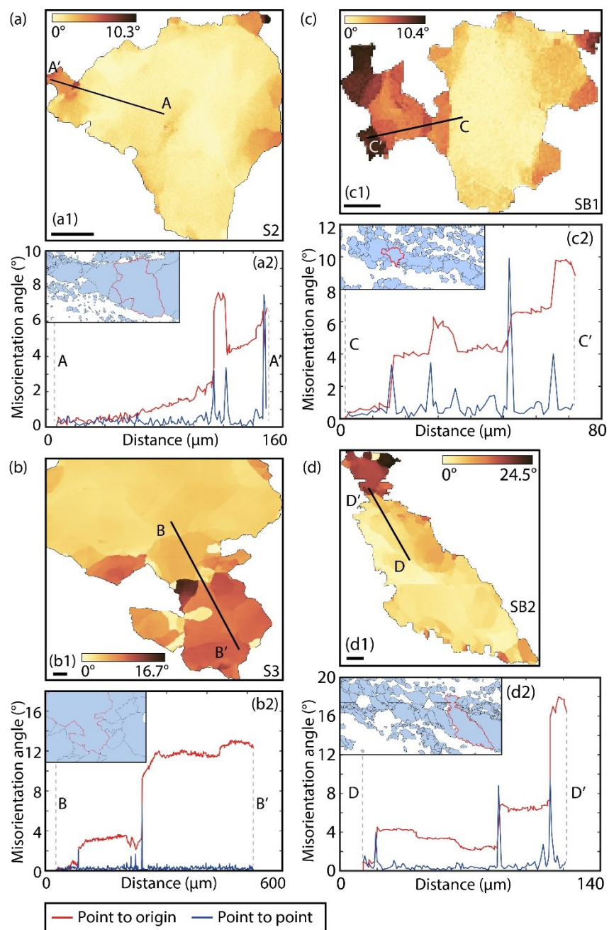
Fig. 11. Misorientation to mean orientation ( mis2mean ) maps of selected quartz grains of the host rock (outside the shear bands) and the core-to-rim misorientation line profiles. (a) S2 (outside SB2). (b) S3 (outside SB3). (c) SB1. (d) SB2. The misorientation profile for each grain is shown right below it. Both ‘point-to-origin’ (red) and ‘point-to-point’ (blue) misorientation profiles are shown. The grains of interest are shown in the inset phase maps. The complete phase map of (a, d) is in Fig. 7b , of (b) is in Supplementary Fig. SF10 , and that of (c) can be seen in Fig. 7a . All the black bars present below the mis2mean maps are 50 mm long for (a, b) and 25 mm long for (c, d). The ‘lajolla’ colour map of Crameri (2018) is used here.
