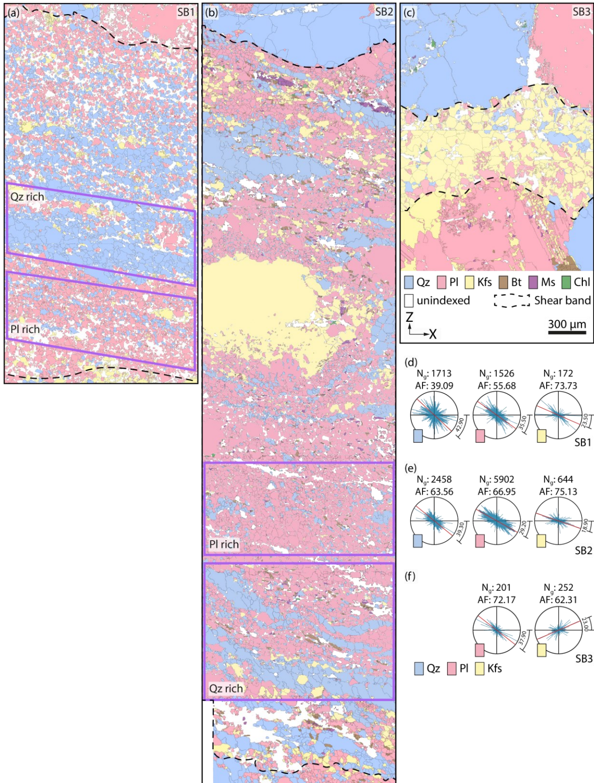
Fig. 7. EBSD-derived phase maps of (a) SB1, (b) SB2 and (c) SB3. Purple solid boxes are quartz and plagioclase-rich regions used for EBSD analyses. (a) and (b) have same scale, legend, and orientation as those of (c). The black dashed curves demarcate the shear bands. Mineral
