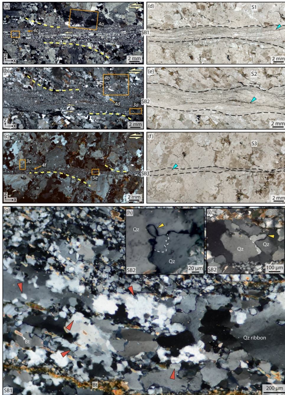
Fig. 2. Photomicrographs of the shear bands. (a, d) SB1, (b, e) SB2 and (c, f) SB3. (a) – (c) are cross-polarised images. (d) – (f) are plane-polarised images. Black dashed curves demarcate the shear bands in (d) – (f). The deflected markers (yellow dashed curves) in (a) – (c) and sigmoid polycrystalline quartz aggregates in (a) and (b) indicate sinistral ductile shear senses. The orange boxes and arrows mark the locations of figures used in Figs. 2-5. The thread-like networks of phyllosilicate grains are shown using cyan arrowheads. Quartz deformation microstructures (g) – (i). Grain boundary migration bulges (yellow arrowheads) and subgrains (red arrowheads) in the quartz ribbons within SB1 and SB2. The bulges and subgrains are nearly
