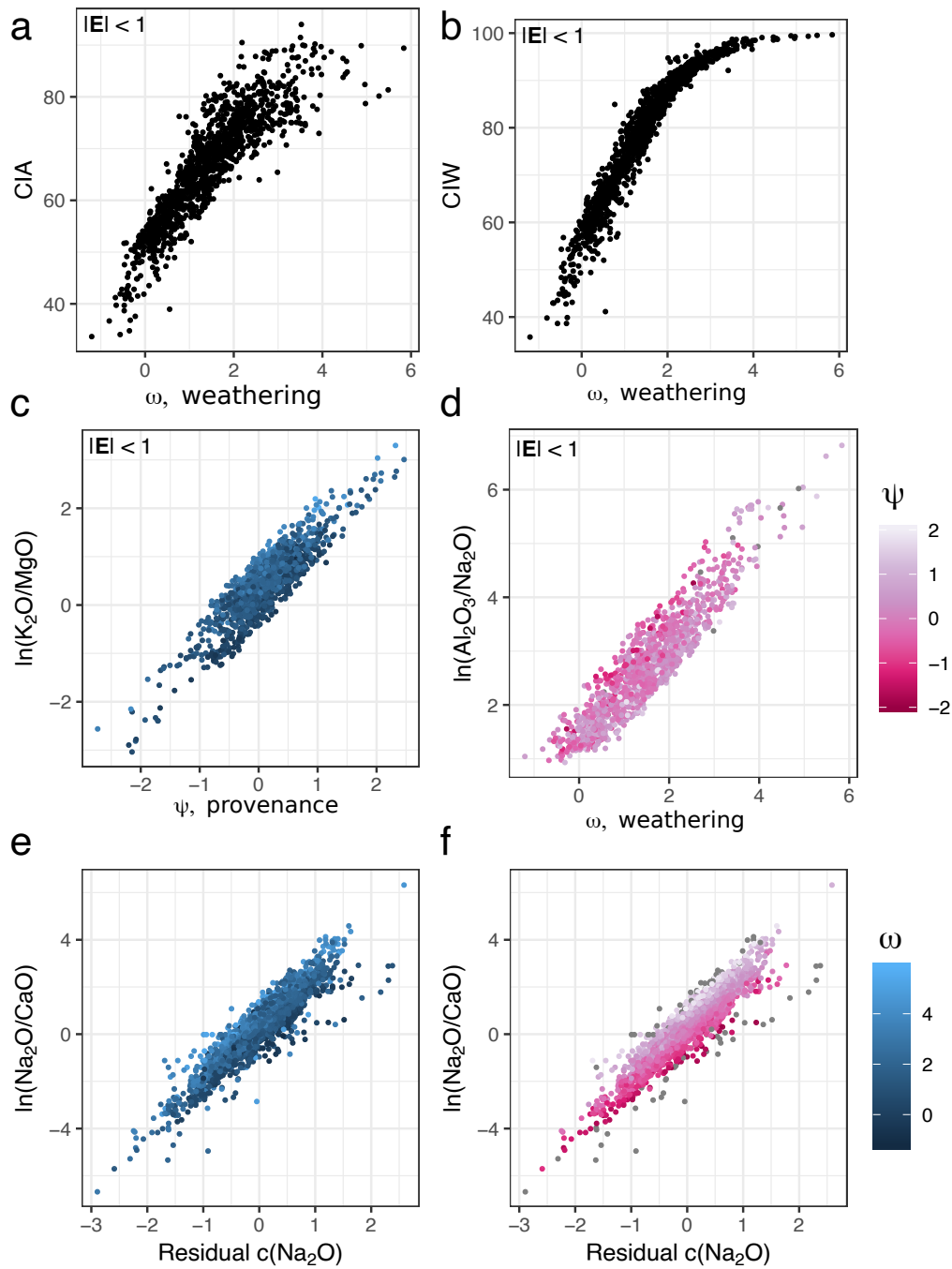
Figure 11. Comparison of \omega to the Chemical Index of Alteration (CIA) (a) and Chemical Index of Weathering (CIW) (b) shows that all are strongly related, but the CIW saturates at higher \omega values. (c) indicates that \ln(K_2O/MgO) is a good proxy for \psi and is weakly affected by weathering. (d) indicates that \ln(Al_2O_3/Na_2O) is a good proxy for \omega and is weakly affected by provenance. (e) & (f) indicate that \ln(Na_2O/CaO) is a good proxy for diagenesis and is weakly affected by both weathering and provenance. Figures 11a-d only show samples with residual magnitude < 1 .
