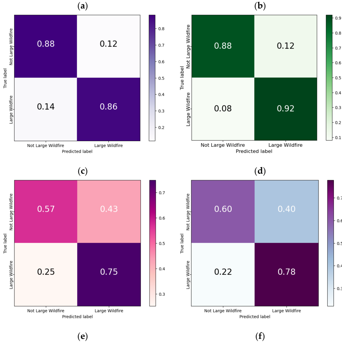
Figure 4. Validation of actual vs. predicted large wildfire classification through confusion matrix: (a) Logistic Regression model with a TPR of 0.75 and a TNR of 0.64; (b) Decision Tree Classification model with a TPR of 0.83 and a TNR of 0.67; (c) Random Forest Classification model with a TPR of 0.86 and a TNR of 0.88; (d) XGBoost Classification model with a TPR of 0.92 and a TNR of 0.88; (e) KNN Classification model with a TPR of 0.75 and a TNR of 0.57; (f) SVM Classification model with a TPR of 0.78 and a TNR of 0.60.
