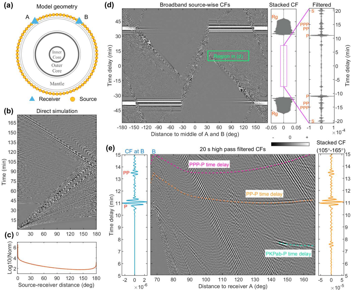
Figure 1: (a) Geometry of the model for synthesizing the inter-receiver ANC. (b) Global seismograms simulated using AxiSEM. (c) Variations of the logarithm of norms of two-hour seismograms with respect to distance. (d) Source stack for synthesizing the ANC between two stations 68^\circ apart, at periods from 10 s to 100 s. (e) An enlarged part of (d), at periods from 10 s to 20 s.
