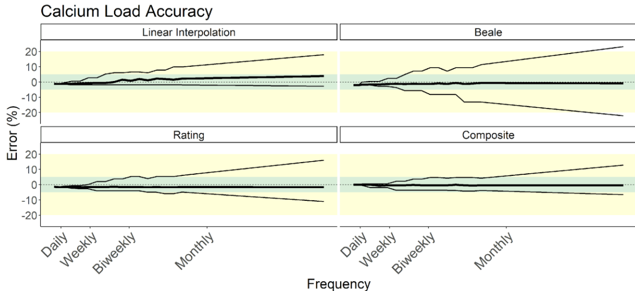
Figure 12: Results from applying four different load estimation methods to artificially coarsened, high-frequency sensor time series of Calcium, taken from Plynlimon Research Catchments' Upper Hafren site. Percent error of estimated annual load from the "true" load, calculated using the full time series, is on the y-axis. Coarsened data frequency is on the x-axis. The solid line indicates the median error for that frequency, with thin lines indicating
