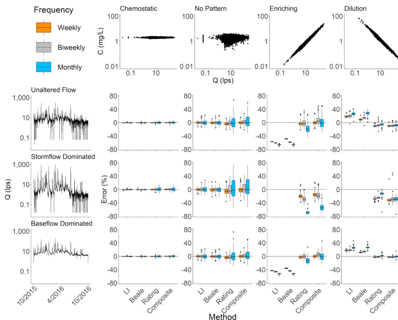
Figure 13: Load estimation error across chemodynamic and hydraulic regimes, and four estimation methods. Load estimates were generated from simulated data. The top row of plots describes the concentration discharge relationship. The side column of plots describes the hydrologic regime. The grid of boxplots is the result of applying the four estimation methods across each combination of concentration discharge relationship and hydrologic regime. Linear interpolation (LI) and Beale estimates from enriching or diluting time series under stormflow conditions, and some outlier values (beyond 1.5 interquartile ranges) excluded for readability. A table of summary values for all methods, hydrologic regimes, and C:Q relationships is available in supplementary_table_1.csv . Note that no-pattern
