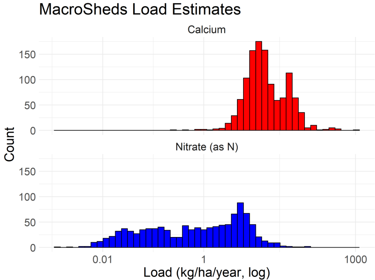
Figure 14: A histogram of annual load estimates present in the MacroSheds dataset. The complete load calculations from each solute and site-year of MacroSheds data are available at 10.6084/m9.figshare.24975504 .
