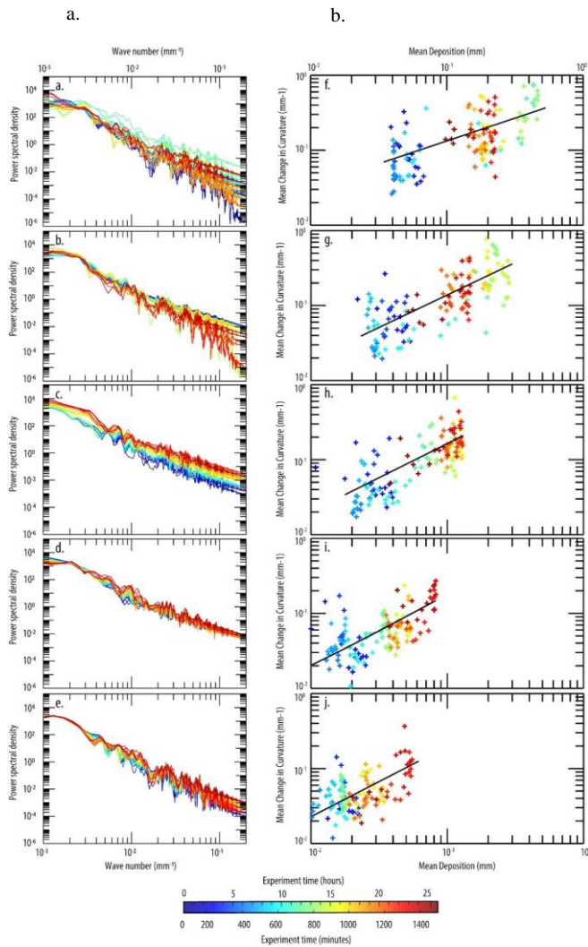
Figure 9: (a) Power spectral densities of the sub-aqueous slope through time. (b) The mean change in the absolute value of surface curvature versus mean deposition rate at each transect through time. The highest mean deposition rates occurred at 2.5 m from the inlet at ~13 hours and were connected to the rapid growth of delta lobes and associated significant changes in cross stream surface curvature.
