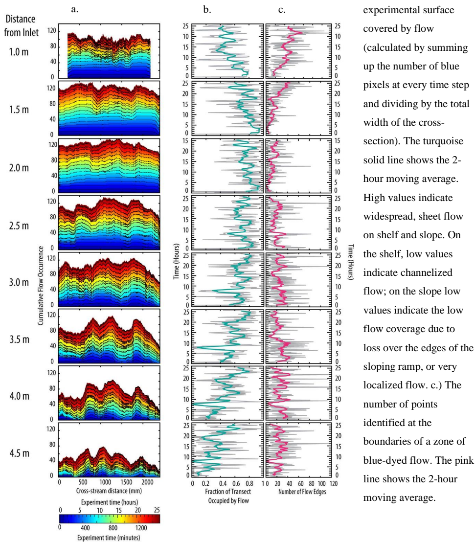
Figure 6: a.) The cumulative count of pixels with blue-dyed flow at each point along strike-oriented transects at 1.5, 2, 2.5, 3, 3.5, 4, 4.5 m from the inlet. The color bar is used to indicate time. Black lines are time-lines plotted every 100 minutes. Peaks indicate locations that were visited by subaerial flow or subaqueous turbidity currents most often. The difference between high and low values in these cumulative plots grows more pronounced from proximal to distal areas. b.) The fraction of the
