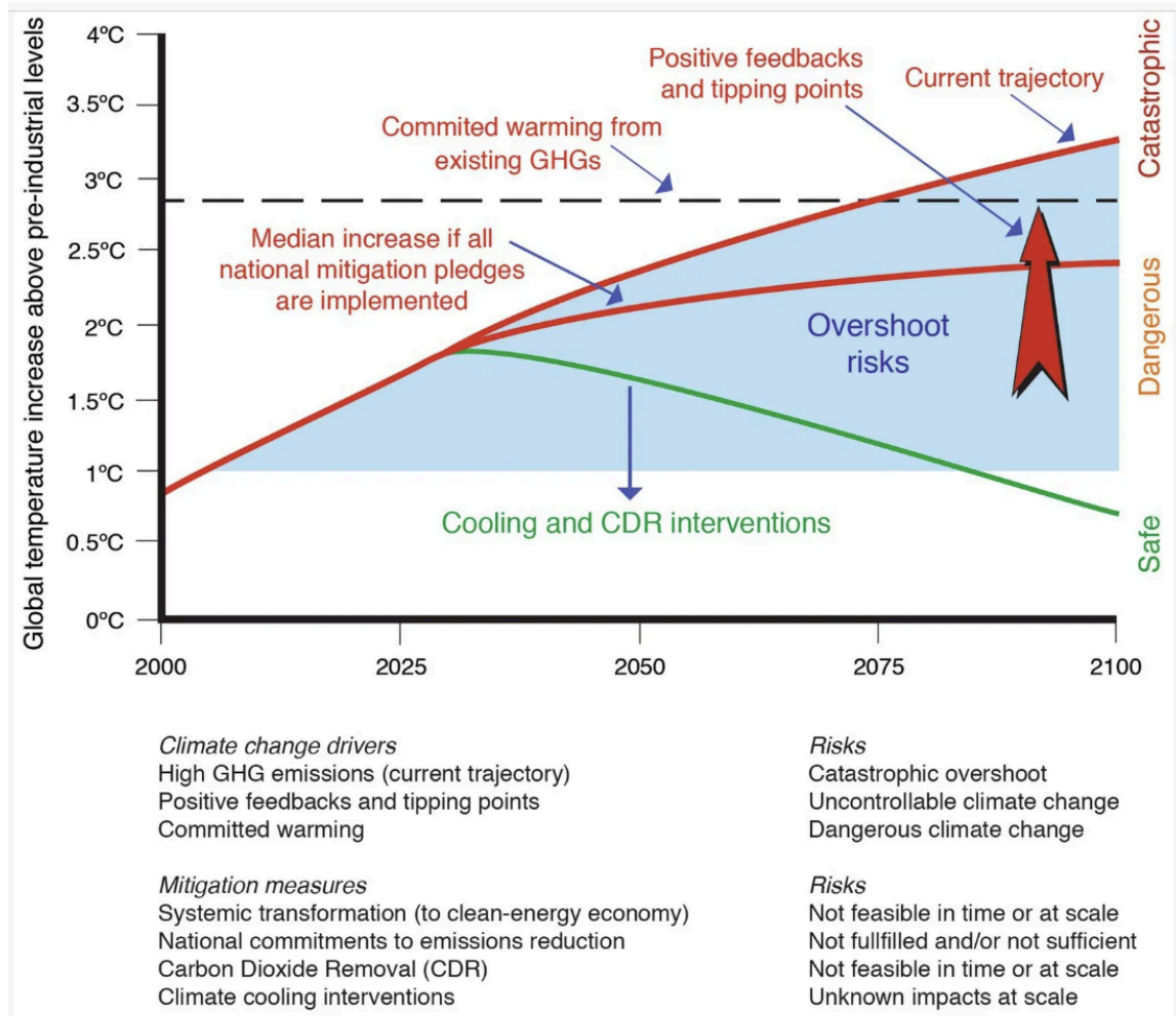
Figure 10. Possible Global Temperature Risks and Trajectories
