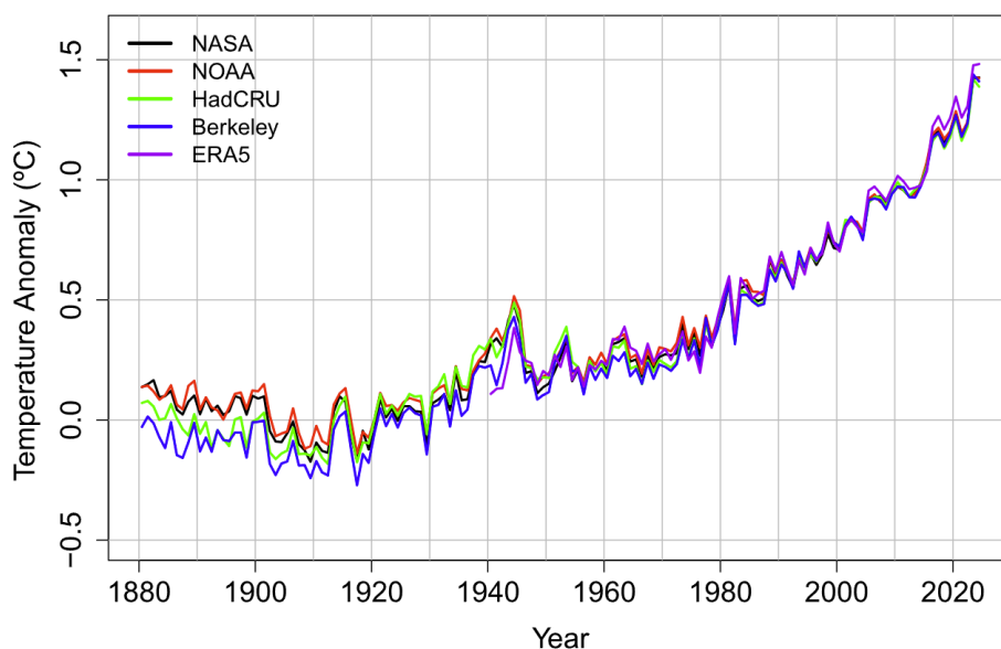
Figure 1 from Foster & Rahmstorf (2026). “Yearly average global mean surface temperature from five data sources, in two versions: (top) [not included here], (bottom) adjusted for El Niño/Southern Oscillation, volcanism, and solar variation. All are aligned
