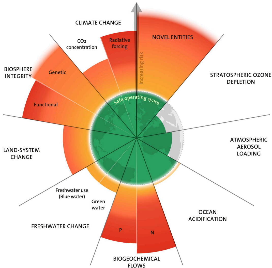
Figure 1. Planetary Boundaries: Nine Assessed, Six Crossed
