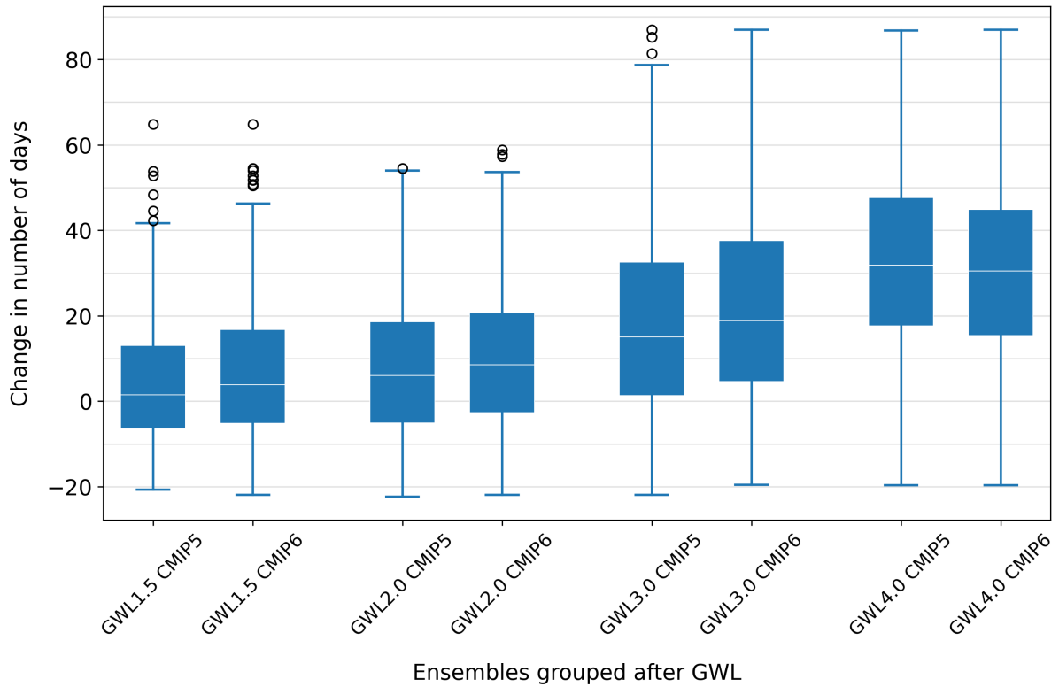
Change in annual number of days in Kyselý periods in Vienna, AT relative to 1991-2020 for CMIP5 and CMIP6 at four GWLs
