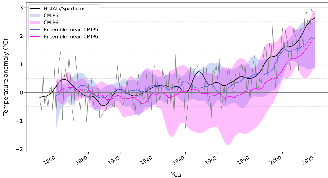
Regional temperature anomalies in Austria compared to 1850-1900 for two model ensembles (CMIP5, CMIP6) and HistAlp observational data
