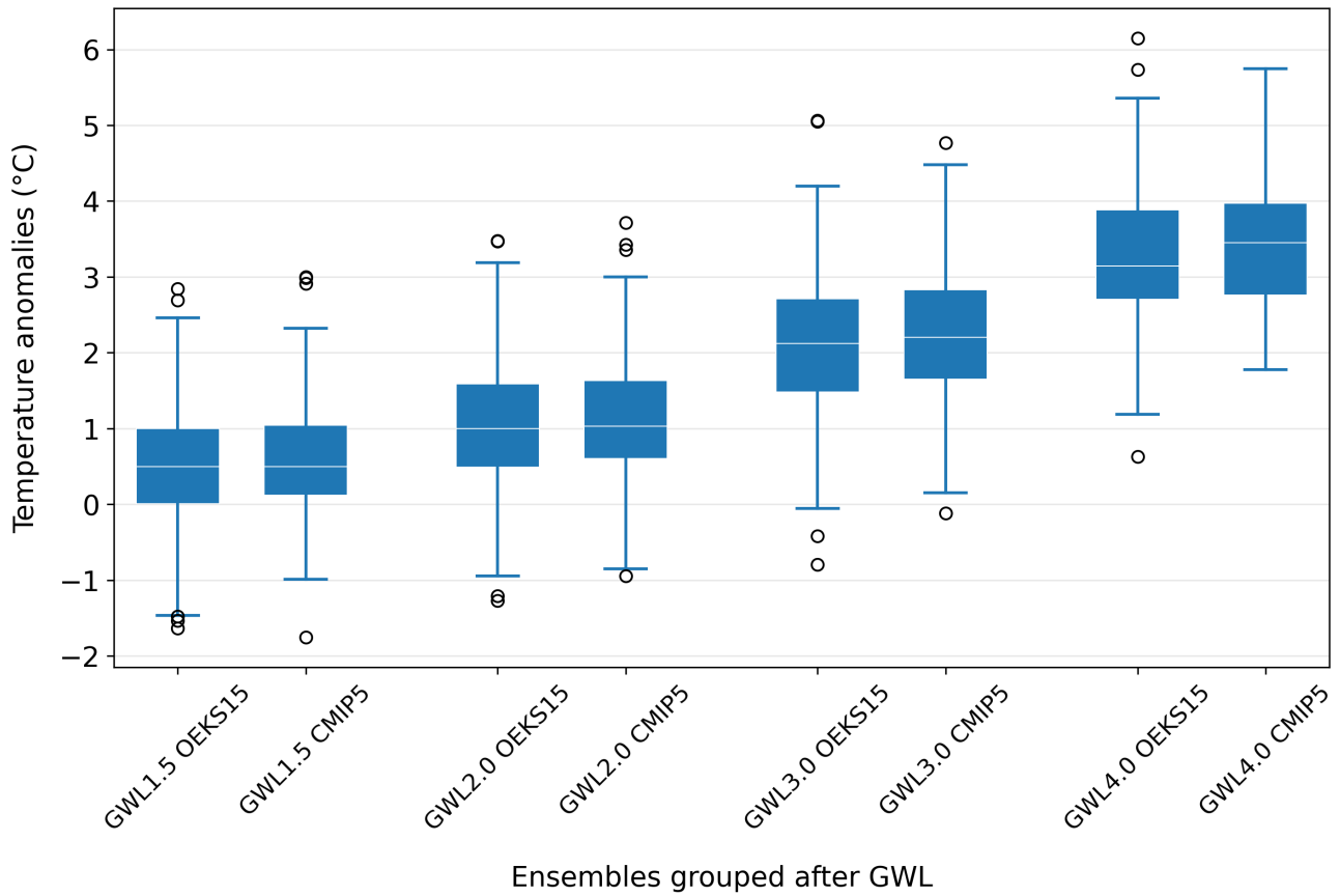
Annual mean temperature anomalies in Austria relative to 1991-2020 for OEKS15 and CMIP5 background models at four GWLs
