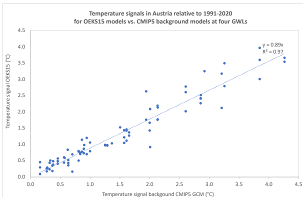
Figure 2: Correlation between mean temperature signals of the OEKS15 ensemble and their respective background GCM in Austria at four GWLs. Each data point represents the mean temperature change of a 20-year period at the time when a model crosses a certain GWL, and the period 1991-2020. On the y-axis, temperature signals of all OEKS15 models reaching the respective GWLs are shown. The x-axis depicts the temperature signal of the associated background GCM.
