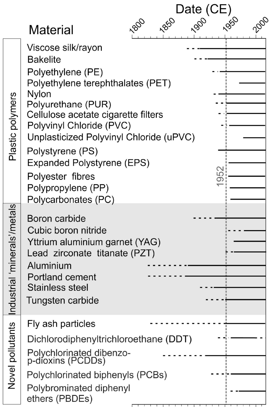
Figure 3. Range zones of common novel plastic polymers, synthetic mineral-like compounds, metals and industrial pollutants; dashed lines denote relative low abundances. NB dioxins occurred naturally before ~1850 CE but in low concentrations. From Waters et al. (2018b).
