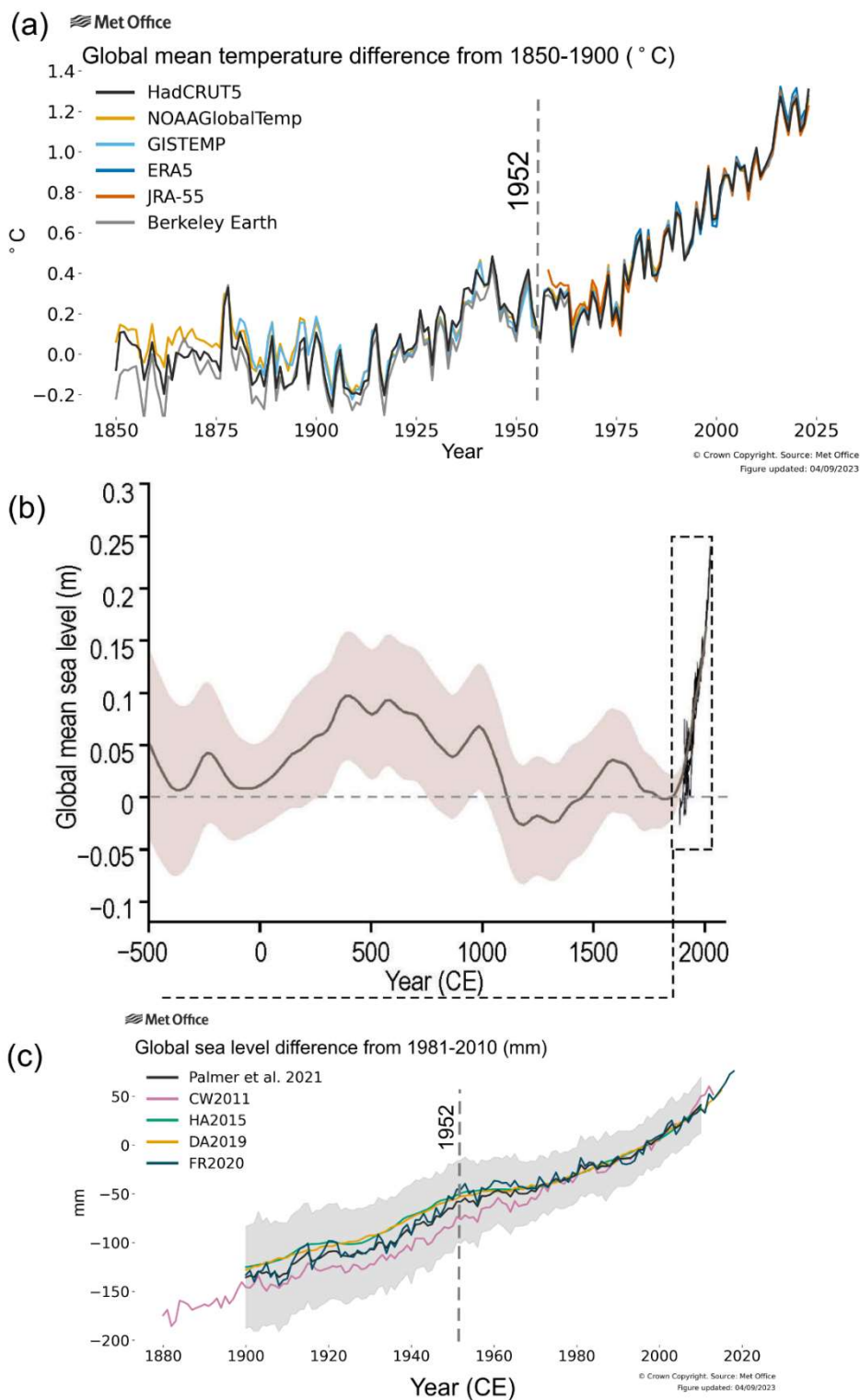
Figure 17. Changes in global temperature and mean sea level. (a) Annual global mean temperatures expressed as a difference from pre-industrial conditions using different data sets (from Met Office 2023 https://climate.metoffice.cloud/temperature.html ); (b) reconstructions for the last 2500 years based upon a range of proxy sources with direct instrumental records superposed since the late 19 th century (from IPCC, 2021, fig. 2.28); (c) annual global mean sea-level from 1870-present expressed as a difference from the average for 1993-2010. A number of longer tide gauge-based records are shown (from Met Office 2023 https://climate.metoffice.cloud/sea_level.html ).
