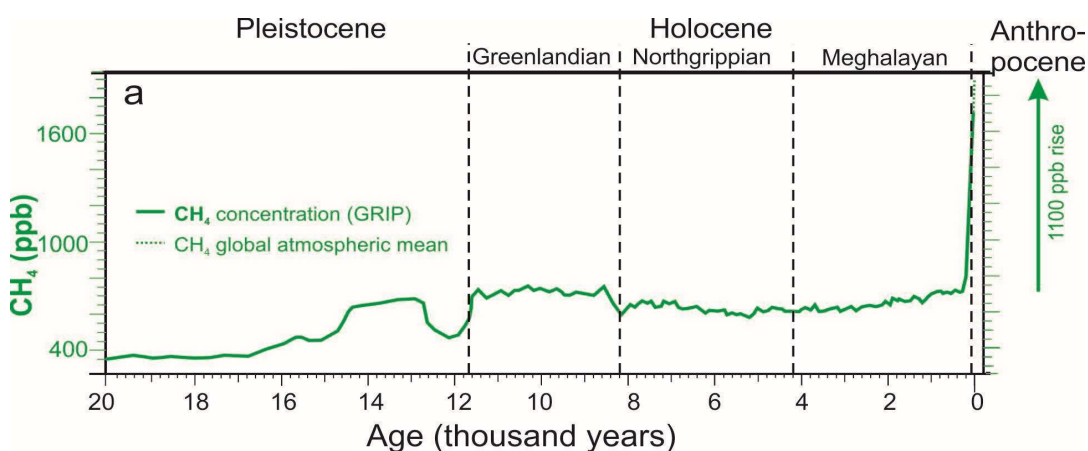
Figure 23. Atmospheric \text{CH}_4 records in ice core from Greenland GRIP (Blunier et al. , 1995) and global atmospheric mean values (NOAA, 2023a).
