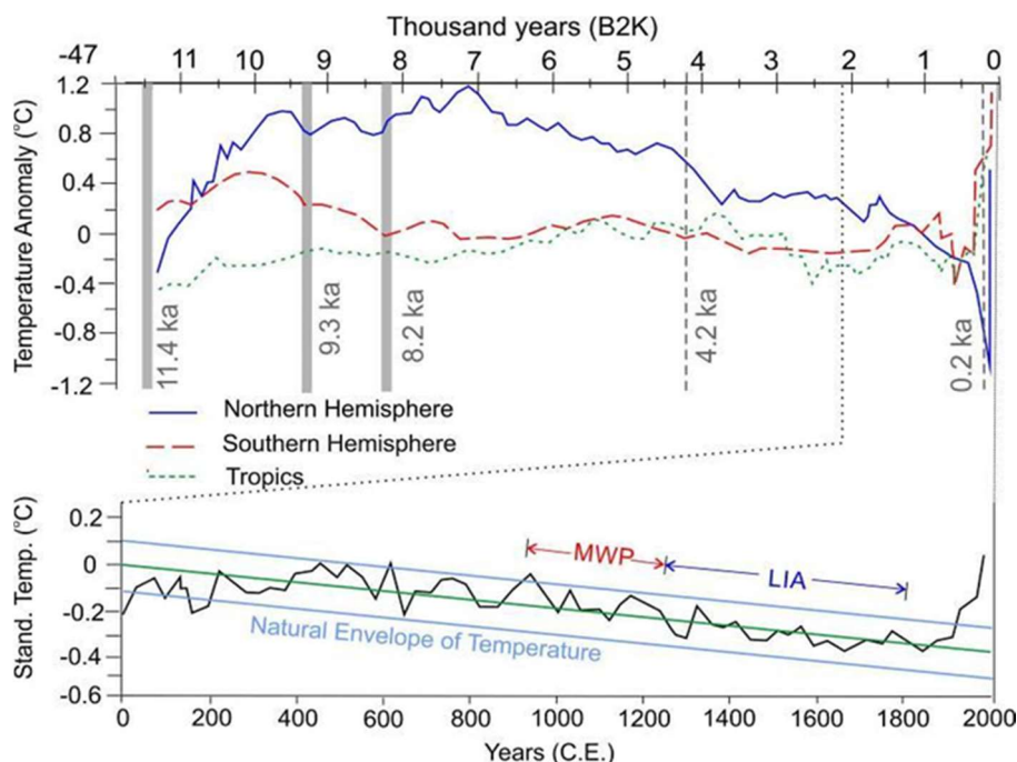
Figure 27. Upper figure shows mean temperature reconstructions for 60° latitude bands (Northern Hemisphere: 90–30°N; Tropics: 30°N–30°S and Southern Hemisphere: 90–30°S; based upon Marcott et al. , 2013). Lower figure shows standardised global mean temperature for the past 2000 years, represented by 30-year means (from Pages 2k Consortium, 2013, redrawn in Waters et al. , 2016), showing the natural temperature envelope for the past 2000 years; Little Ice Age (LIA) and the Medieval Warm Period (MWP) of the Northern Hemisphere are indicated.
