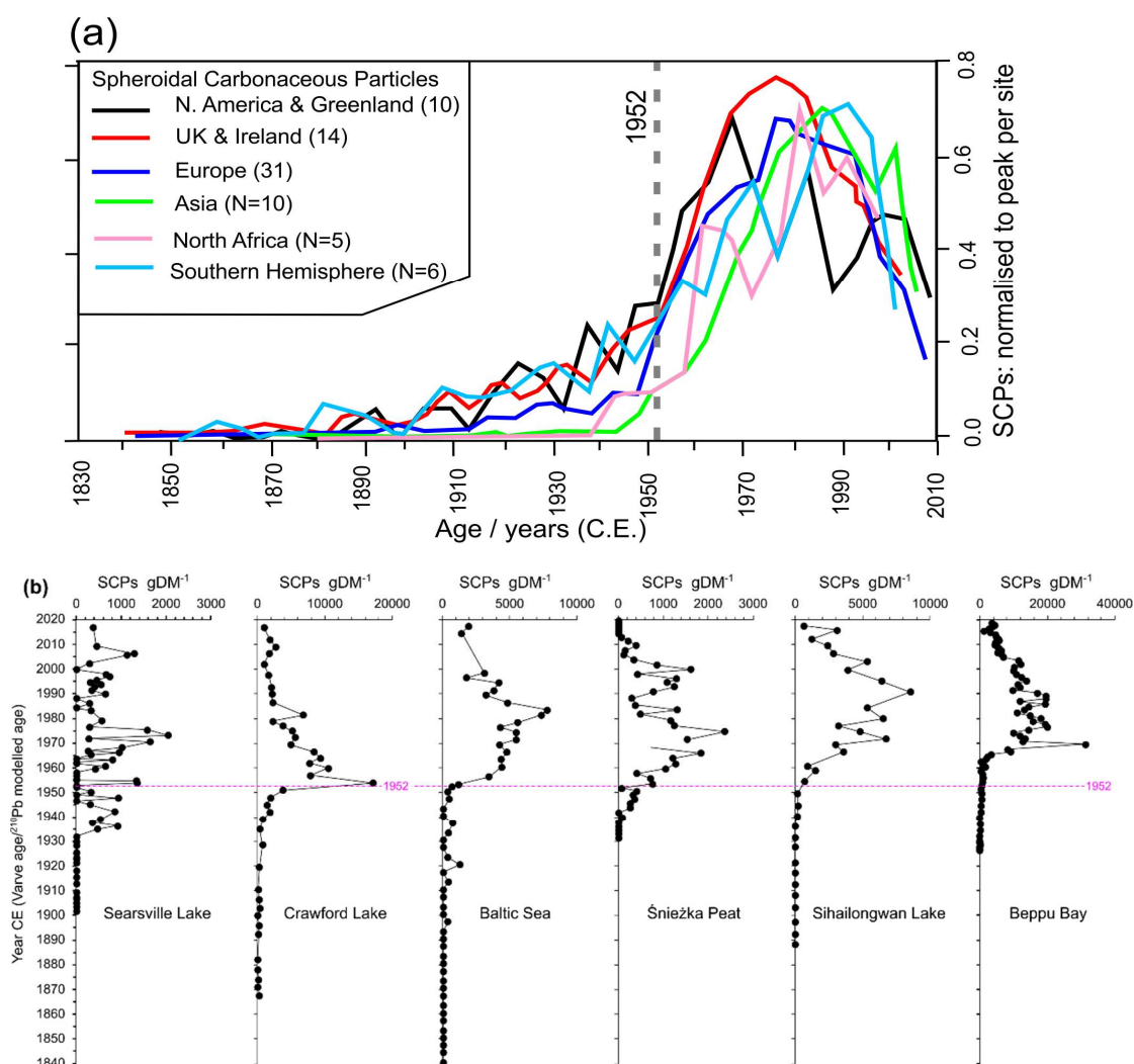
Figure 5. (a) Global mid-20 th century rise and late 20 th century spike in SCPs, normalised to the peak value in each lake core (from Waters et al. , 2016, based on data from Rose, 2015); (b) Concentrations of SCPs (units: numbers of particles per gram dried sediment) in reference sites included in this study (see Part 2).
