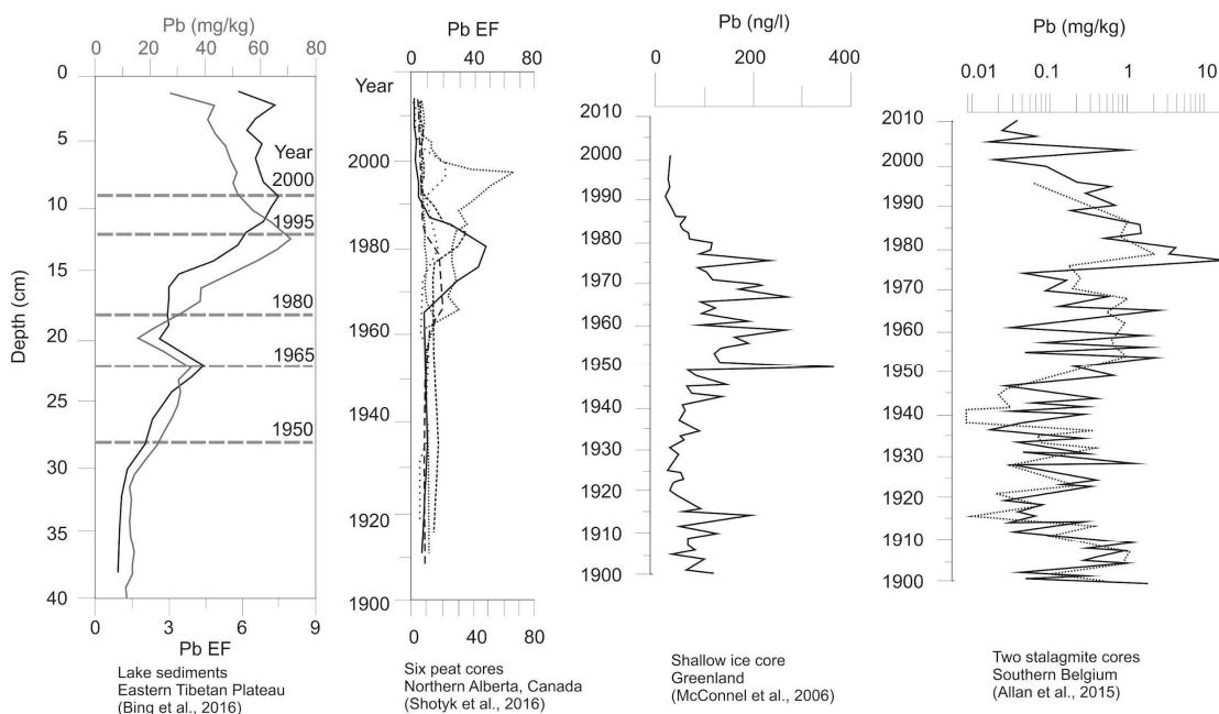
Figure 13. Examples of temporal changes in lead levels in different natural archives during the 20 th century (from Gałuszka & Wagreich, 2019 and references therein). EF-enrichment factor.
