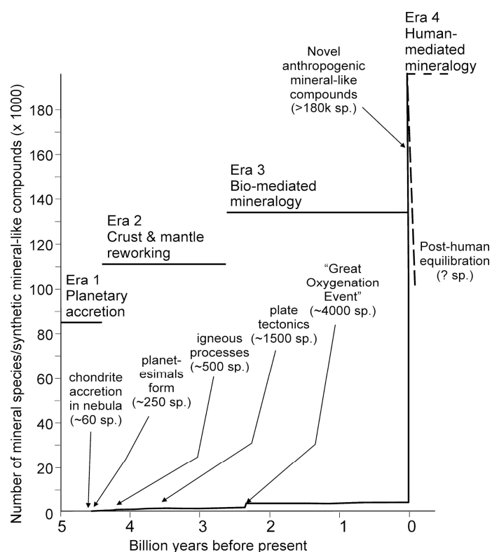
Figure 21. Earth’s mineral evolution (after Hazen et al. , 2008) modified to show the human addition (from Zalasiewicz et al. , 2014a), the scale of which is here shown to be much greater than originally figured (see Hazen et al. , 2017) and since has estimated to have increased to >200,000 mineral-like compounds. From Zalasiewicz et al. (2019a).
