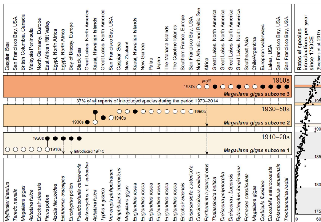
Figure 19. Potential web of palaeontological correlation for three intervals of the 20 th century (from Williams et al. , 2022 and sources therein). White circles are earliest recorded introductions for a specific region; black circles indicate introduced taxa with confirmed palaeontological records (‘lowest occurrence datums’) in their area of introduction. ‘Prolif.’ Means proliferation, noted from human observation of ecologies. The 20 th century global spread of Magallana gigas (Pacific oyster), a species with a fossil range in its native area, is used to suggest a theoretical biozone. Three subzones might be defined within this biozone, with the ability to correlate between marine and non-marine successions at sub-decadal level. Of these, subzone 2 of the M. gigas biozone would correlate with the suggested mid-20 th century start of the Anthropocene. Right side of figure shows the recorded rates of global species introductions since 1750 CE (0–600 per year), reported by Seebens et al. (2017): 37% of all such records of introductions occurred between 1970 and 2014 CE.
