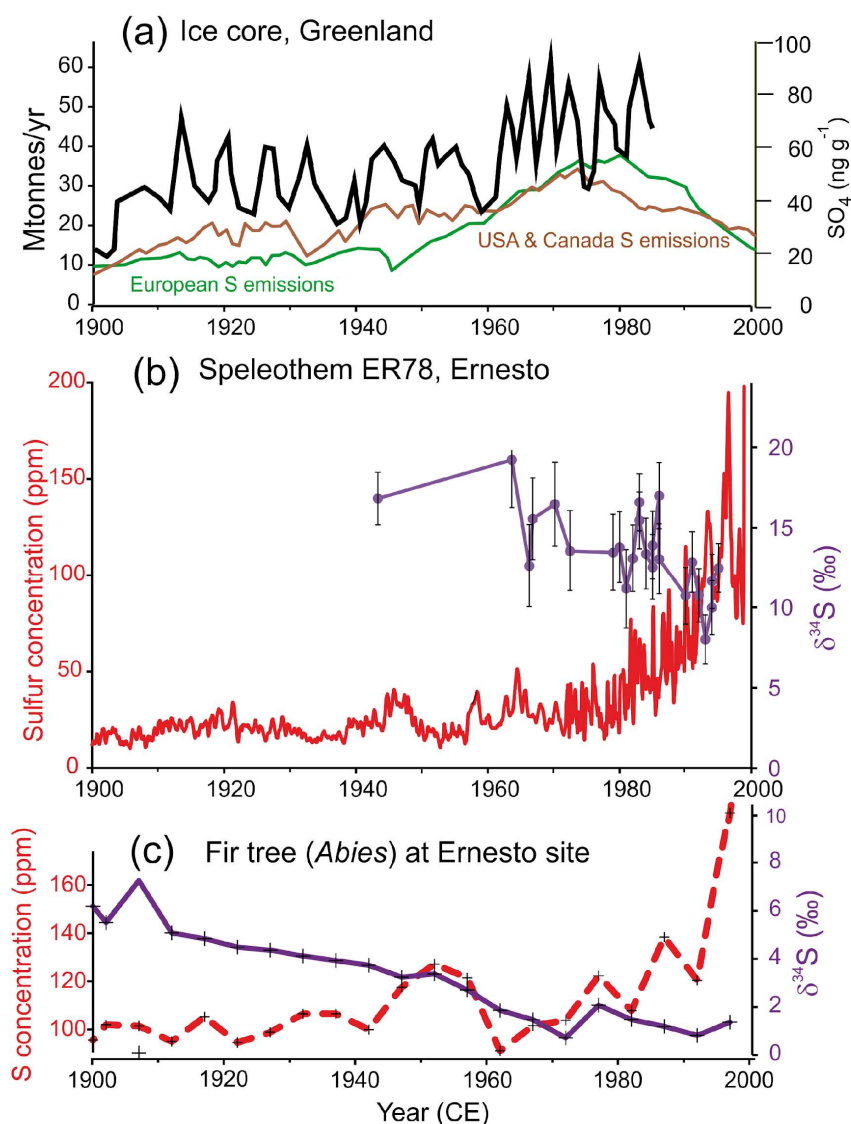
Figure 12. (a) Sulfate concentrations in Greenland ice core (Mayewski et al., 1990), and sulfur emissions from N. America and Europe (from Hoesly et al., 2018); (b) S concentration and \delta^{34}\text{S} from Ernesto cave, Italy (Frisia et al., 2005; Wynn et al., 2010; Borsato et al., 2023); and (c) S concentrations and \delta^{34}\text{S} in Abies alba from NE Italy (Wynn et al., 2014).
