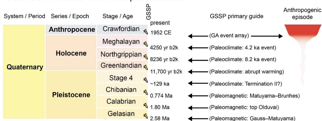
Figure 1. Chronostratigraphic subdivision of the Quaternary System/Period showing the position of the proposed Anthropocene Series/Epoch. Black type and yellow golden-spike symbols indicate ratified names and Global boundary Stratotype Sections and Points (GSSPs); grey type and grey golden spike symbols indicate names not yet approved (Stage 4 is a placeholder) and GSSPs in progress. Abbreviations yr b2k = years before 2000 CE; GA = Great Acceleration (modified from Head et al., 2022a).
