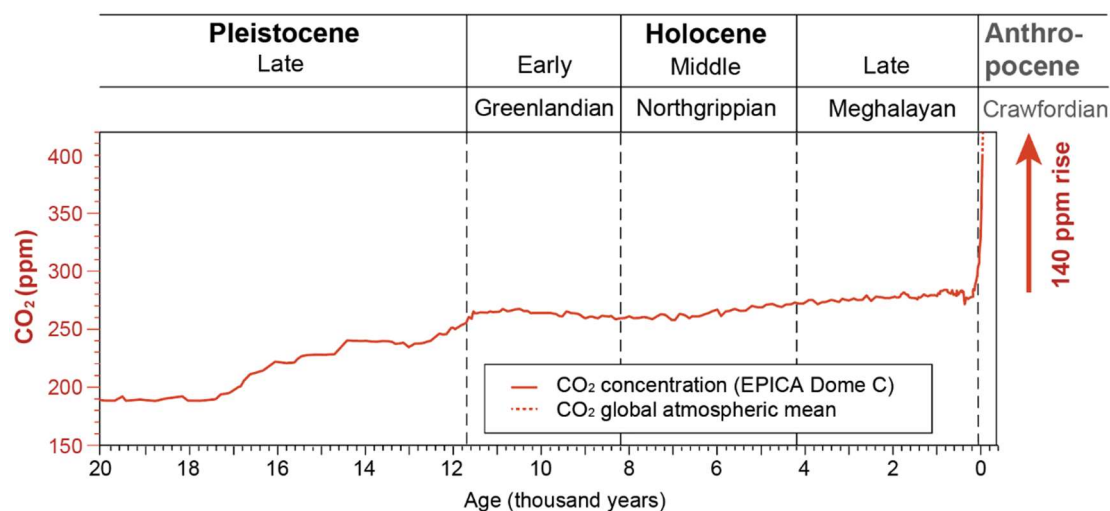
Figure 22. Atmospheric CO 2 records in Antarctic (EPICA Dome C) ice core over the last 20 kyr (Monnin et al. , 2001), supplemented by observational data from Rubino et al. (2013).
