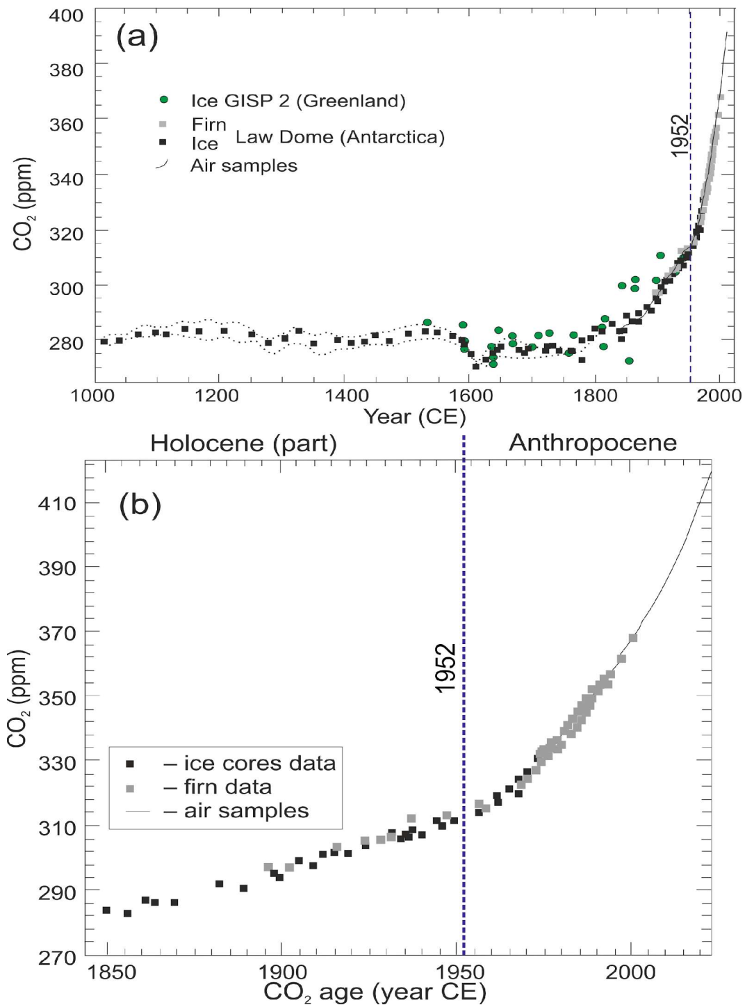
Figure 8. Atmospheric CO 2 records: (a) since 1000 CE from the Antarctic Law Dome ice core (Rubino et al., 2013) and Greenland GISP 2 ice core (Wahlen et al., 1991); reproduced from Zalasiewicz et al., 2020); (b) since 1850 CE from Antarctic Law Dome ice core, firn data and air samples (from Rubino et al., 2013, modified from Waters et al., 2016, and updated with data from Mauna Loa Observatory, Hawaii, from NOAA Climate.gov.).
