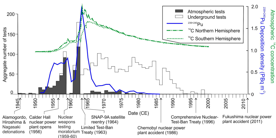
Figure 15. Timeline of key events that have influenced anthropogenic radiogenic signatures. The frequency of above-ground and underground nuclear weapons testing is compared with the fallout signals detected for plutonium and radiocarbon ( ^{14}\text{C} ). Note that fallout follows the aggregate number of tests, with a time lag of 6 months–2 years, with the ^{14}\text{C} peak lagging and at reduced levels in the Southern Hemisphere compared with the Northern Hemisphere. Data on aggregate test numbers sourced from UNSCEAR (2000), atmospheric ^{14}\text{C} concentrations from Hua et al. (2013) and for Pu from Hancock et al. (2014). From Cundy et al. (2022), modified from Waters et al. (2015).
