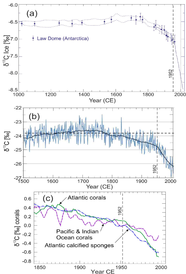
Figure 10. (a) \delta^{13}\text{C} variability in the Antarctic Law Dome ice core (Rubino et al. , 2013); (b) \delta^{13}\text{C} variability for a composite tree ring chronology developed using Pinus sylvestris trees from northern Fennoscandia (Loader et al. , 2013). Fine blue line represents annually-resolved \delta^{13}\text{C} variability, solid black line presents the annual data smoothed with a centrally-weighted 51-year moving average. Dashed line represents the mean \delta^{13}\text{C} value for the “pre-industrial” period 1500–1799 CE; and (c) changes in \delta^{13}\text{C} from Atlantic and Pacific/Indian ocean corals and Atlantic calcified sponges, shown as a five-year running mean (Swart et al. , 2010). Reproduced from Zalasiewicz et al. (2020).
