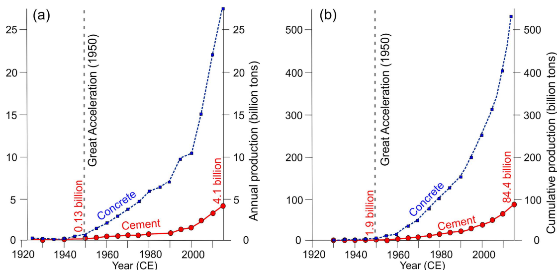
Figure 7. (a) annual global production and (b) cumulative production of cement and estimated concrete production (from Waters & Zalasiewicz, 2018).
