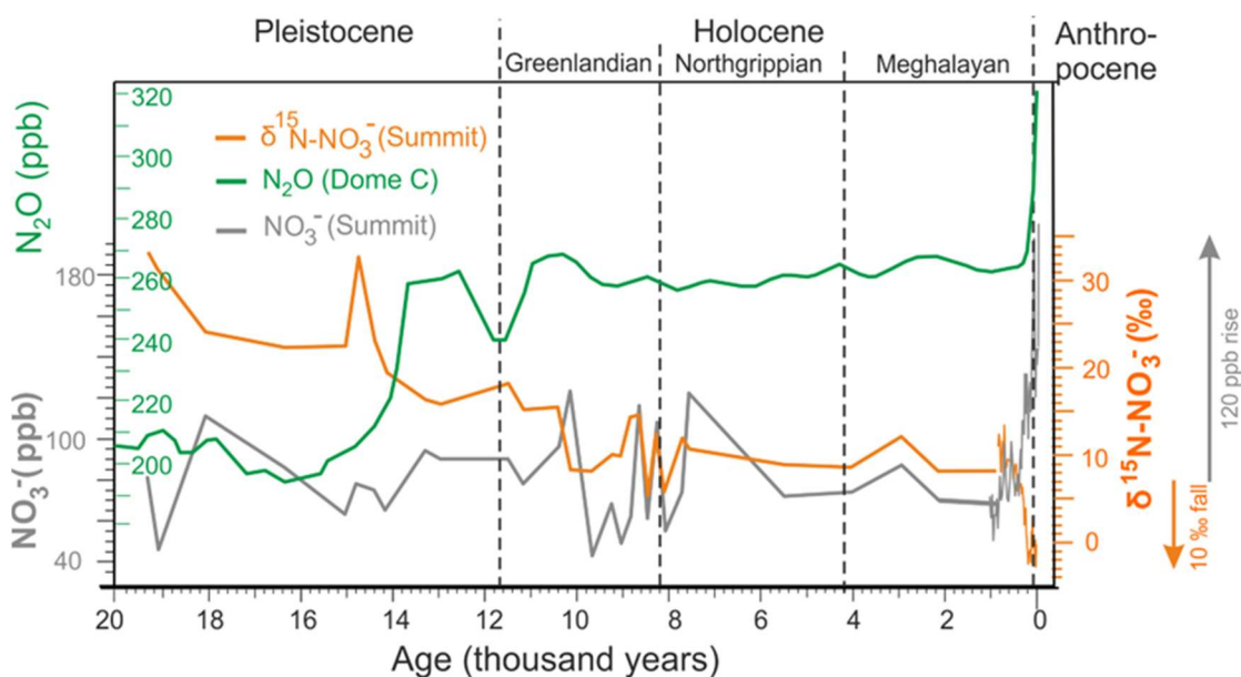
Figure 25. Ice core \text{NO}_3^- and \delta^{15}\text{N} from Summit, Greenland (from Hastings et al. , 2005, 2009 and Wolff, 2014, reproduced in Waters et al. , 2016); \text{N}_2\text{O} curve from Antarctic Dome C ice core (Flückiger et al. , 2002; Schilt et al. 2010b).
