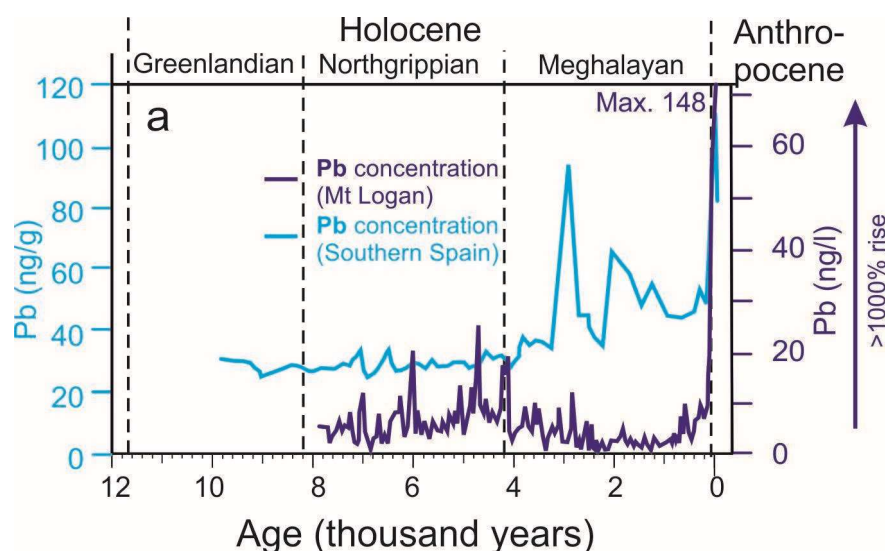
Figure 26. Variations in Pb concentrations in ice core from Mt. Logan, Yukon (Osterberg et al. , 2008) and Laguna de Rio Seco, southern Spain (García-Alix et al. , 2013).
