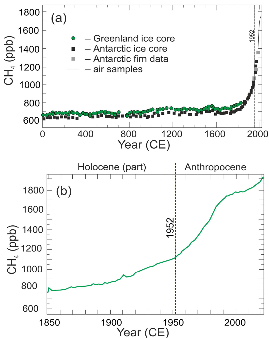
Figure 9. Atmospheric CH 4 records: (a) in ice core from Greenland GISP 2 (Mitchell et al. , 2003) and Antarctic Law Dome ice core, firn data and air samples (Ferretti et al. , 2005); reproduced from Zalasiewicz et al. (2020); (b) since 1850 CE in Antarctic Law Dome ice core, firn data and air samples (Ferretti et al. , 2005, updated with data from Mauna Loa Observatory Hawaii from NOAA Climate.gov.).
