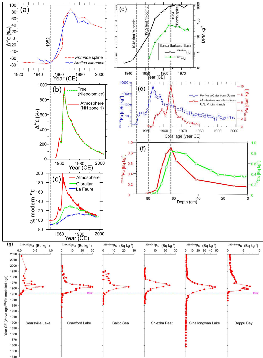
Figure 16. Examples of ^{14}\text{C} , Pu and ^{137}\text{Cs} signals within different environments. (a) Spline for seven different colonies of the deep-sea gorgonian coral Primnoa resedaeformis and the bivalve mollusc Arctica islandica (Sherwood et al., 2005); (b) \Delta^{14}\text{C} in tree rings ( Pinus sylvestris ) at Niepolomice (Poland) compared with Northern Hemisphere atmospheric values (Rakowski et al., 2013); (c) comparison of Northern Hemisphere atmospheric \delta^{14}\text{C} values with speleothems from La Faurie Cave, southwest France and Lower Saint Michael's Cave, Gibraltar (Fairchild & Frisia, 2014); (d) ^{239+240}\text{Pu} and ^{238}\text{Pu} signals in the Santa Barbara Basin, USA (Koide et al., 1975), note
