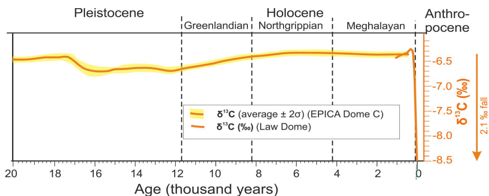
Figure 24 \delta^{13}\text{C} variability over 20 kyr in the Antarctic EPICA Dome C (Schmitt et al. , 2012) and Law Dome ice cores (Rubino et al. , 2013).
