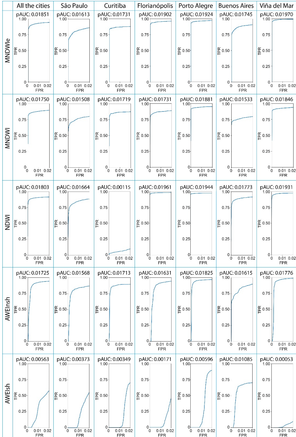
Figure 2 – Partial ROC curve up to 0.02 FPR indicating the cities with the best performances by index.
