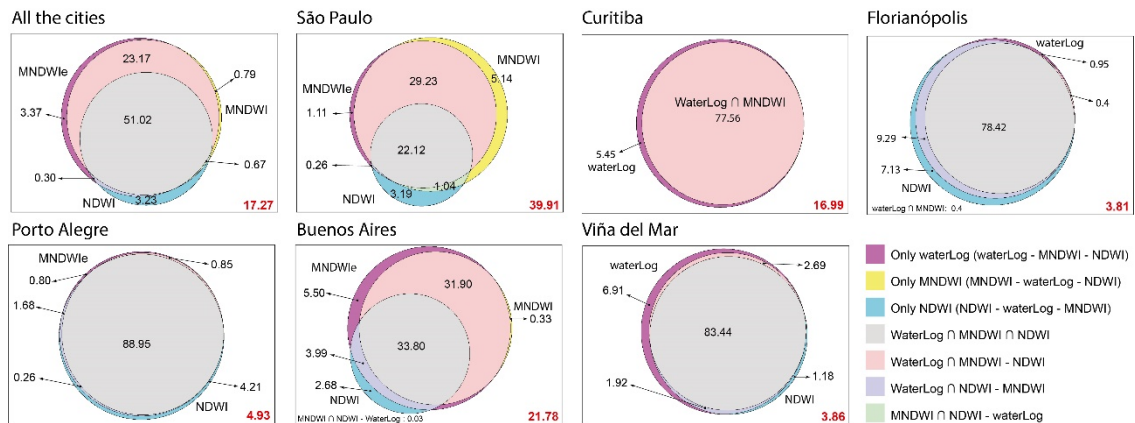
Figure 4 – Venn Diagram with the percentage of sample points classified as water for the MNDWle, MNDWI, and NDWI indices. The values highlighted in red in the graphs represent sample points incorrectly classified as water (False Negative Rate - FNR). The union of all sets equals 100 - FNR. Thus: All Cities = 82.06%; São Paulo = 59.44%; Curitiba = 79.06%; Florianópolis = 96.02%; Porto Alegre = 94.46%; Buenos Aires = 78.47%; Viña Del Mar = 96.27%.
