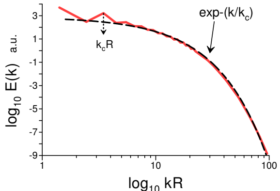
Figure 1: Magnetic energy spectrum E(k) generated by a chaotic magnetohydrodynamic dynamo in a conducting spherical Couette flow at Pr_m = 0.25 (a direct numerical simulation).
