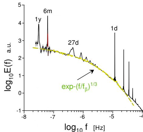
Figure 7: Frequency magnetic energy spectrum obtained using measurements provided by the global magnetic observatory network.
