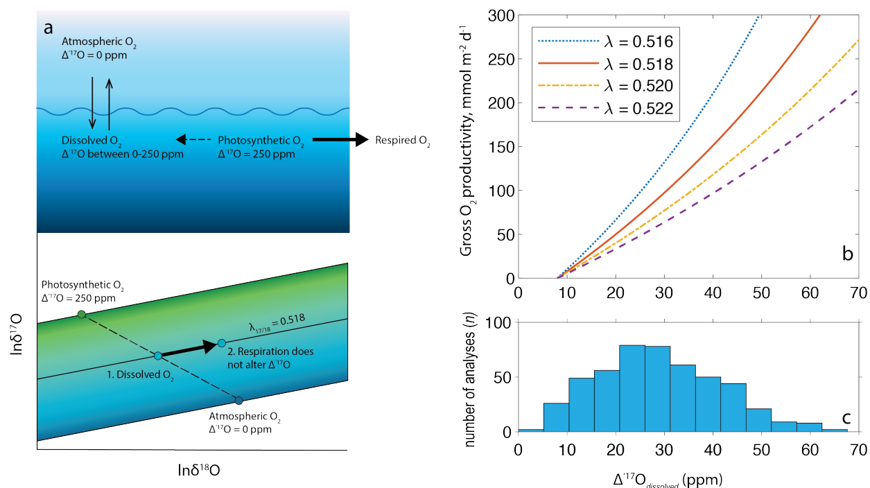
Figure 1: (a) Schematic (after Juranek and Quay) 21 showing how dissolved O 2 \Delta^{17}\text{O} can be a mixture (dashed line) of endmember atmospheric and photosynthetic O 2 compositions, and respiration fractionation that assumes \lambda_{17/18} will preserve \Delta^{17}\text{O} . (b) Calculated GOP plotted against \Delta^{17}\text{O} value for different \lambda values using the method of Prokopenko et al. 22 and photosynthetic O 2 from average marine phytoplankton according to Luz and Barkan 61 assuming \delta^{18}\text{O}_{\text{O}_2} = 0.73\text{‰} , k = 3 \text{ m d}^{-1} , and [\text{O}_2]_{\text{eq}} = 230 \text{ mol m}^{-3} . (c) Histogram of Southern Ocean \Delta^{17}\text{O} data from Reuer et al as an example of the range of measured \Delta^{17}\text{O} values in an field studies. 49
