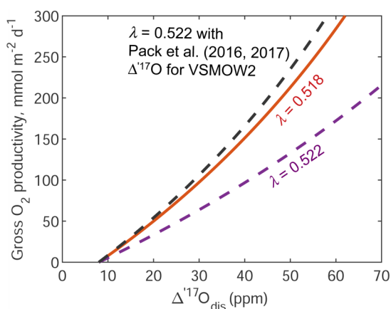
Figure 9. Calculated GOP using the parameters shown in Fig. 1B-C, with effect of VSMOW2 composition overlaid. Using the \Delta^{17}\text{O} value of VSMOW2 from Pack et al. (2016, 2017) instead of Barkan and Luz (2011) and \lambda = 0.522 —approximating a closed system in which ^{18}\epsilon_{resp} \sim -18\text{‰} and \theta_{17/18,resp} = 0.520 —results in much smaller changes to GOP ( \lambda = 0.518 ) compared to a \lambda = 0.522 revision alone. 30, 31, 122
