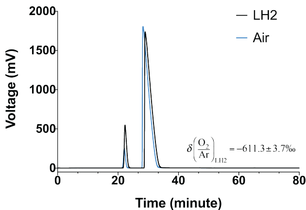
Figure 2: Typical chromatogram obtained from the thermal conductivity detector (25 mL min -1 , 1/8" x 3.05 m Molecular Sieve 5A column, 80/100 mesh) showing the baseline separation of O 2 and Ar (an important mass 36 interference) achieved during purification for both a standard air (blue line) and LH2 incubation (black line).
