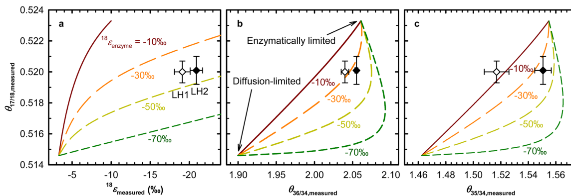
Figure 8. Results of two-step diffusion-enzymatic reduction model for isotopologue fractionation. Cross-plots are shown of the predicted covariations of \theta_{17/18,\text{measured}} with (a) ^{18}\epsilon_{\text{measured}} , (b) \theta_{36/34,\text{measured}} , and (c) \theta_{35/34,\text{measured}} , together with experimental results.
