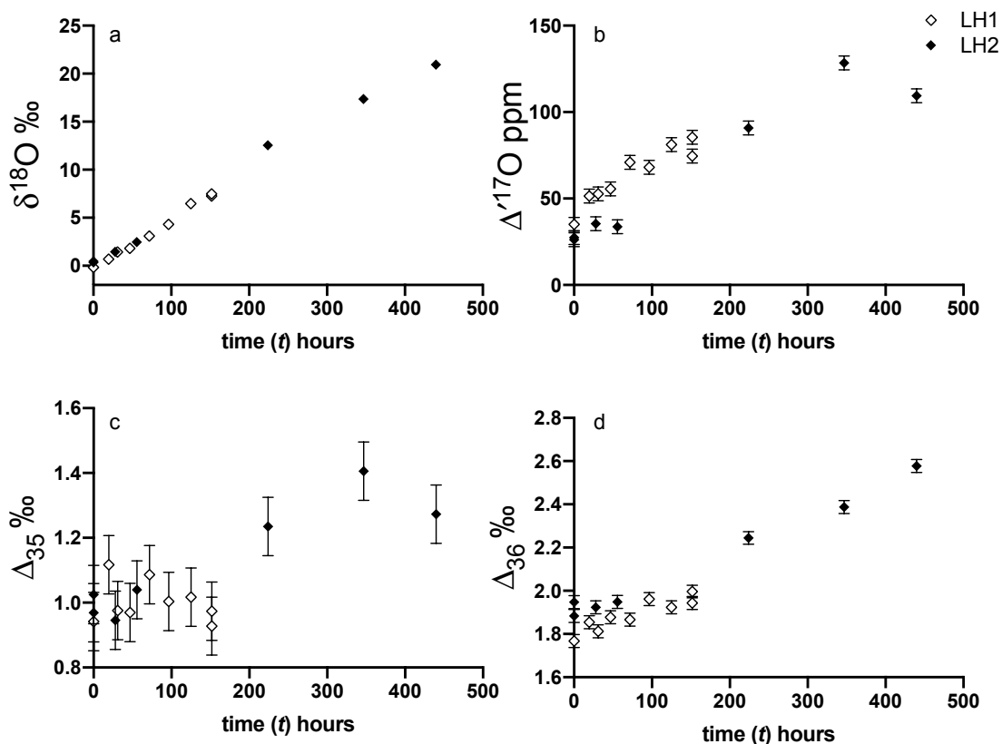
Figure 5. Variations in (a) \delta^{18}\text{O} , (b) \Delta^{17}\text{O} , (c) \Delta_{35} and (d) \Delta_{36} for LH1 (white diamonds) and LH2 (black diamonds) as a function of time. Error bars are 1 \sigma from replicate measurements of air dissolved in water and are smaller than symbols for \delta^{18}\text{O} .
