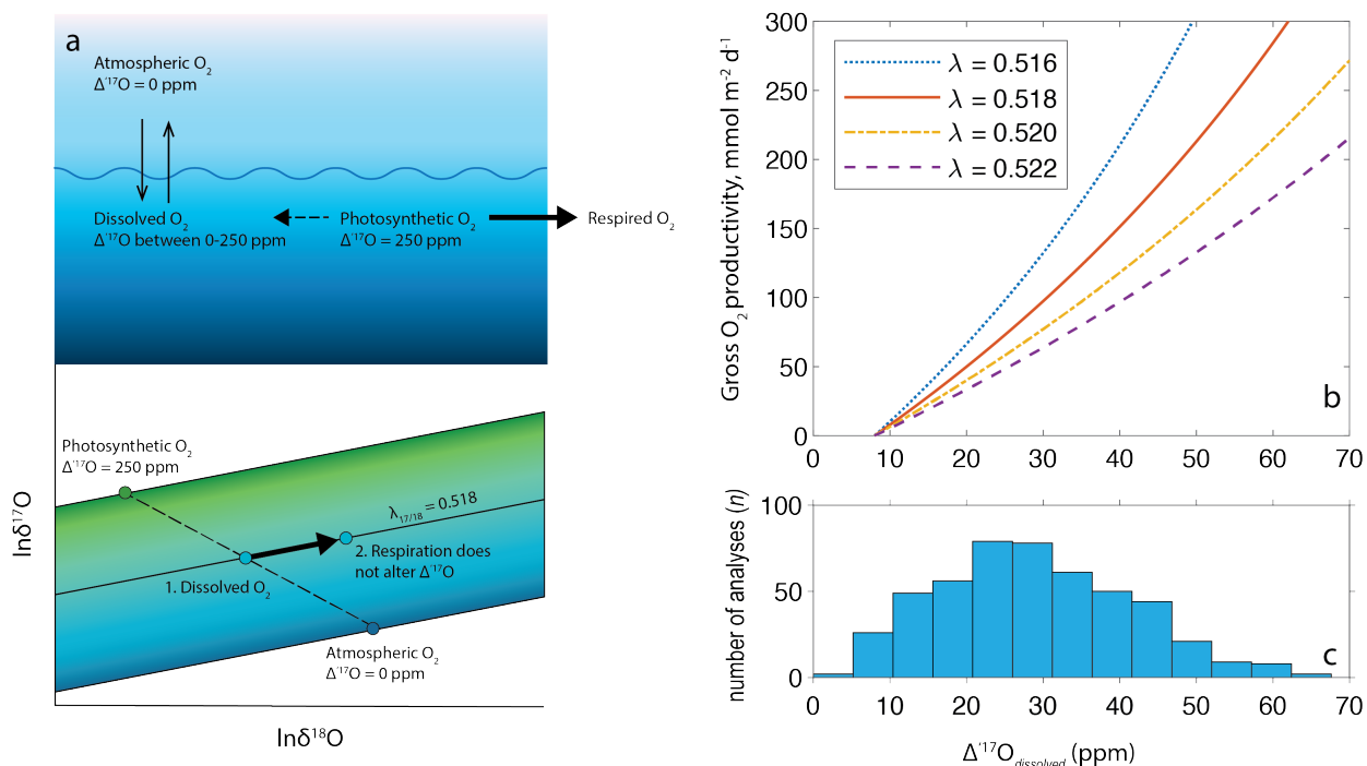
Figure 1: (a) Schematic (after Juranek and Quay) 21 showing how dissolved O 2 Δ 17 O can be a mixture (dashed line) of endmember atmospheric and photosynthetic O 2 compositions, and respiration fractionation that assumes \lambda_{17/18} will preserve Δ 17 O. (b) Calculated GOP plotted against Δ 17 O value for different λ values using the method of Prokopenko et al. 22 and photosynthetic O 2 from average marine phytoplankton according to Luz and Barkan 61 assuming \delta^{18}\text{O}_{\text{O}_2} = 0.73\text{‰} , k = 3 \text{ m d}^{-1} , and [\text{O}_2]_{\text{eq}} = 230 \text{ mol m}^{-3} . (c) Histogram of Southern Ocean Δ 17 O data from Reuer et al as an example of the range of measured Δ 17 O values in an field studies. 49
