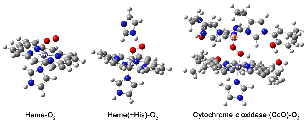
Figure 3. Oxyheme models used in this study. White atoms are hydrogen, grey atoms are carbon, blue atoms are nitrogen, and red atoms are oxygen. Transition-metal atoms (Fe, in lavender, and Cu, in orange) are labeled.
