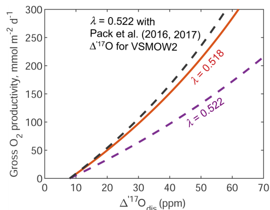
Figure 9. Calculated GOP using the parameters shown in Fig. 1B-C, with effect of VSMOW2 composition overlaid. Using the Δ 17 O value of VSMOW2 from Pack et al. (2016, 2017) instead of Barkan and Luz (2011) and λ = 0.522—approximating a closed system in which 18 ε resp ~ -18‰ and θ 17/18,resp = 0.520—results in much smaller changes to GOP (λ = 0.518) compared to a λ = 0.522 revision alone. 30, 31, 121
