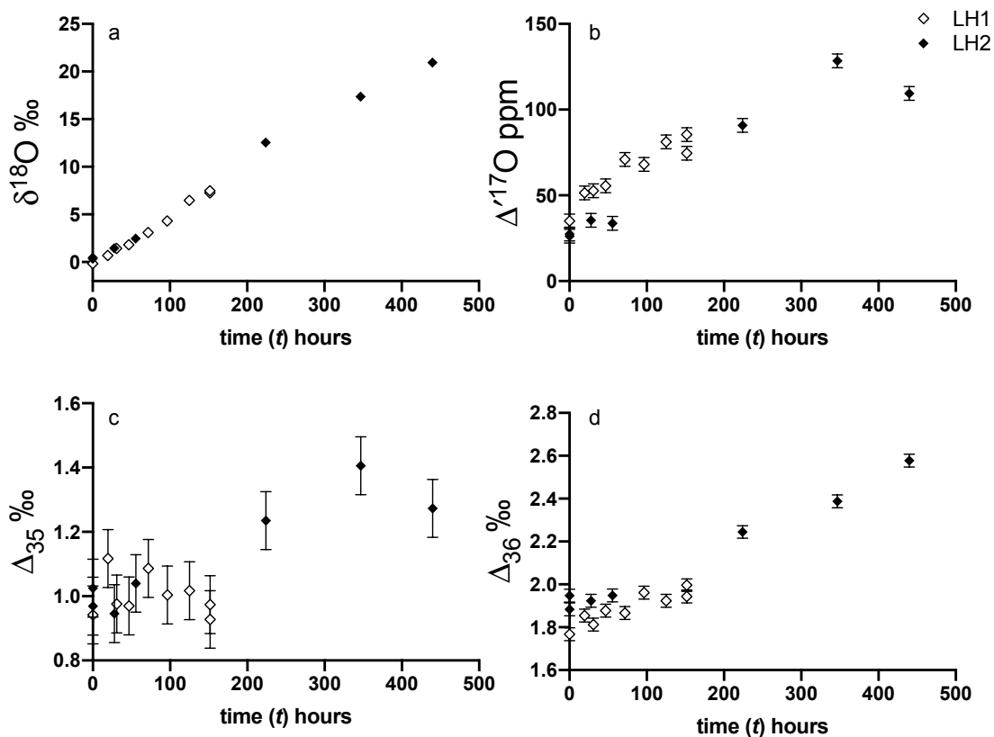
Figure 5. Variations in \delta^{18}\text{O} , \Delta^{17}\text{O} , \Delta_{35} and \Delta_{36} for LH1 (white diamonds) and LH2 (black diamonds) as a function of time. Error bars are 1\sigma from replicate measurements of air dissolved in water and are smaller than symbols for \delta^{18}\text{O} .
